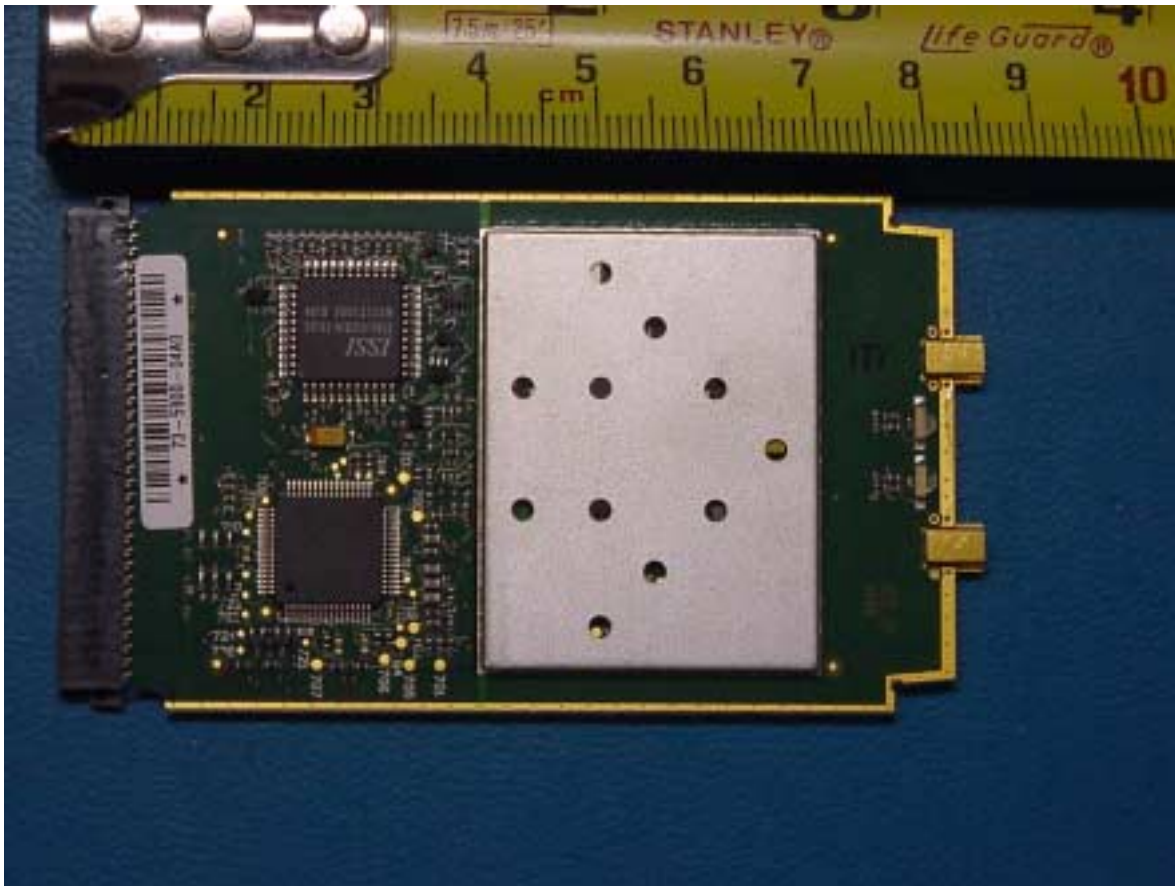
Front of pcb with shields
