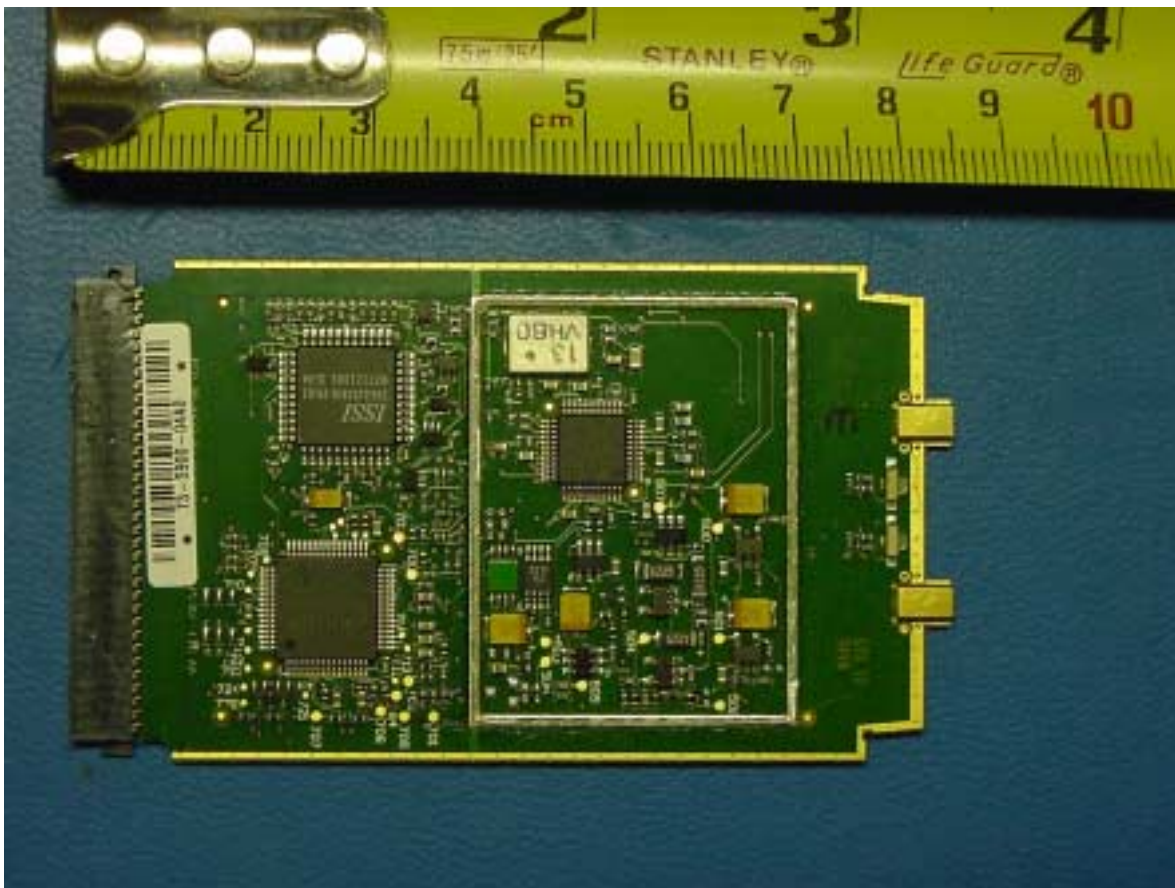
Front of pcb without shields
