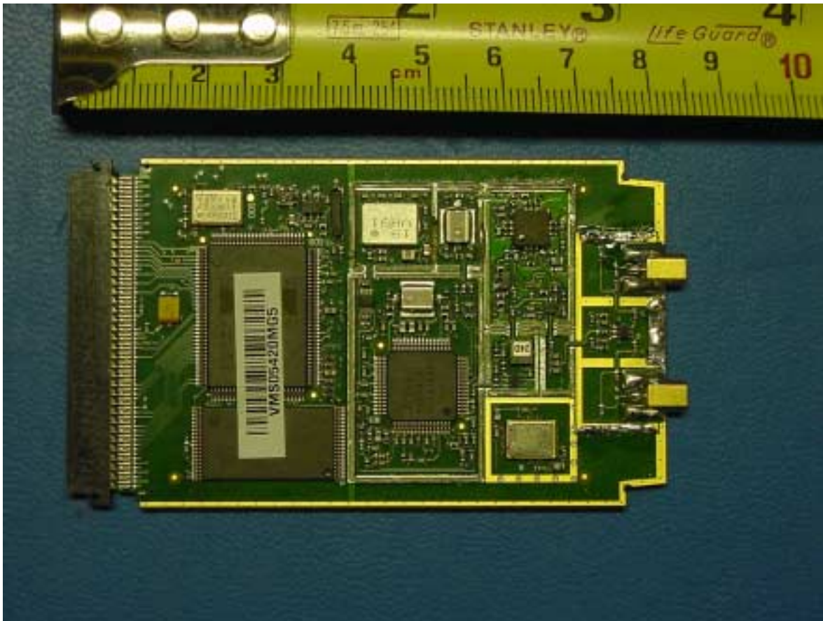
Rear of pcb without shields
