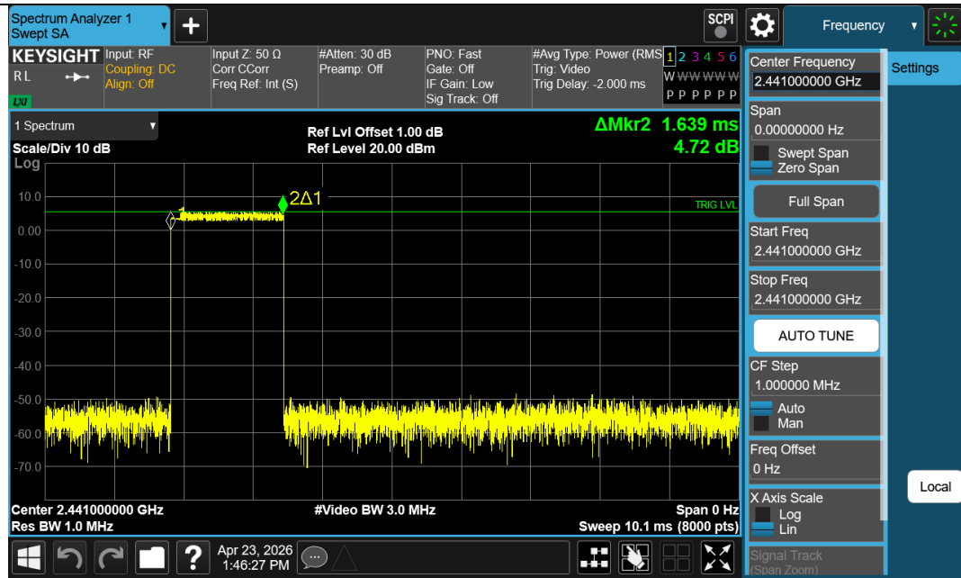
2DH3-Ant1-Hop-PASS
