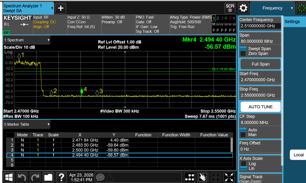
3DH5-Ant1-Hop_2480-PASS
