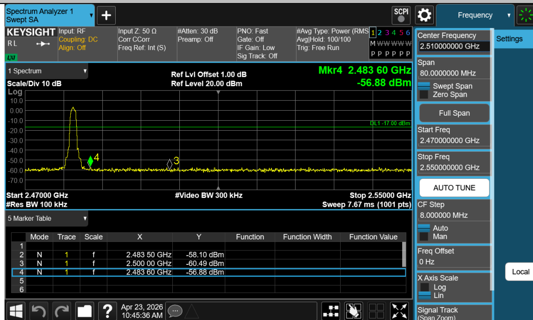
2DH5-Ant1-2480-PASS
