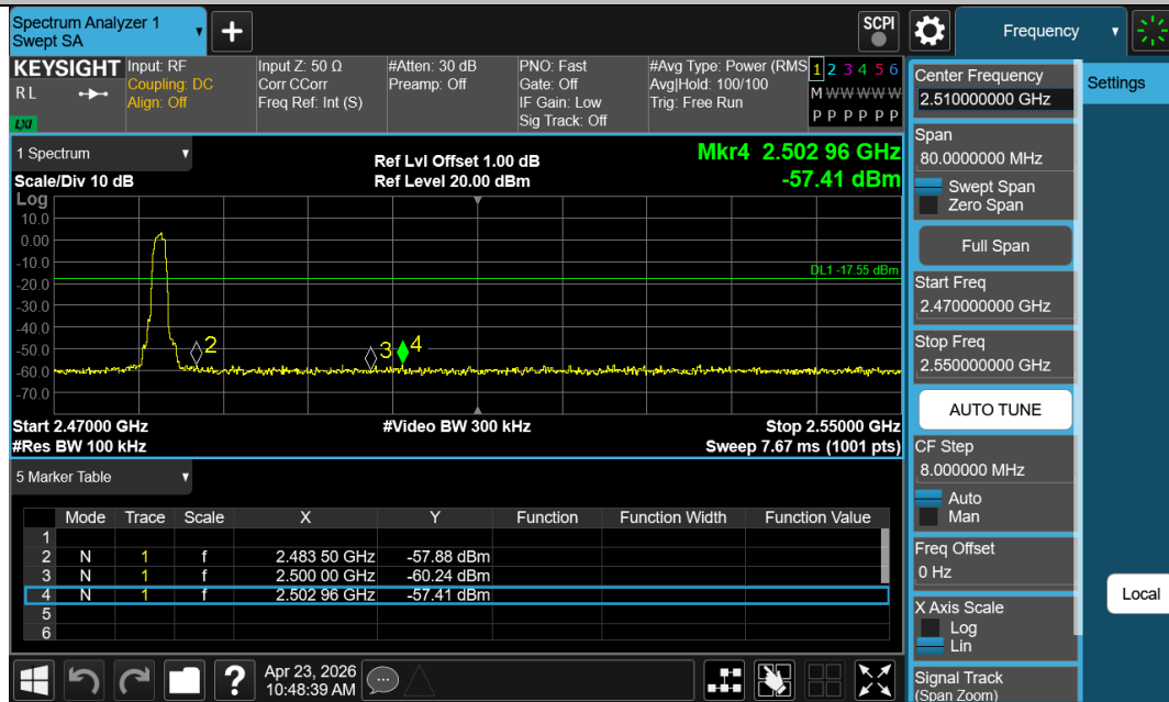
3DH5-Ant1-2480-PASS
