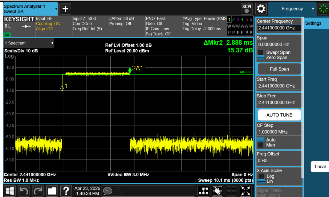
2DH5-Ant1-Hop-PASS
