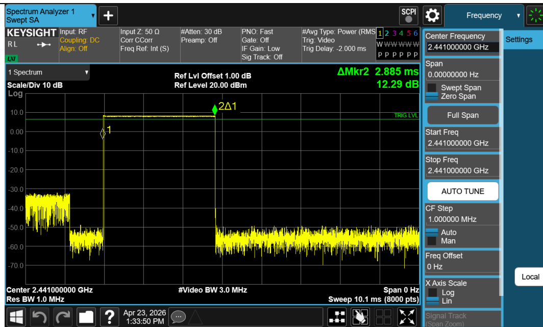
DH5-Ant1-Hop-PASS
