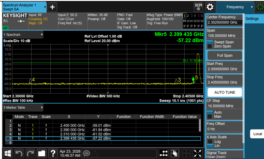
3DH5-Ant1-2402-PASS
