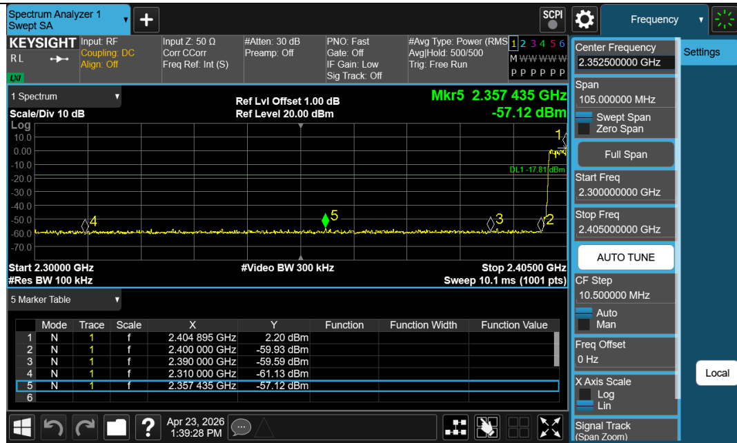
2DH5-Ant1-Hop_2402-PASS
