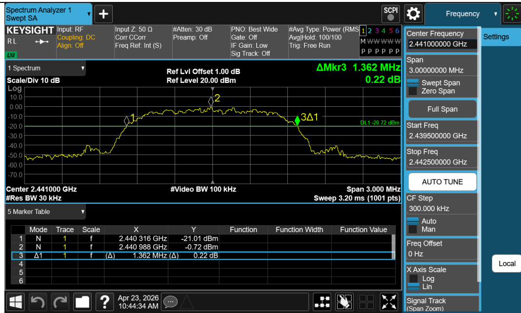
2DH5-Ant1-2441
