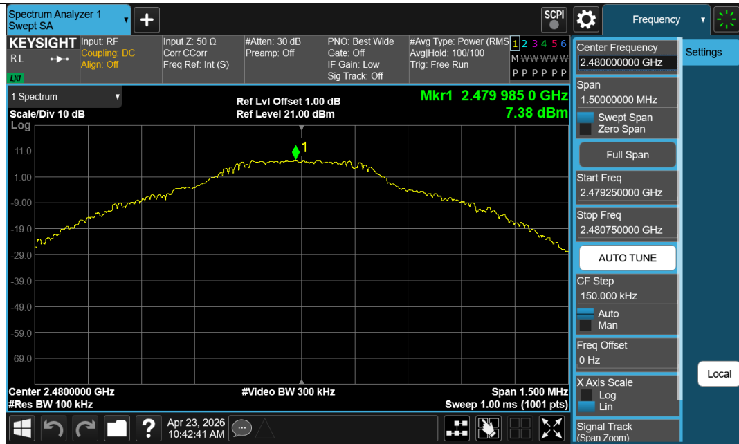
DH5-Ant1-2480-PASS
