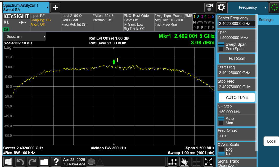
2DH5-Ant1-2402-PASS
