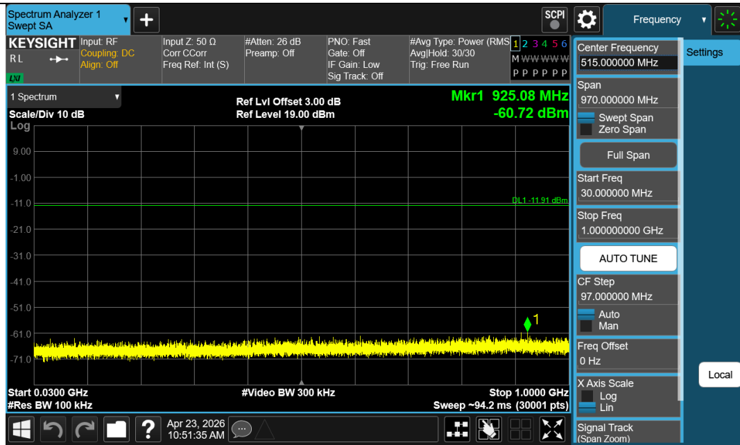
DH5-Ant1-2441-30~1000-PASS
