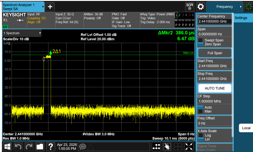
3DH1-Ant1-Hop-PASS
