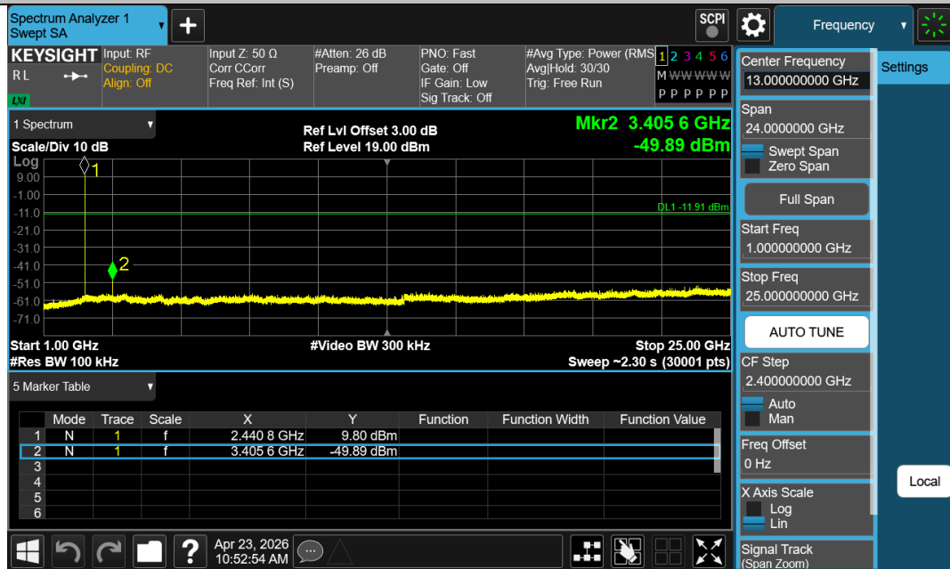
DH5-Ant1-2441-1000~25000-PASS
