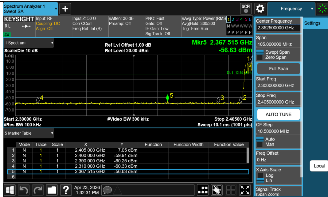
DH5-Ant1-Hop_2402-PASS
