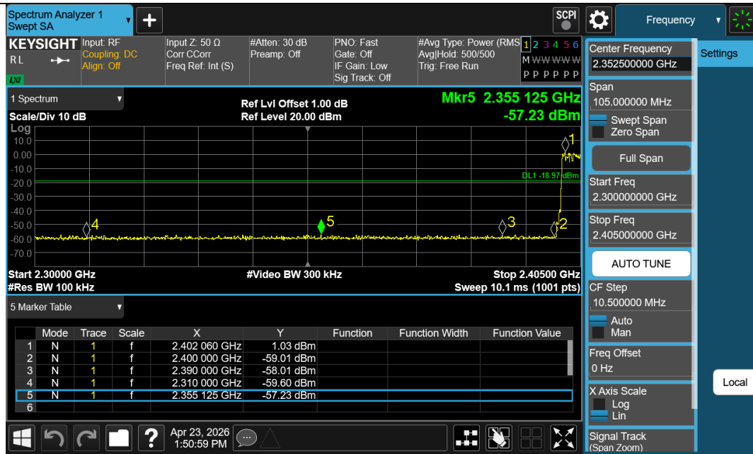
3DH5-Ant1-Hop_2402-PASS
