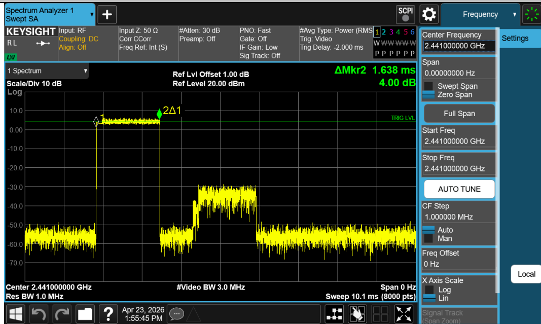
3DH3-Ant1-Hop-PASS
