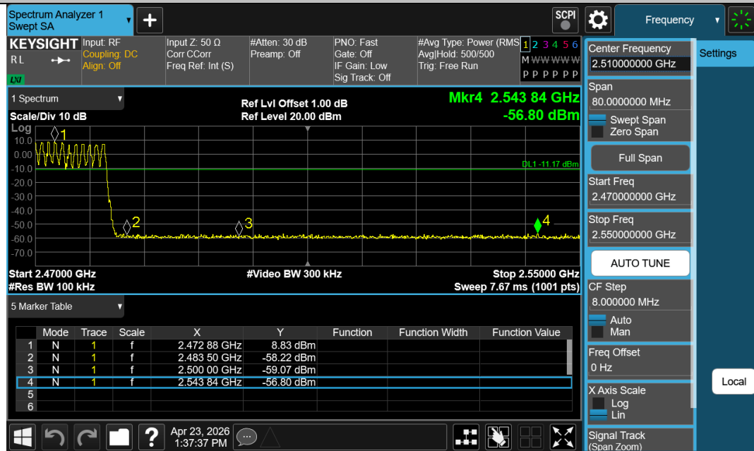
DH5-Ant1-Hop_2480-PASS
