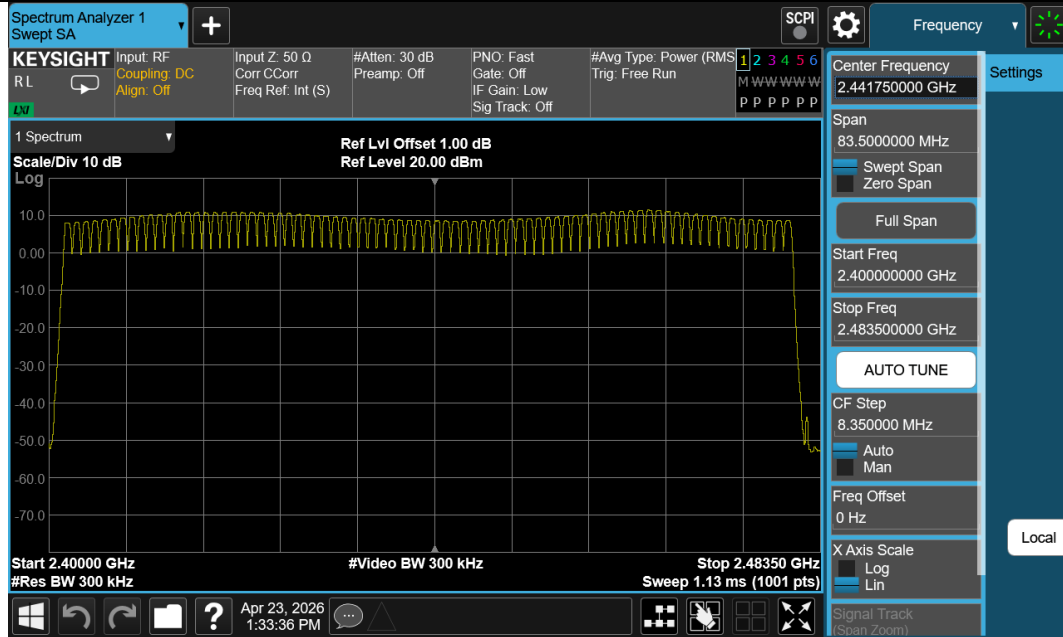
DH5-Ant1-Hop-PASS
