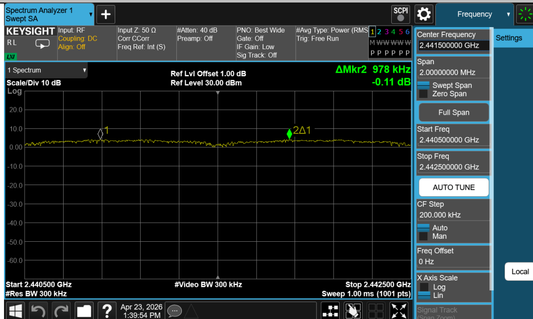
2DH5-Ant1-Hop-PASS
