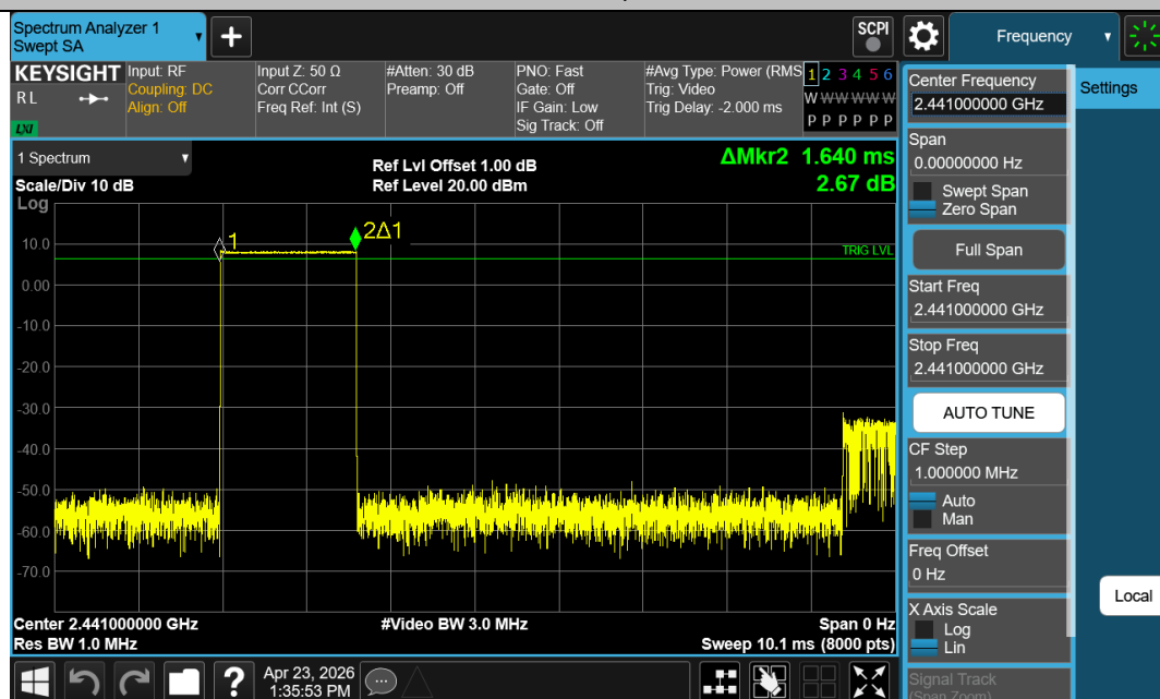
DH3-Ant1-Hop-PASS
