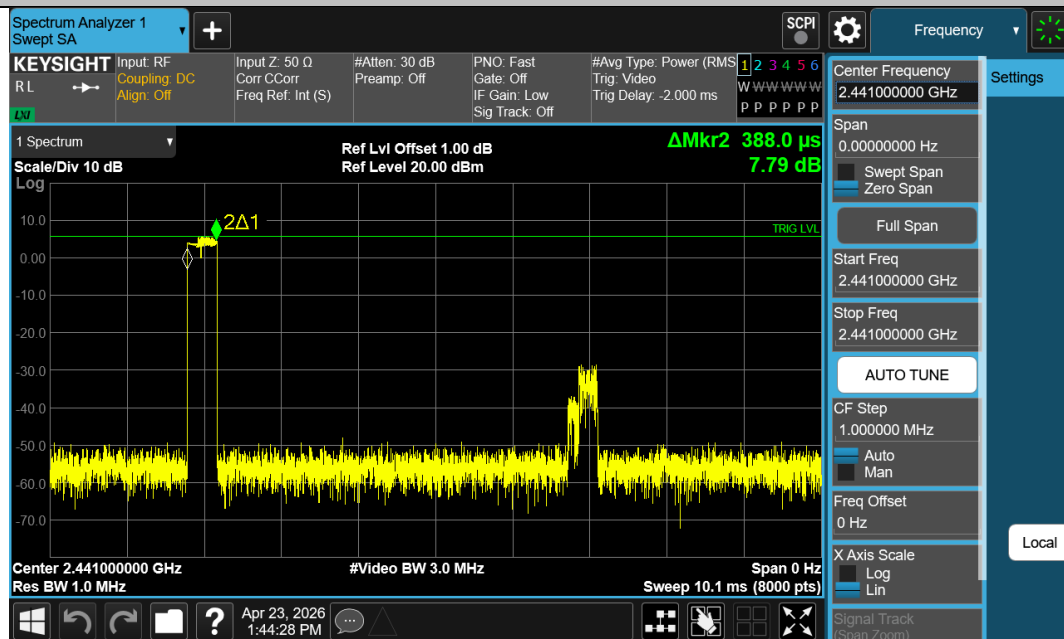
2DH1-Ant1-Hop-PASS
