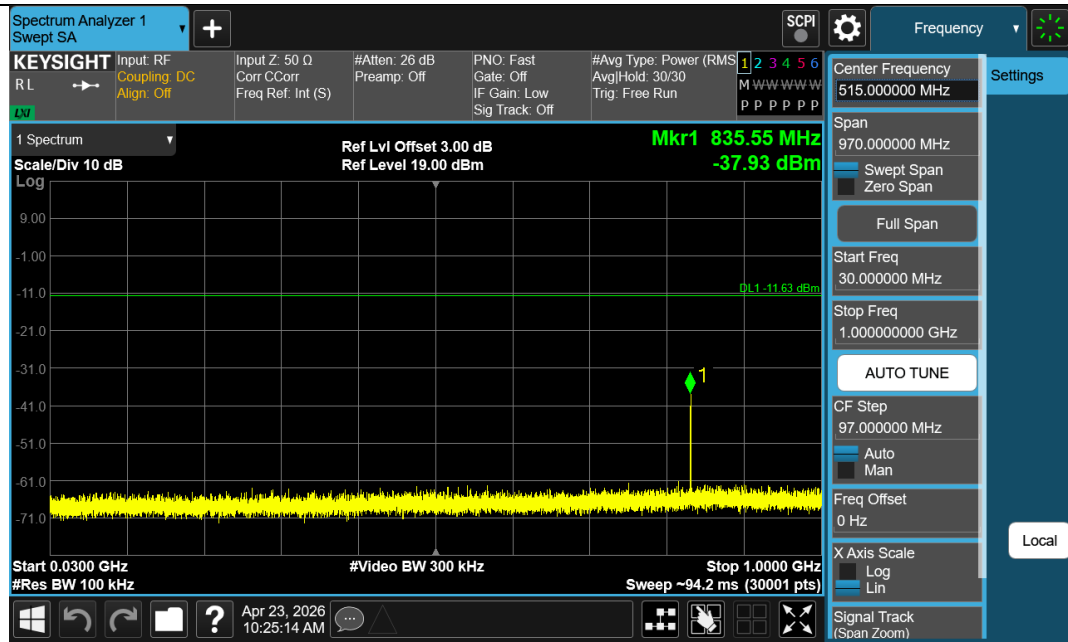
BLE_1M-Ant1-2480-30~1000-PASS
