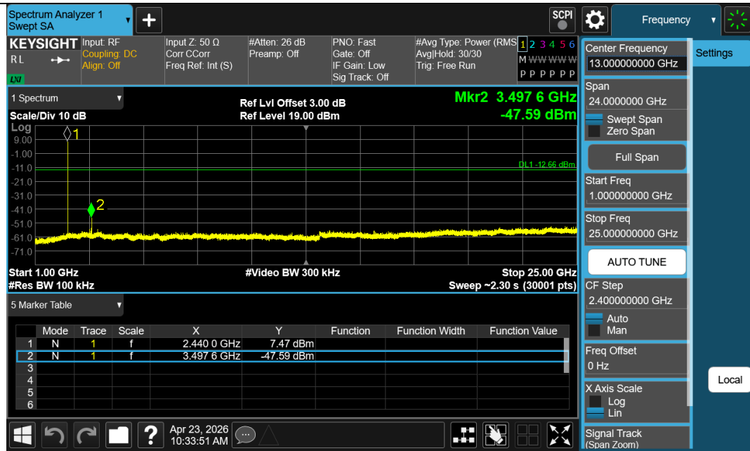
BLE_2M-Ant1-2440-1000~25000-PASS
