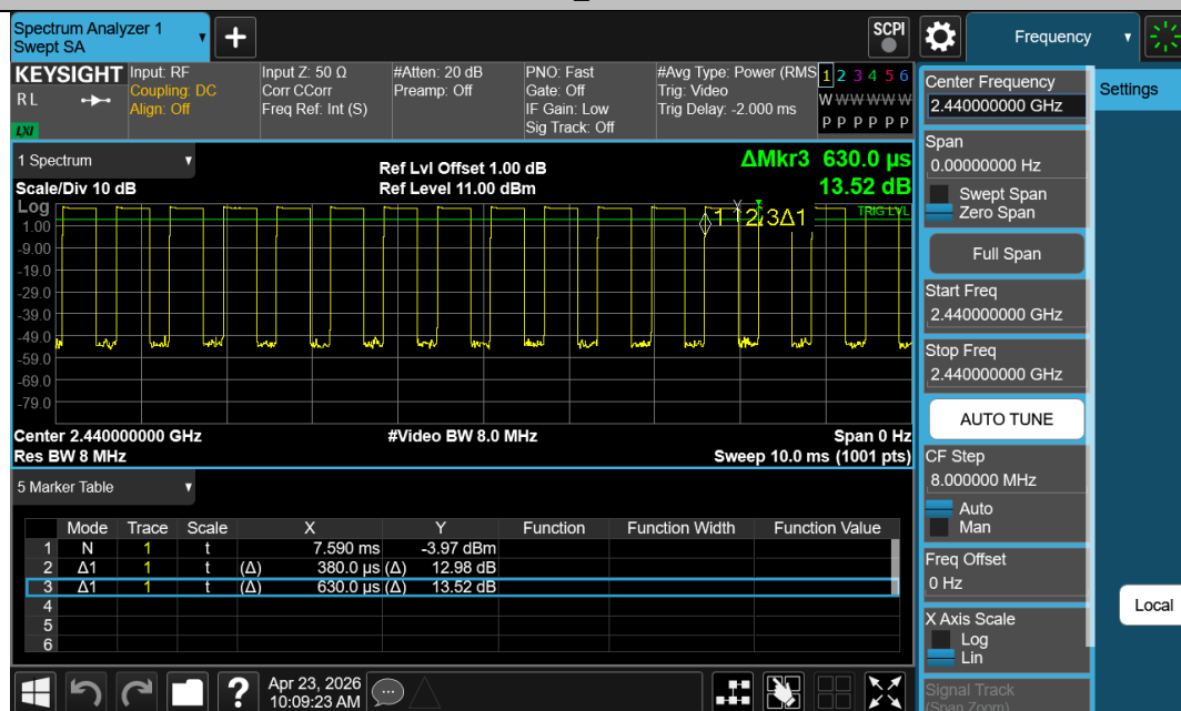
NTNV-BLE_1M-Ant1-2440
