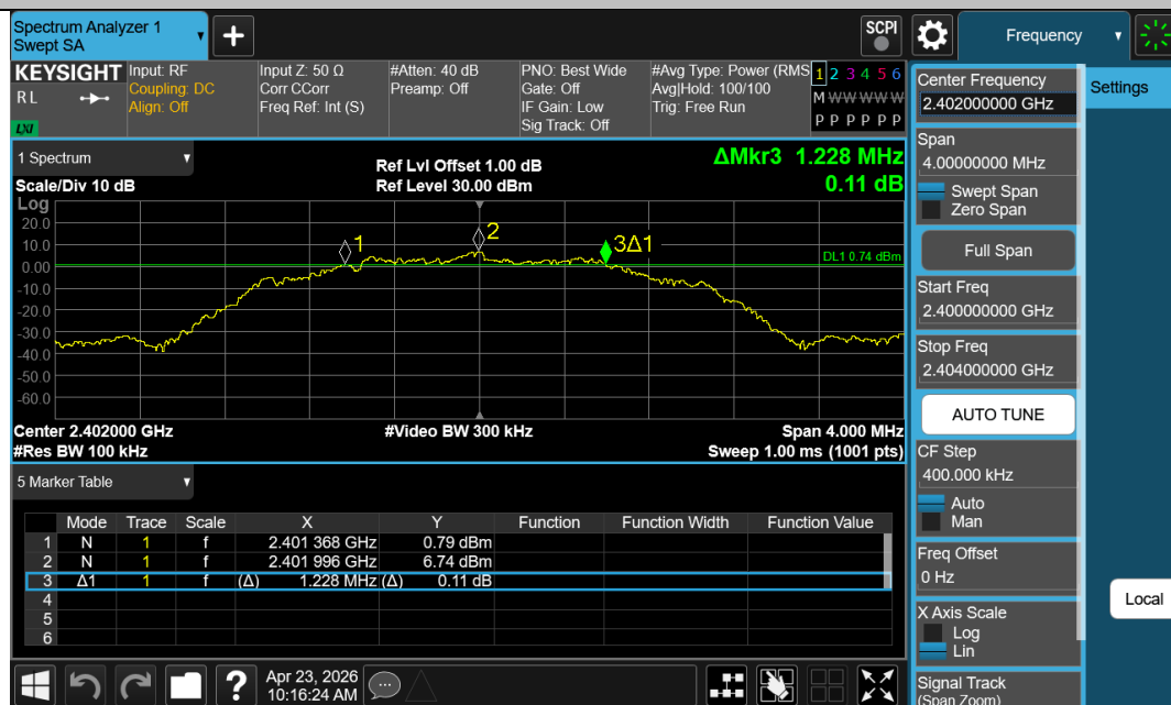
BLE_2M-Ant1-2402-PASS
