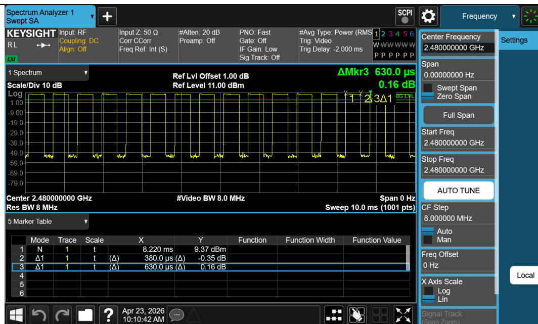
NTNV-BLE_1M-Ant1-2480
