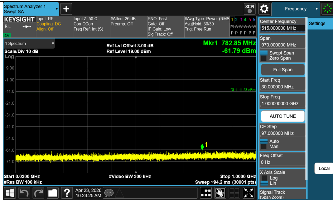
BLE_1M-Ant1-2440-30~1000-PASS
