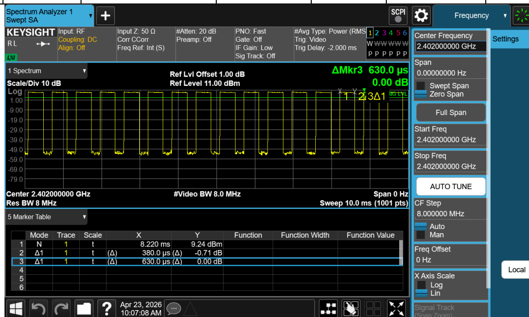
NTNV-BLE_1M-Ant1-2402
