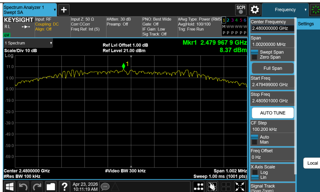
BLE_1M-Ant1-2480-PASS
