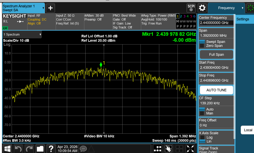
BLE_1M-Ant1-2440-PASS
