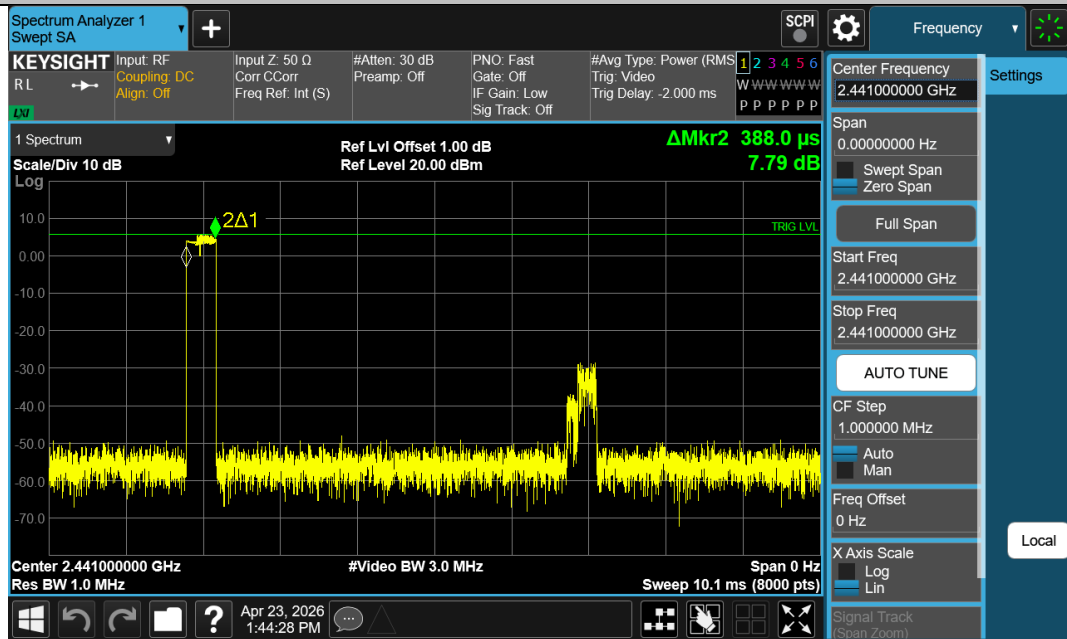
2DH1-Ant1-Hop-PASS
