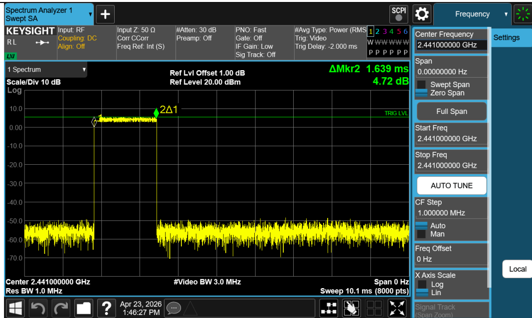
2DH3-Ant1-Hop-PASS
