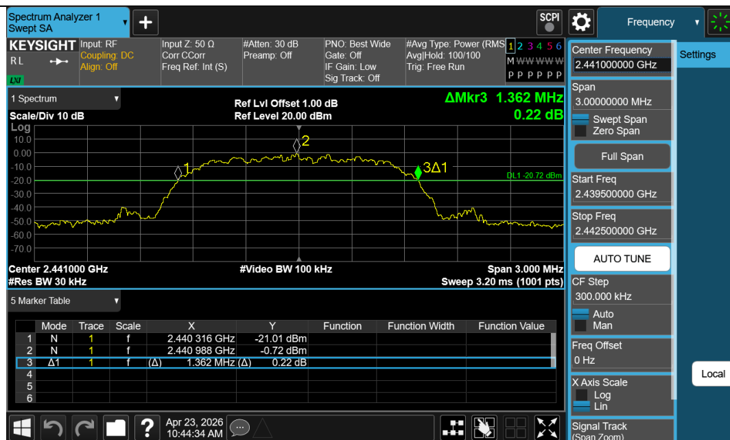
2DH5-Ant1-2441
