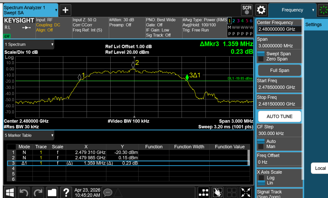
2DH5-Ant1-2480
