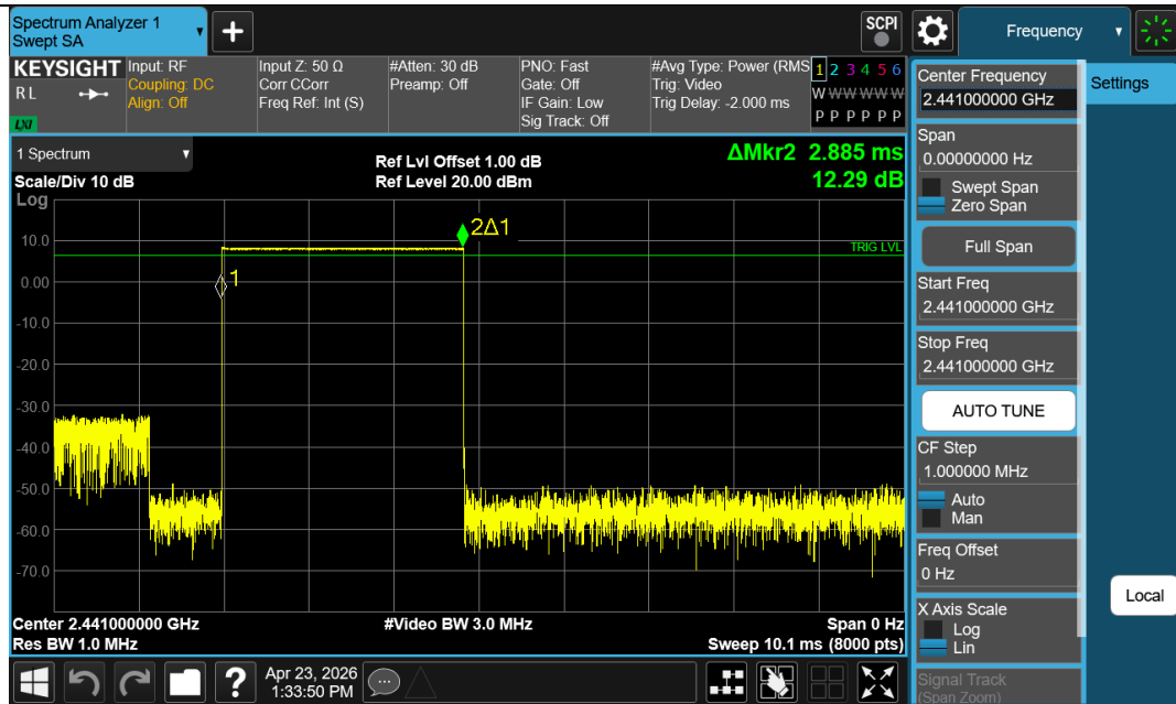
DH5-Ant1-Hop-PASS
