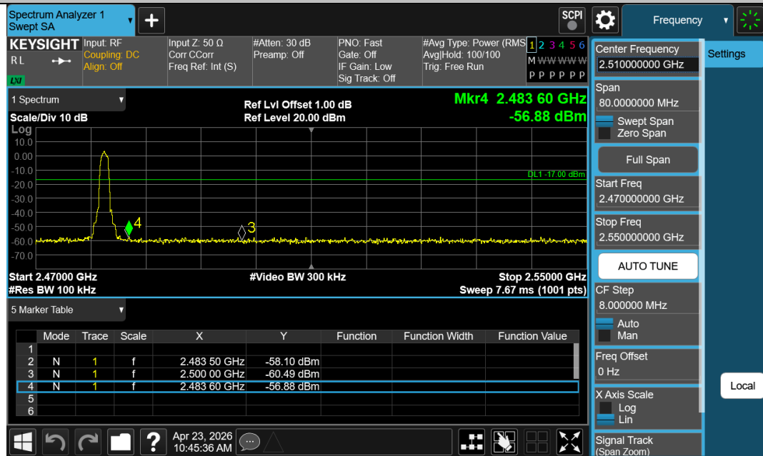
2DH5-Ant1-2480-PASS
