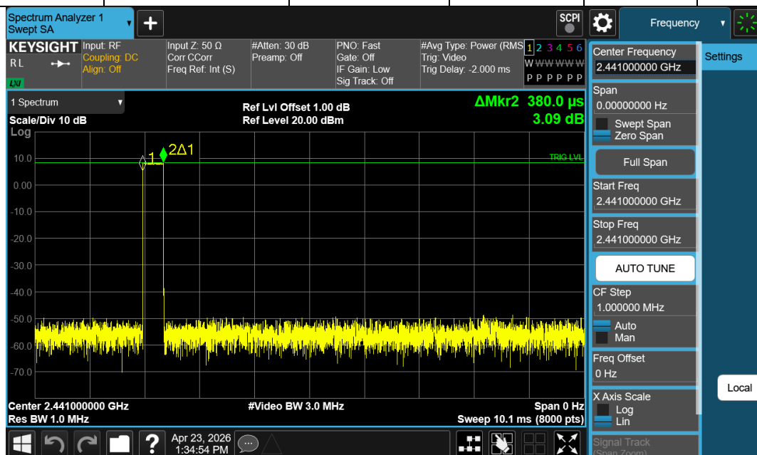
DH1-Ant1-Hop-PASS
