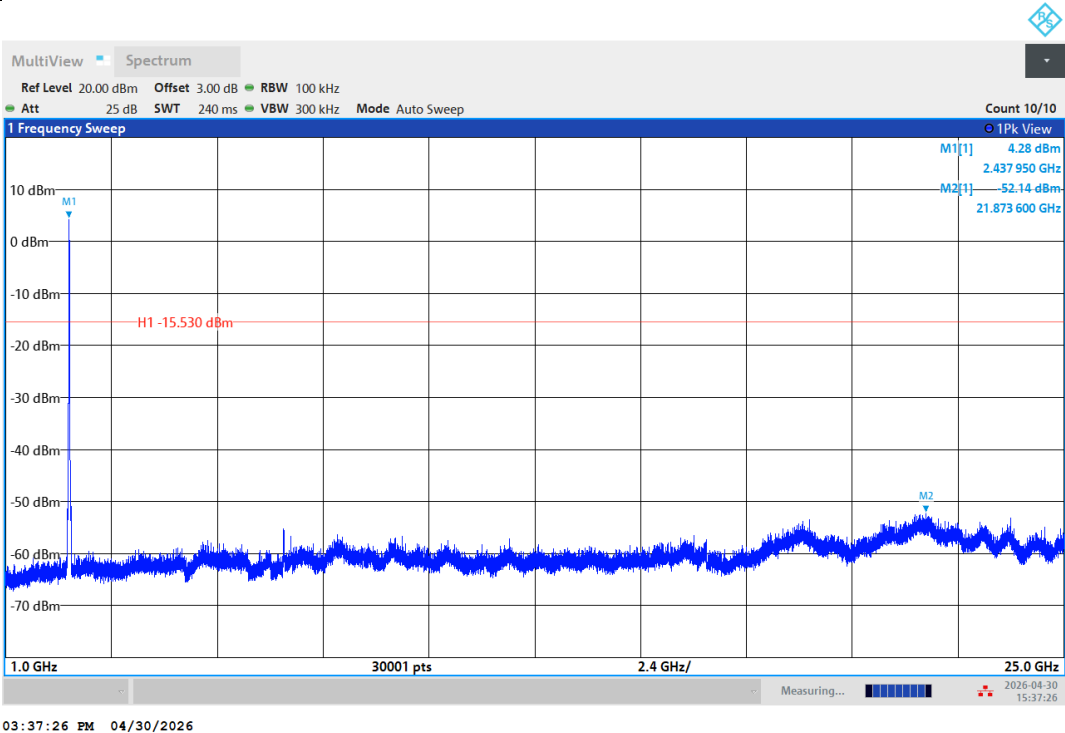
11AC20SISO-Ant1-2437-1000~25000-PASS
