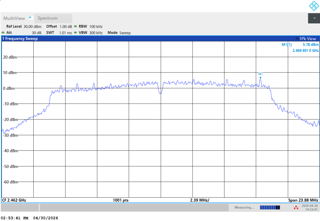
11G-Ant1-2462-PASS
