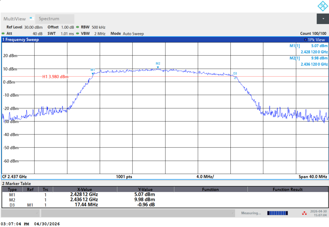
11VHT20SISO-Ant1-2437-PASS
