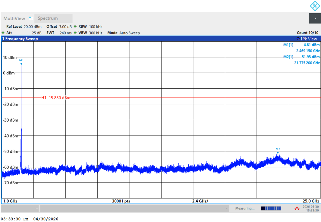
11AX20SISO-Ant1-2462-1000~25000-PASS
