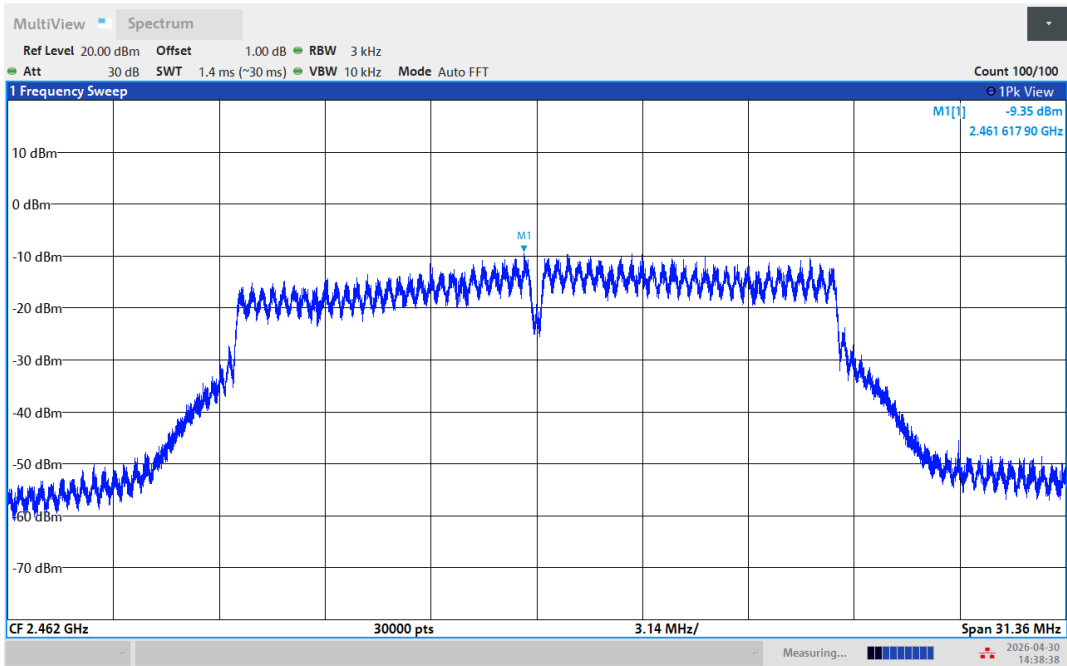
11AC20SISO-Ant1-2462-PASS
