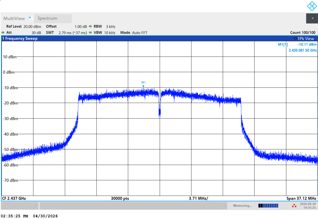
11AX20SISO-Ant1-2437-PASS
