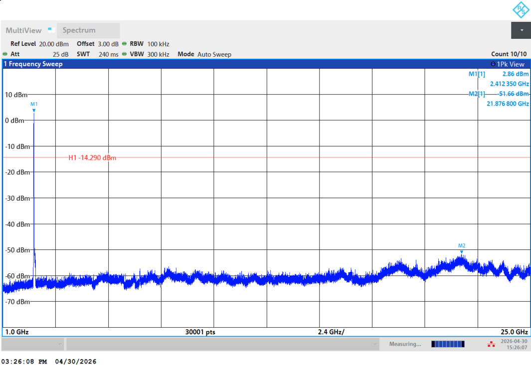
11N20SISO-Ant1-2412-1000~25000-PASS
