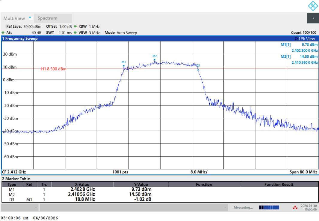
11AX20SISO-Ant1-2412-PASS
