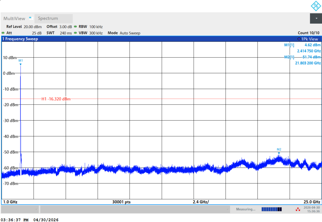
11AC20SISO-Ant1-2412-1000~25000-PASS
