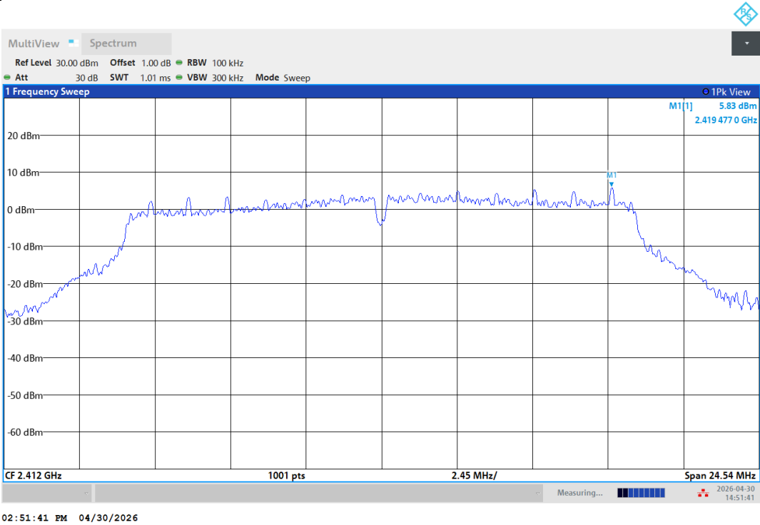
11G-Ant1-2412-PASS
