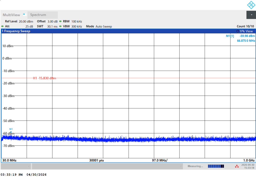
11AX20SISO-Ant1-2462-30~1000-PASS
