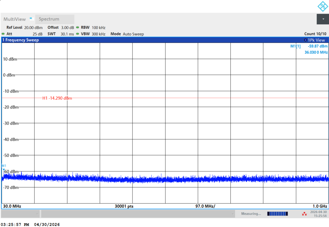
11N20SISO-Ant1-2412-30~1000-PASS
