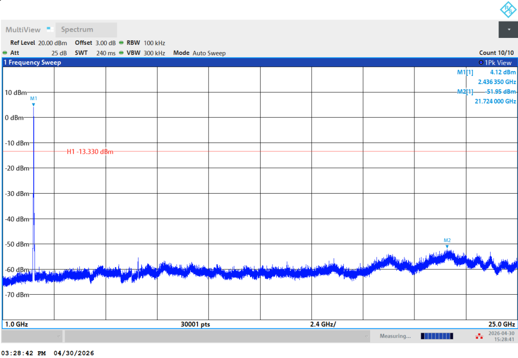
11N20SISO-Ant1-2437-1000~25000-PASS
