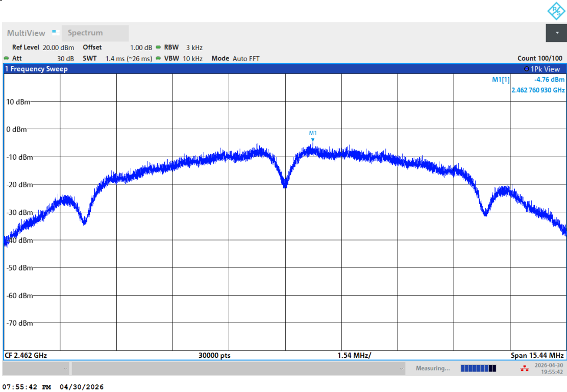
11B-Ant1-2462-PASS
