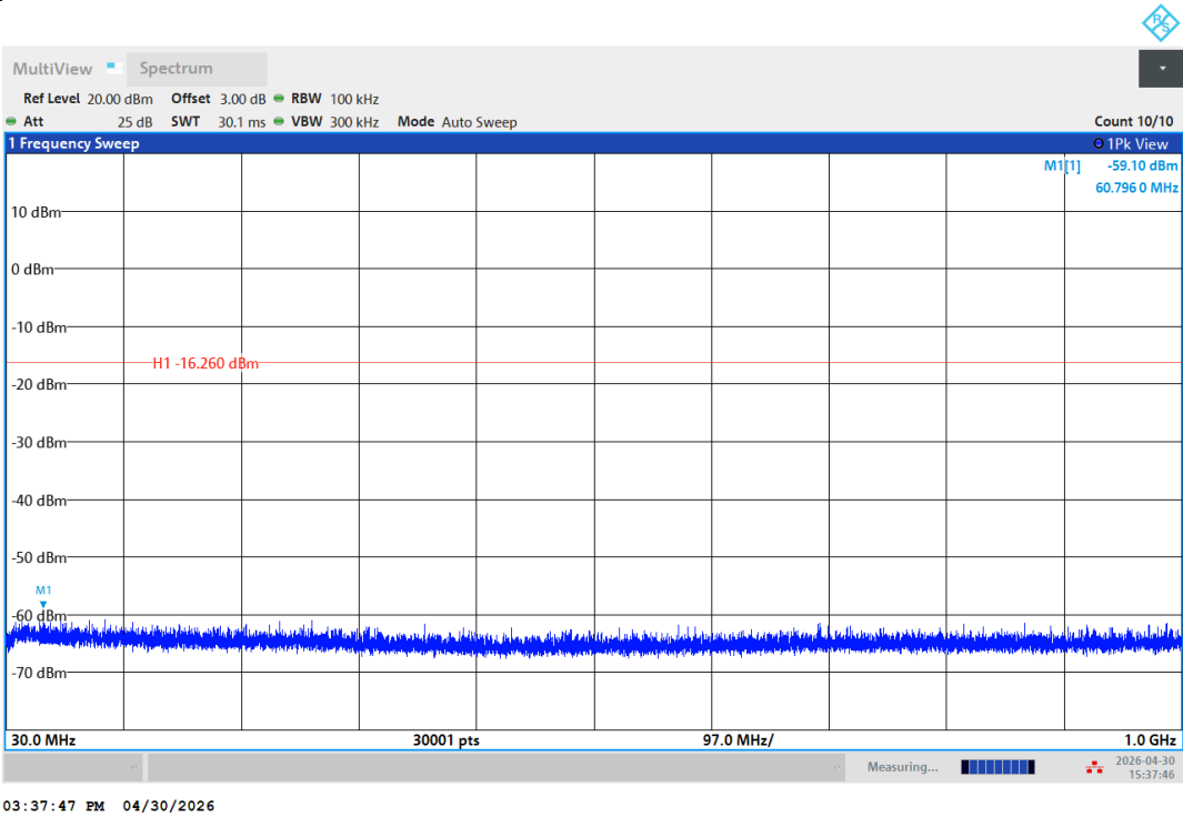
11AC20SISO-Ant1-2462-30~1000-PASS
