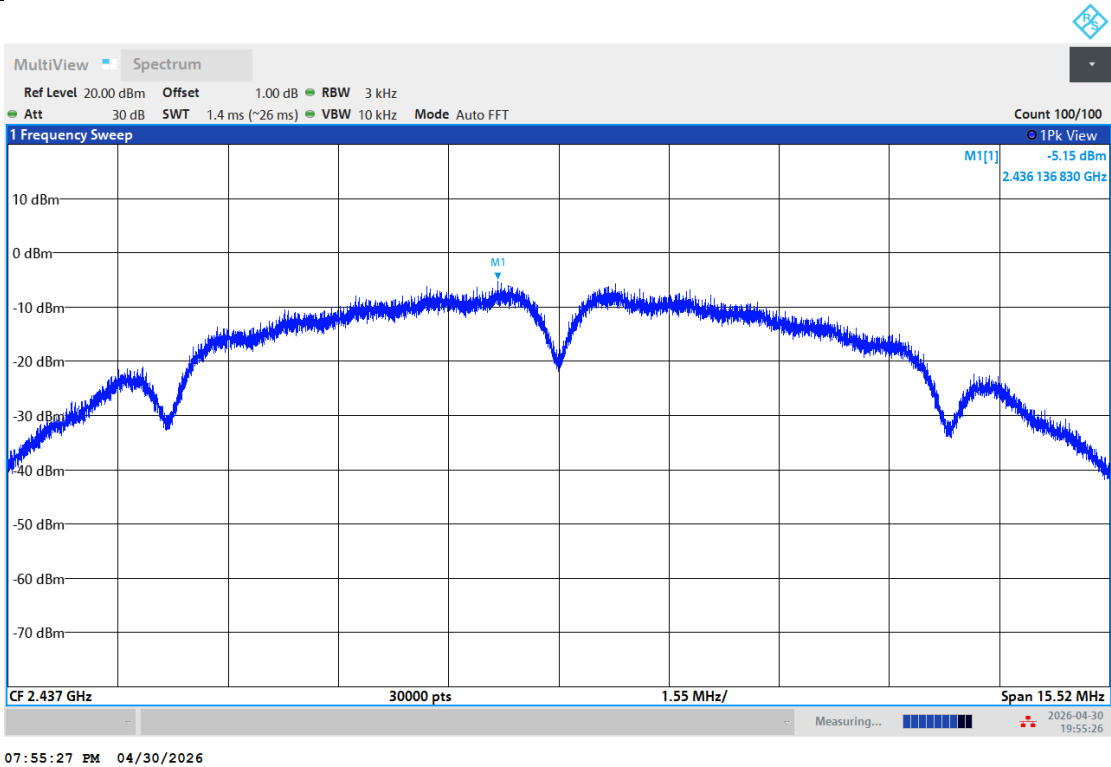
11B-Ant1-2437-PASS
