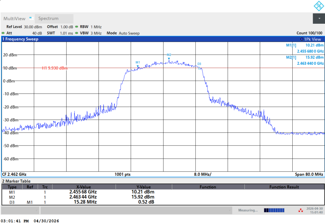
11AX20SISO-Ant1-2462-PASS
