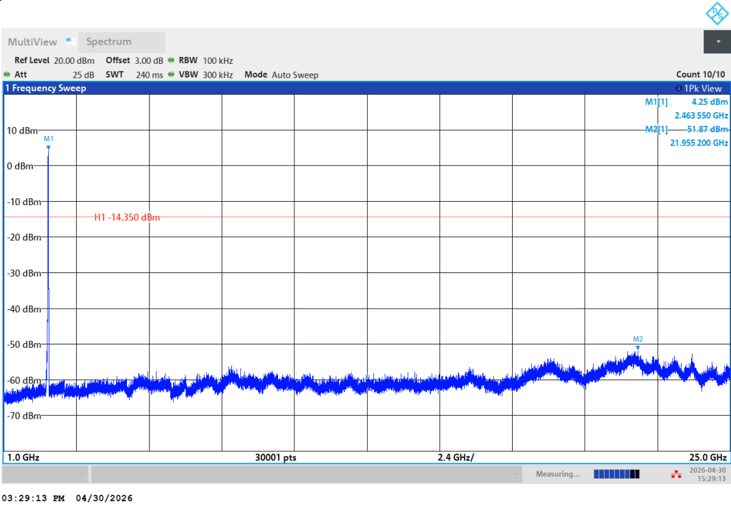
11N20SISO-Ant1-2462-1000~25000-PASS
