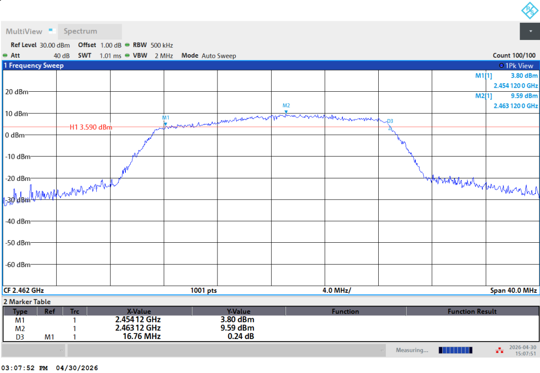
11VHT20SISO-Ant1-2462-PASS
