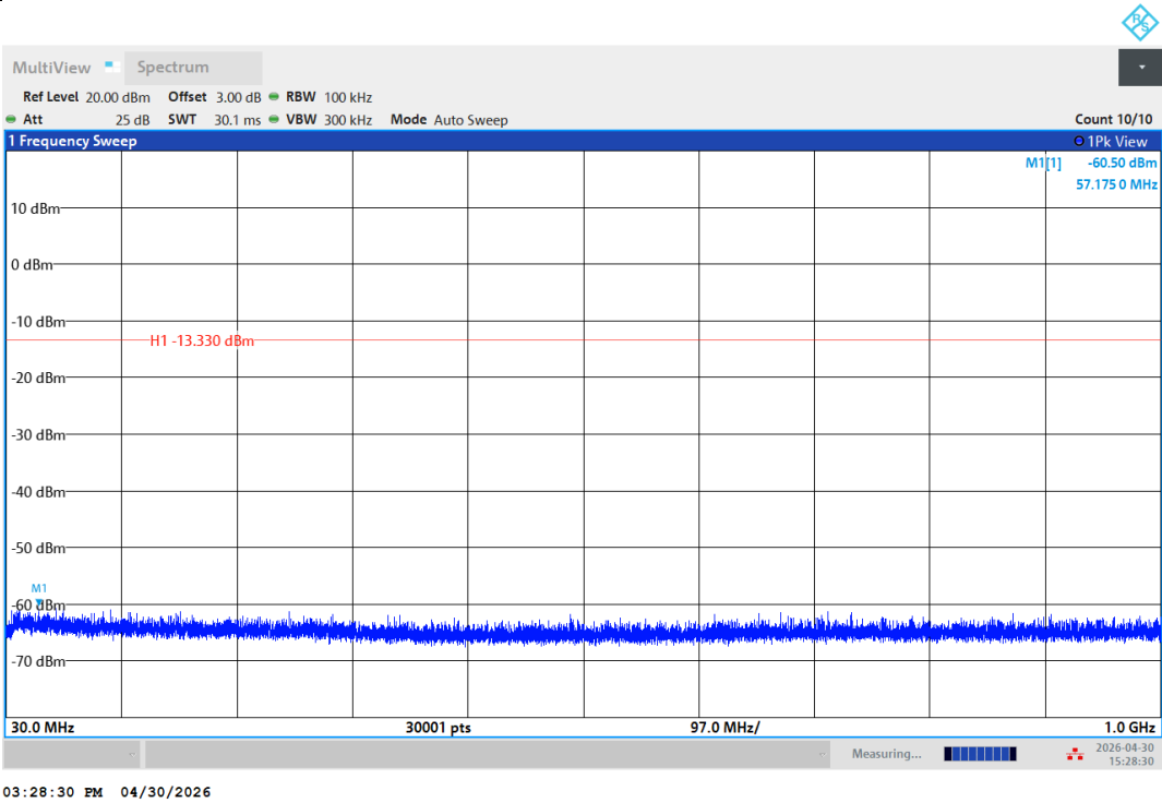
11N20SISO-Ant1-2437-30~1000-PASS
