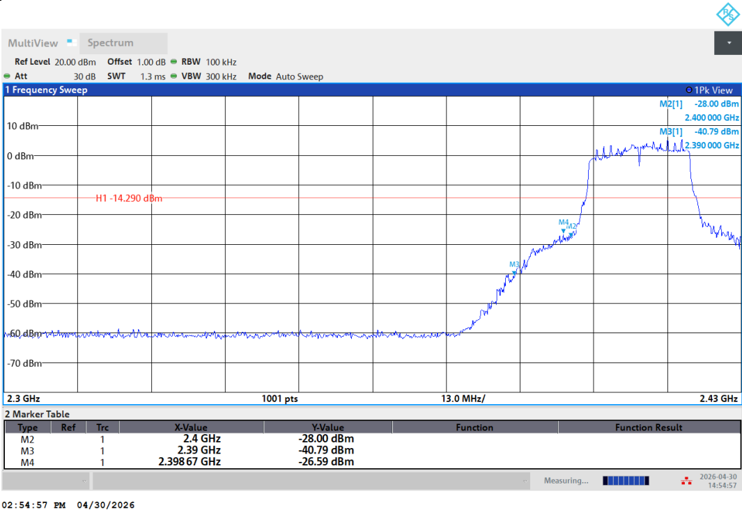
11N20SISO-Ant1-2412-PASS
