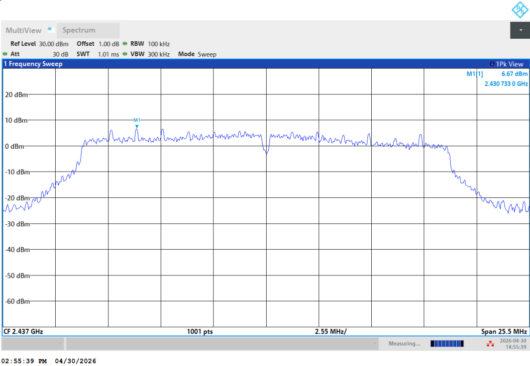
11N20SISO-Ant1-2437-PASS
