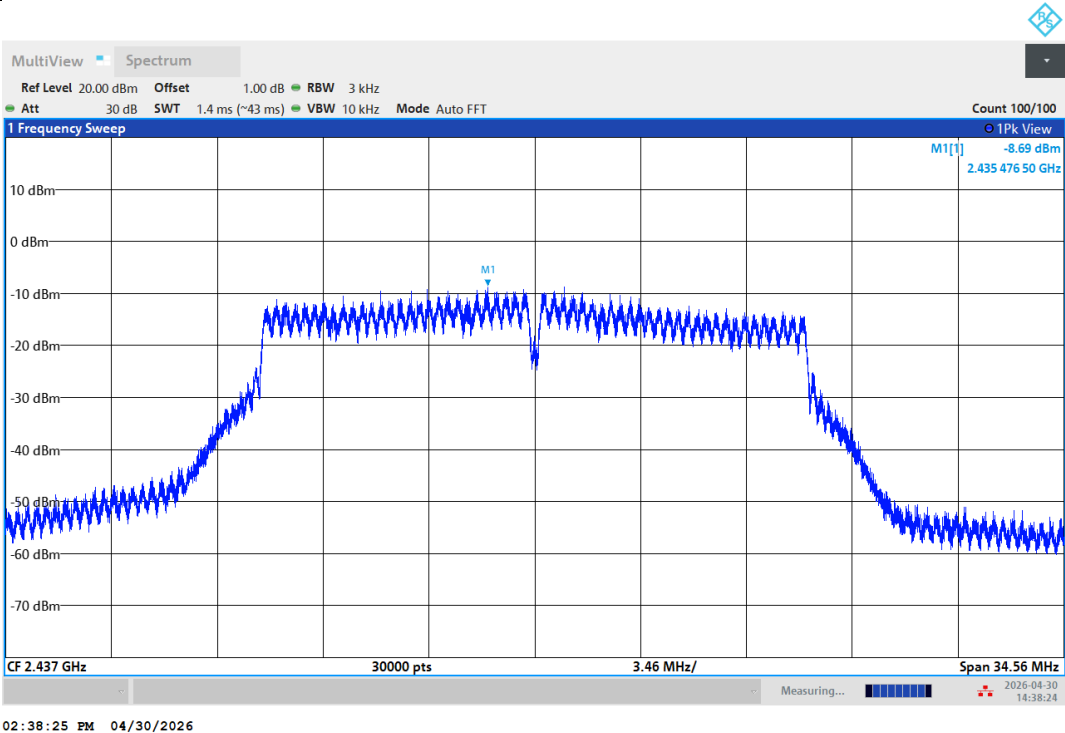
11AC20SISO-Ant1-2437-PASS
