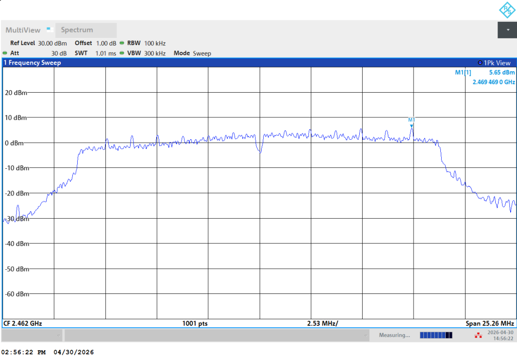
11N20SISO-Ant1-2462-PASS
