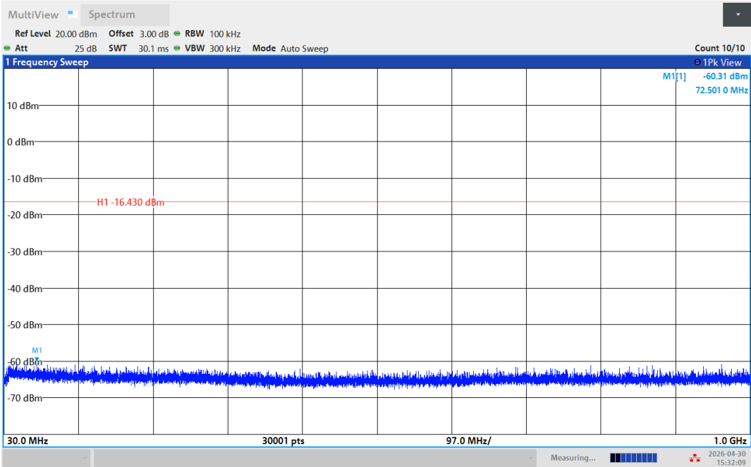
11AX20SISO-Ant1-2412-30~1000-PASS
