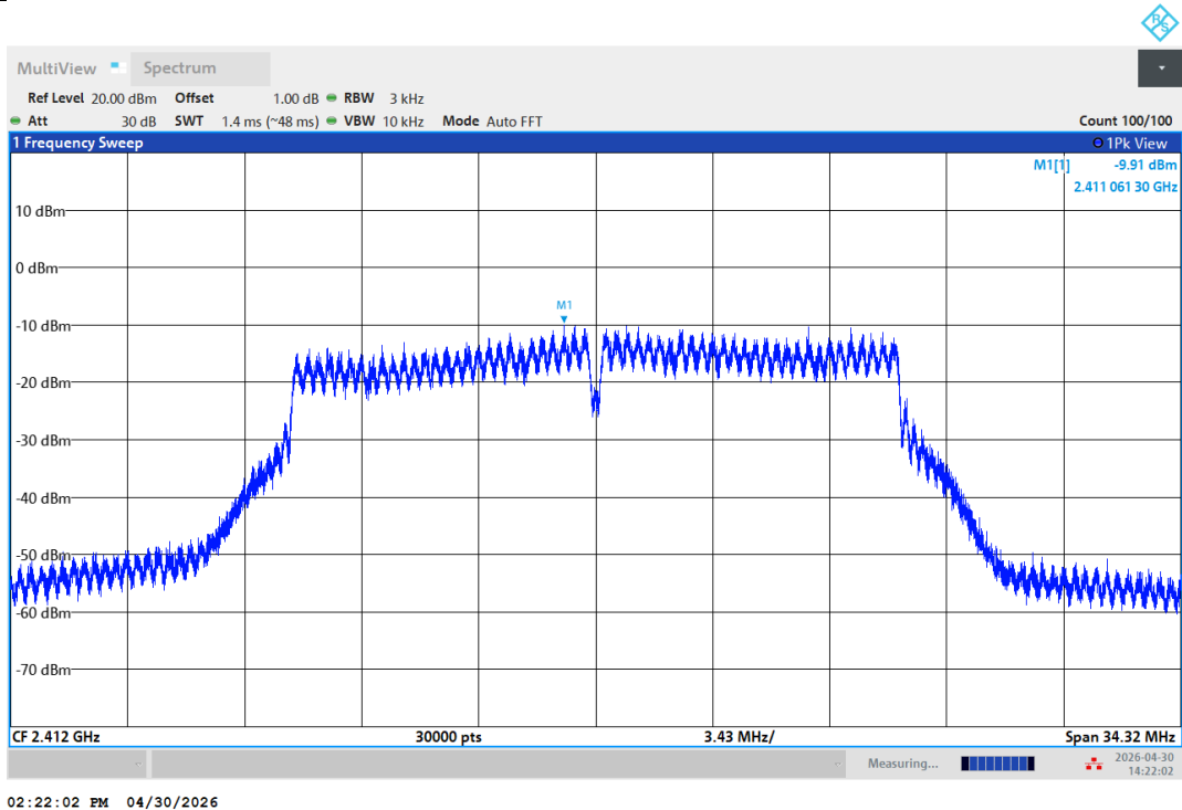
11N20SISO-Ant1-2412-PASS
