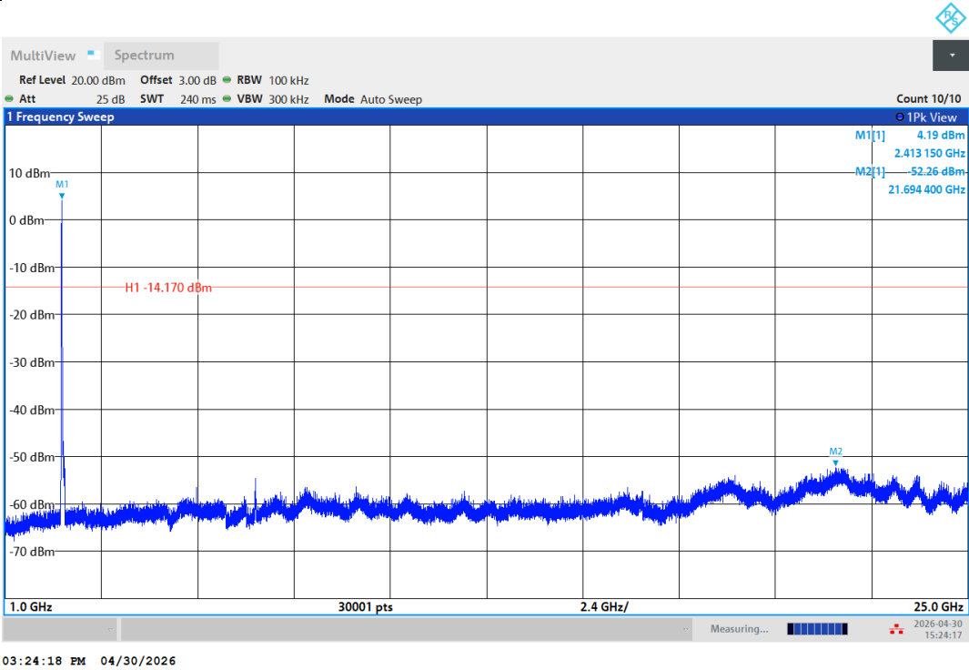
11G-Ant1-2412-1000~25000-PASS
