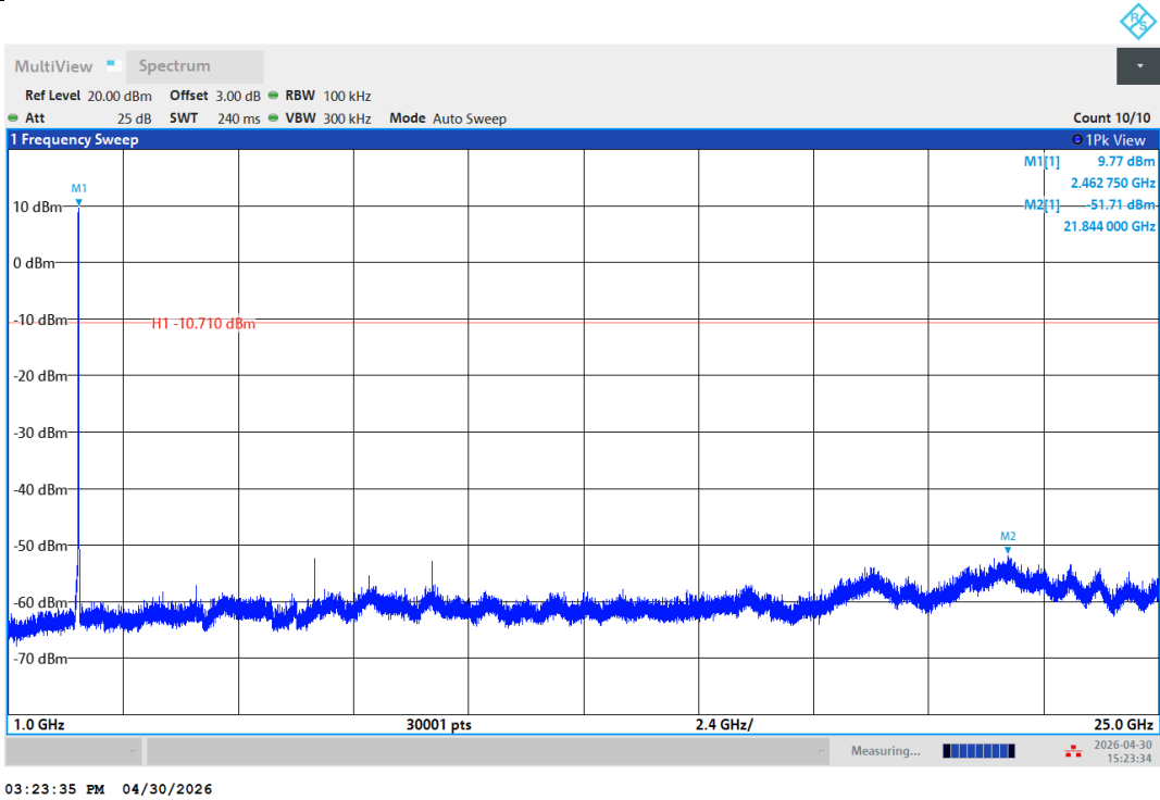
11B-Ant1-2462-1000~25000-PASS
