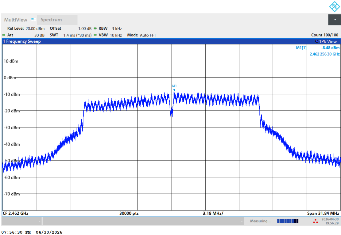
11G-Ant1-2462-PASS
