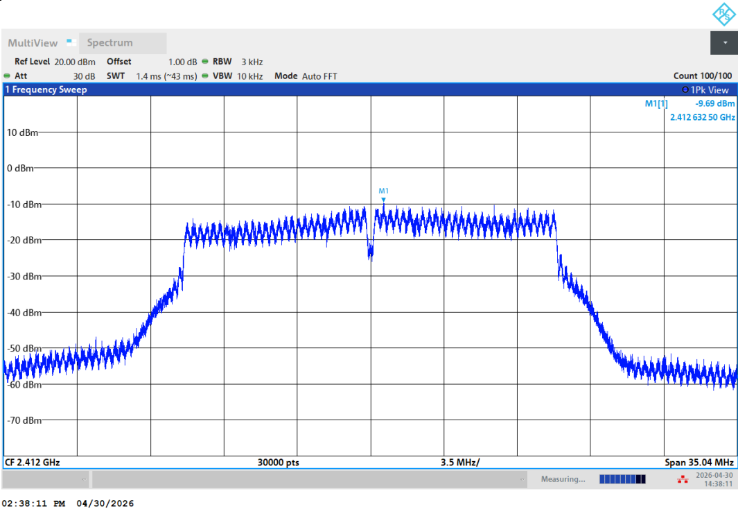
11AC20SISO-Ant1-2412-PASS
