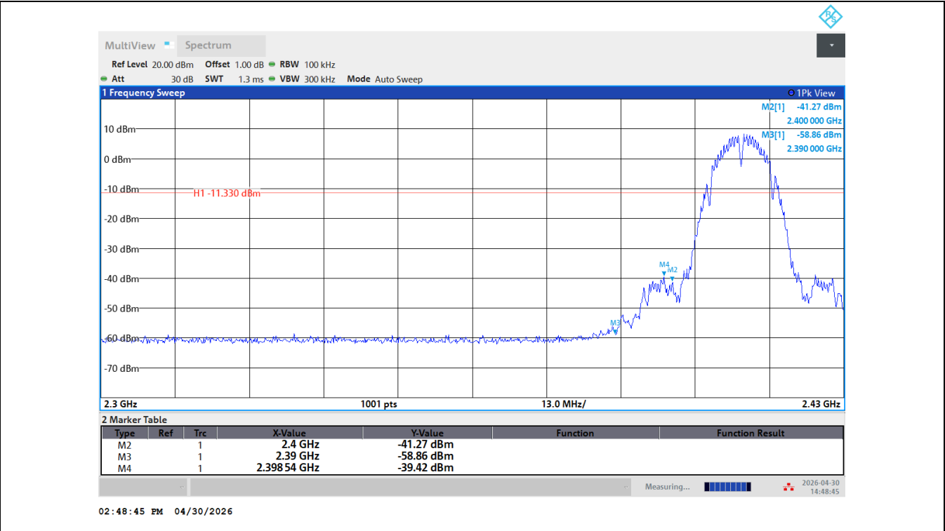
11B-Ant1-2412-PASS
