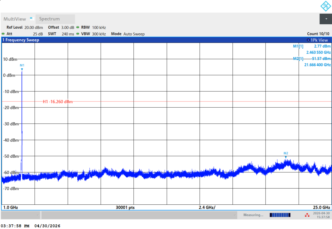
11AC20SISO-Ant1-2462-1000~25000-PASS
