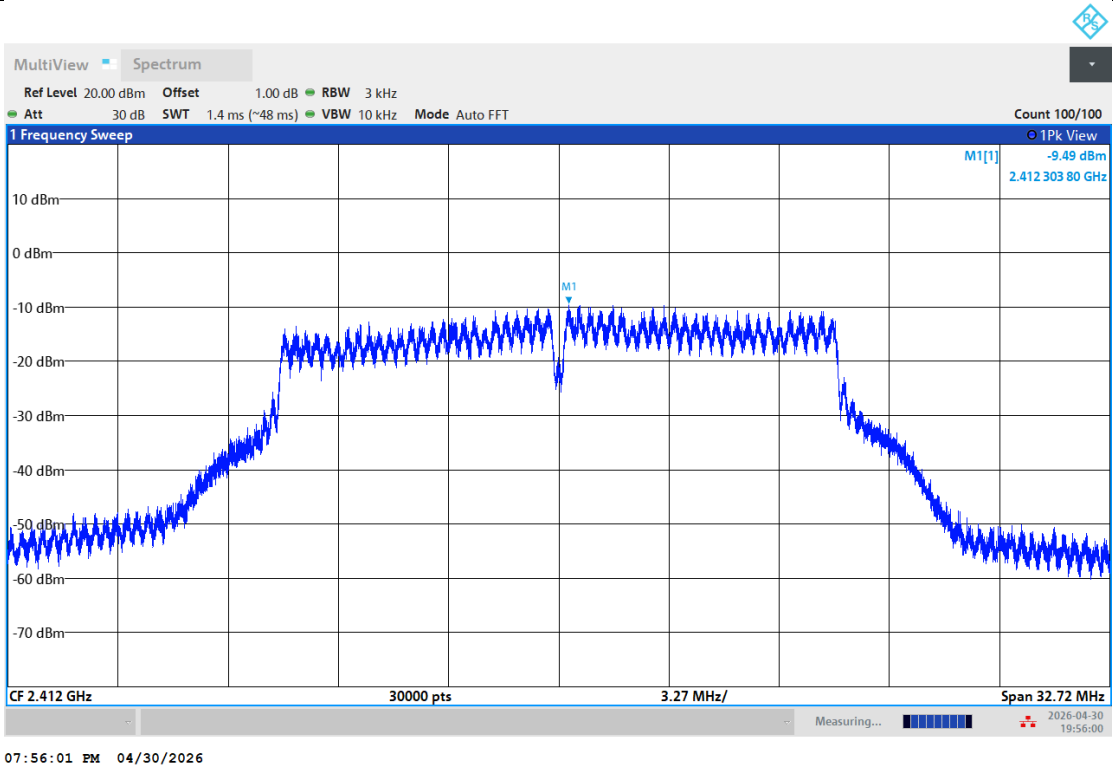
11G-Ant1-2412-PASS
