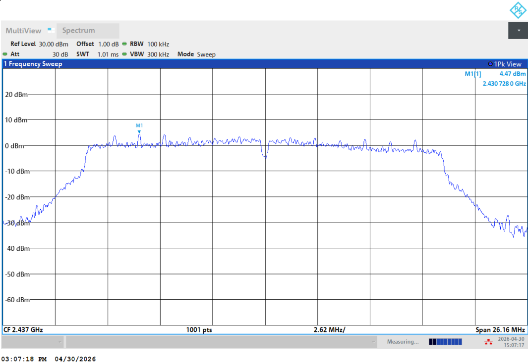
11AC20SISO-Ant1-2437-PASS
