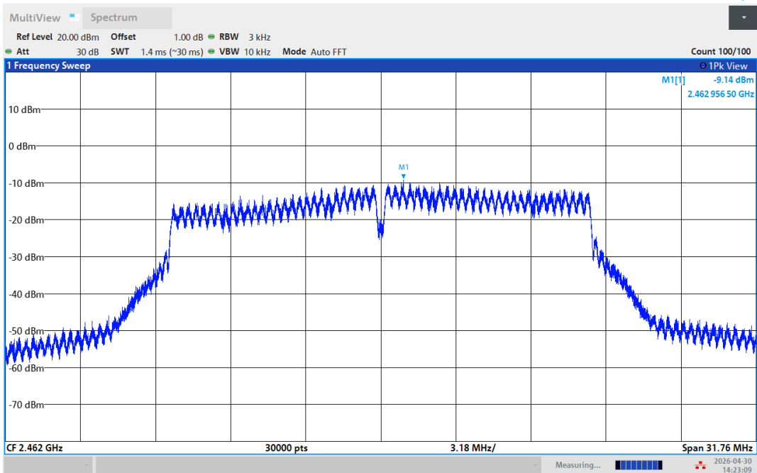
11N20SISO-Ant1-2462-PASS
