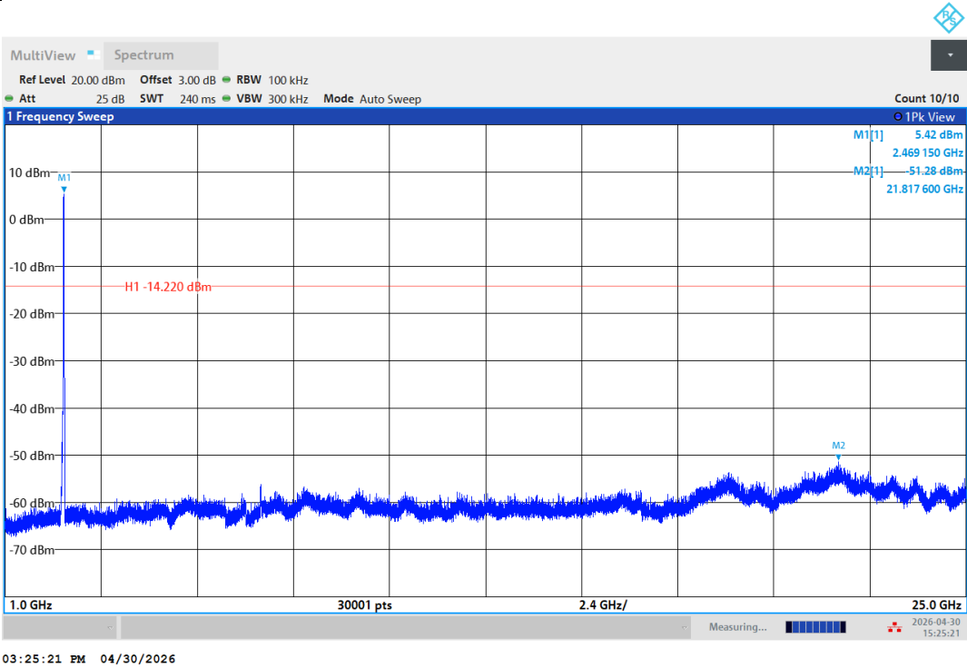
11G-Ant1-2462-1000~25000-PASS
