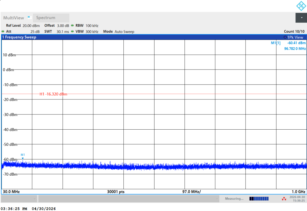
11AC20SISO-Ant1-2412-30~1000-PASS
