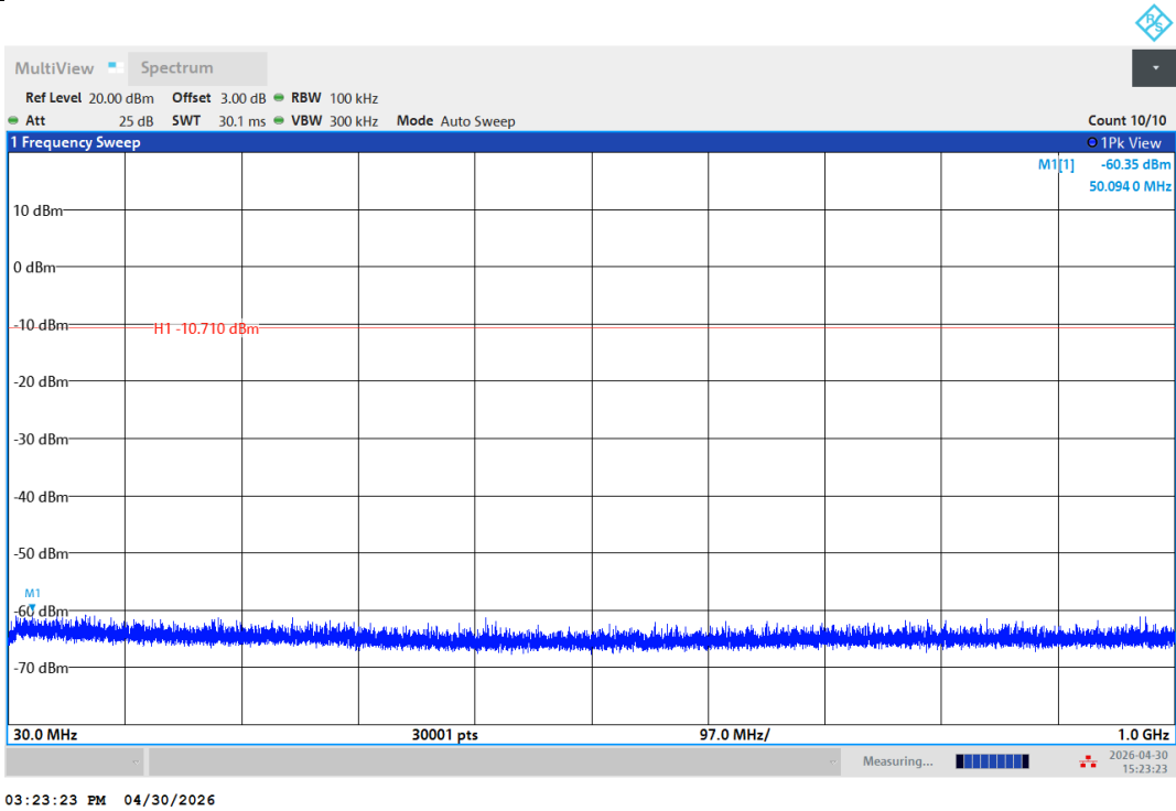
11B-Ant1-2462-30~1000-PASS
