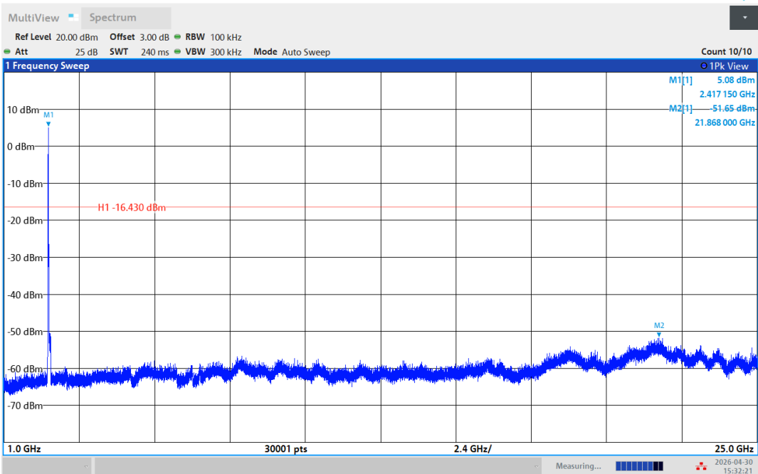
11AX20SISO-Ant1-2412-1000~25000-PASS
