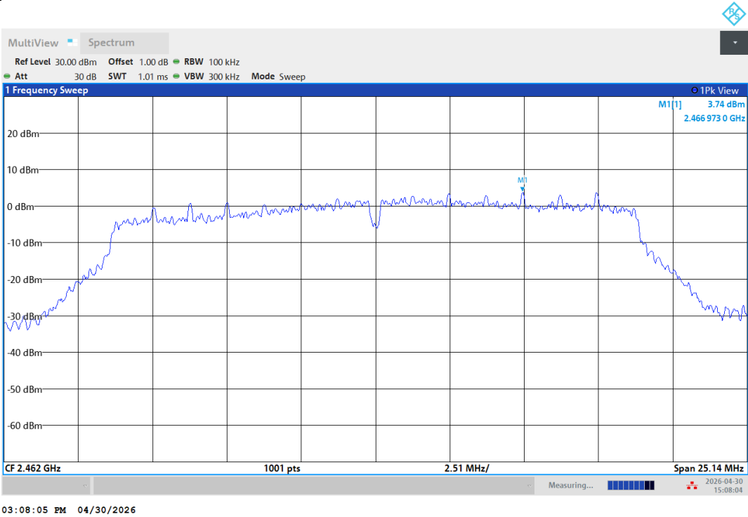
11AC20SISO-Ant1-2462-PASS
