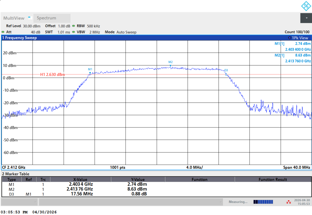
11VHT20SISO-Ant1-2412-PASS
