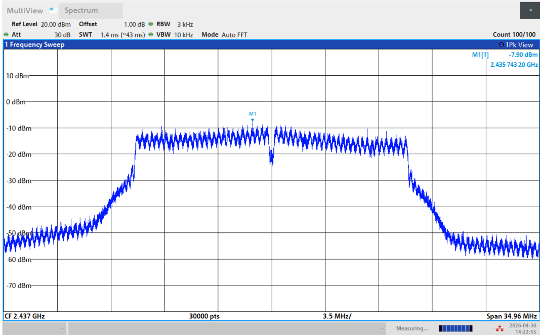
11N20SISO-Ant1-2437-PASS
