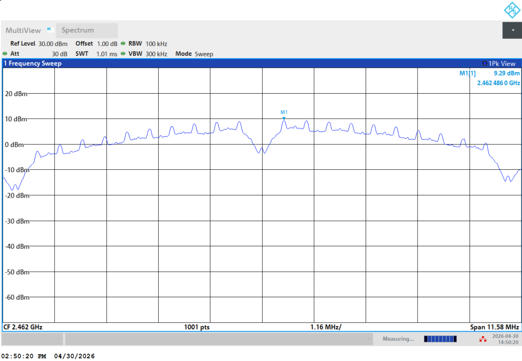
11B-Ant1-2462-PASS
