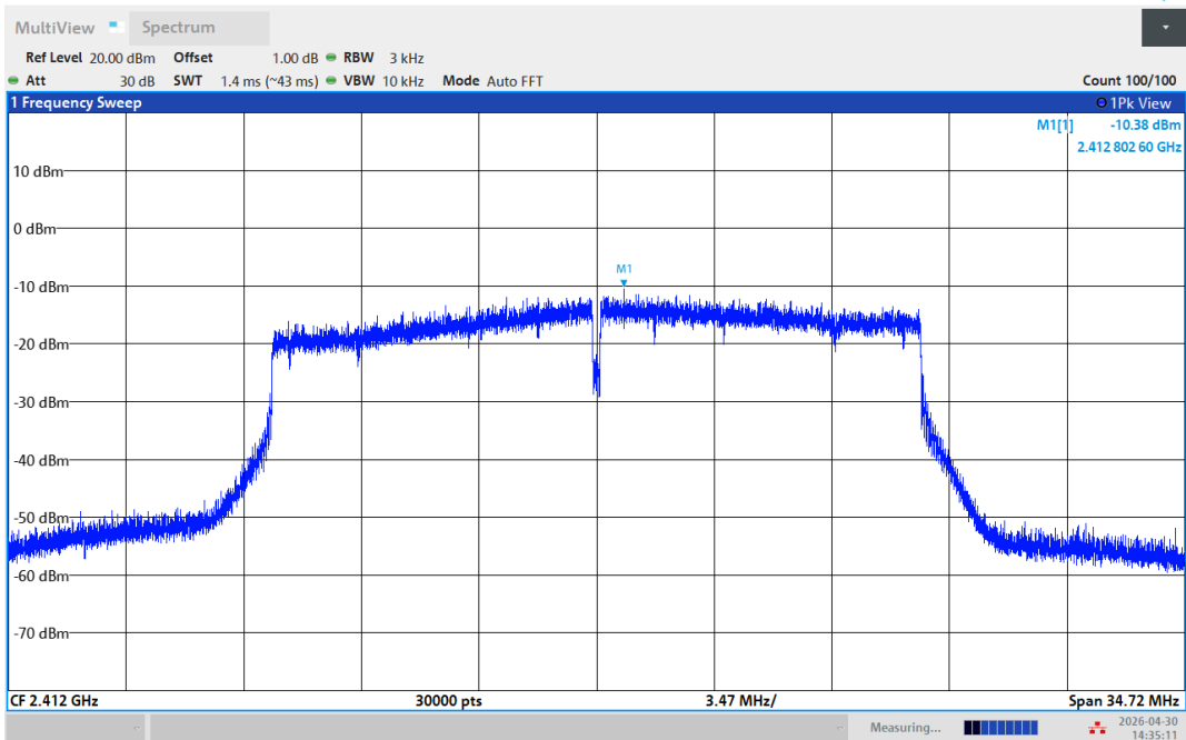
11AX20SISO-Ant1-2412-PASS
