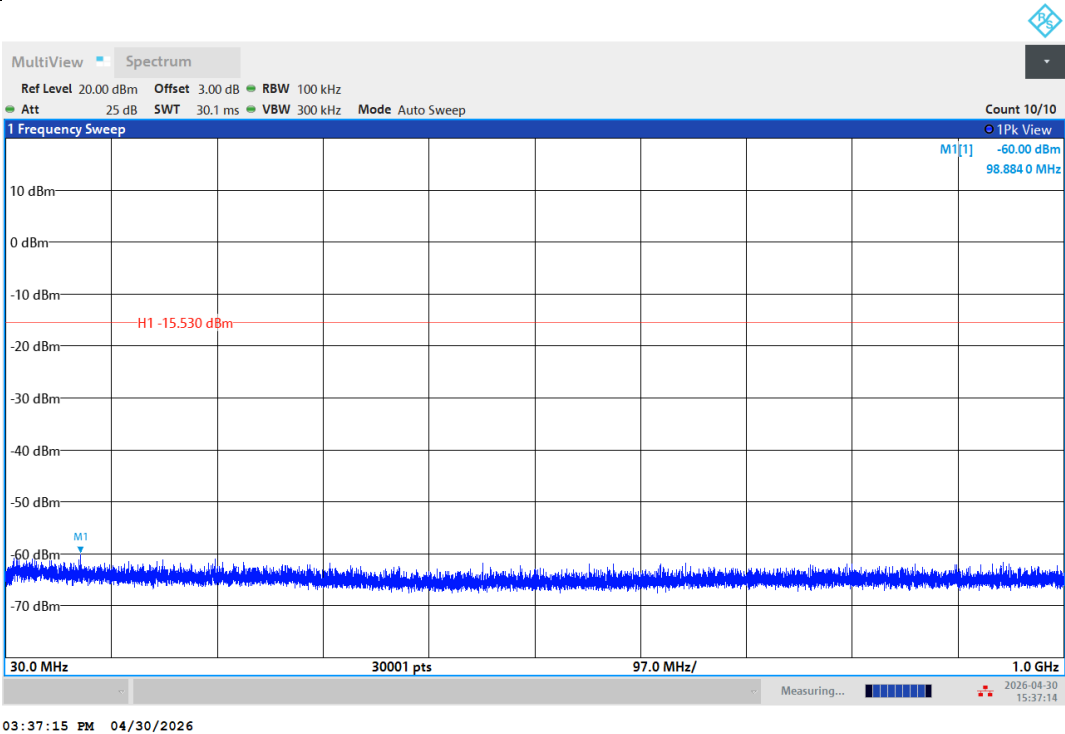
11AC20SISO-Ant1-2437-30~1000-PASS
