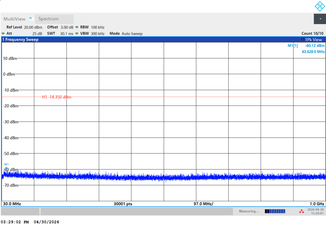
11N20SISO-Ant1-2462-30~1000-PASS
