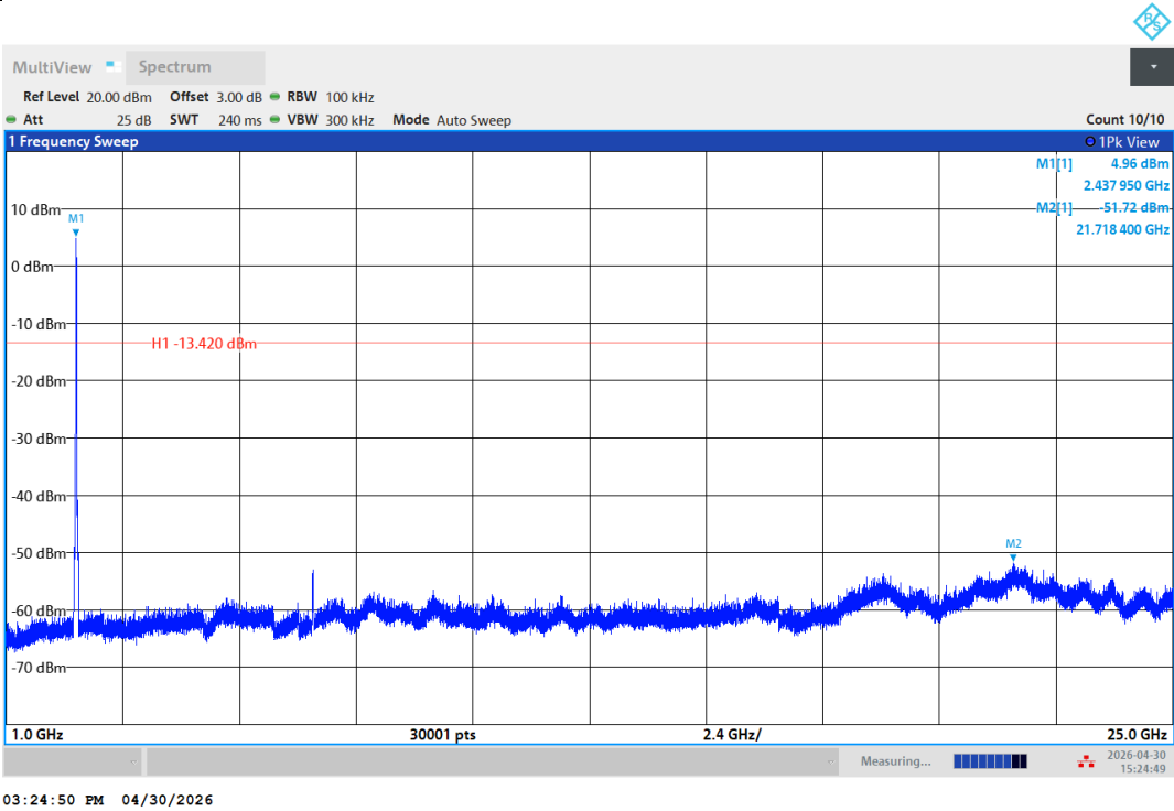
11G-Ant1-2437-1000~25000-PASS
