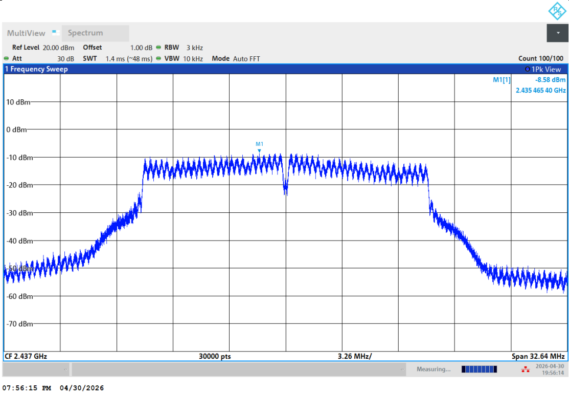
11G-Ant1-2437-PASS
