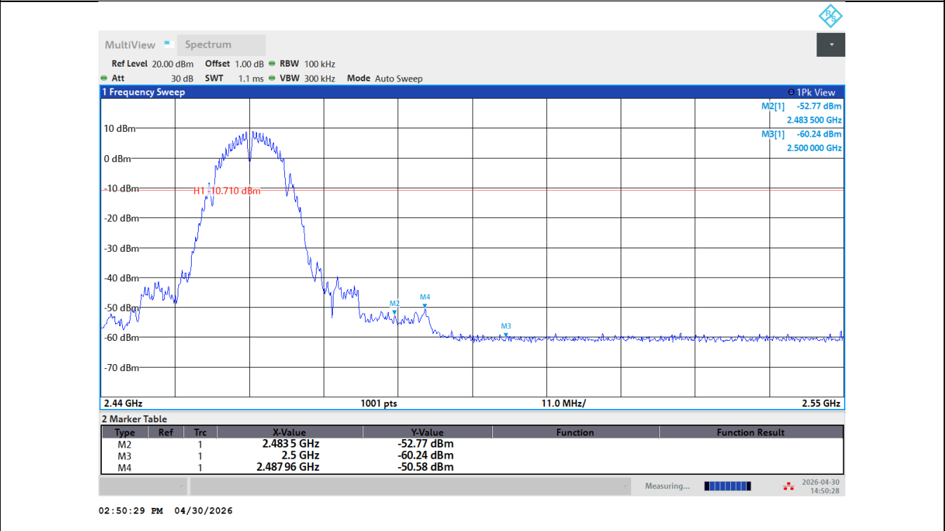
11B-Ant1-2462-PASS
