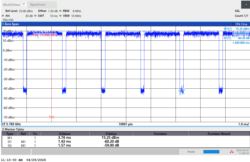
NTNV-11A-Ant1-5785
