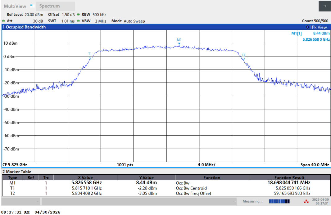
11AC20SISO-Ant1-5825
