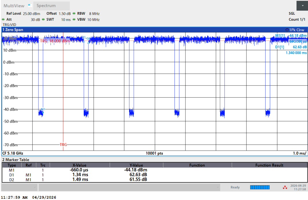
NTNV-11N20SISO-Ant1-5180
