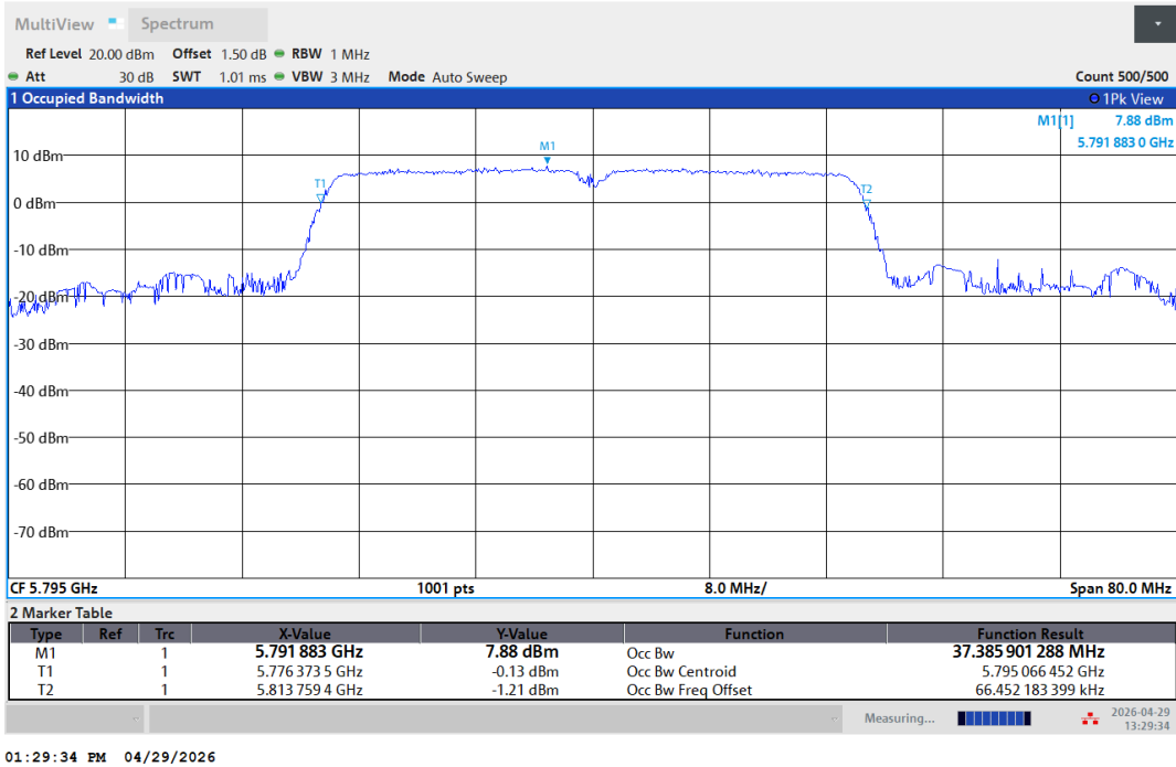
11N40SISO-Ant1-5795
