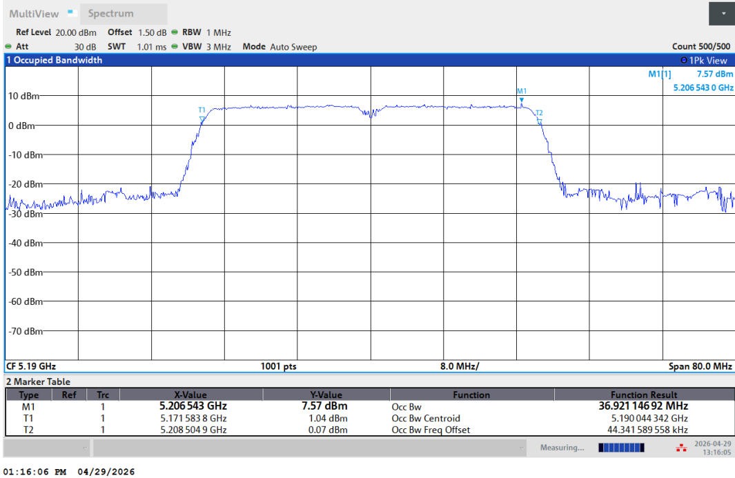
11N40SISO-Ant1-5190
