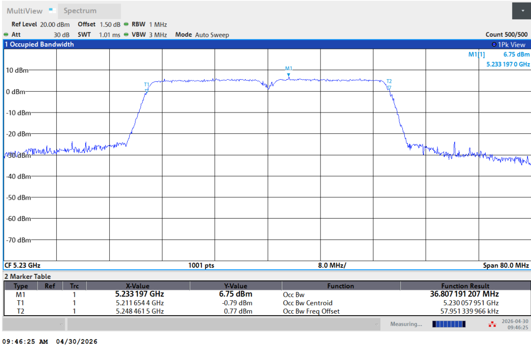
11AC40SISO-Ant1-5230
