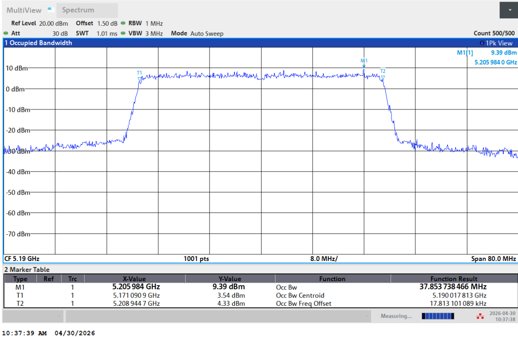
11AX40SISO-Ant1-5190
