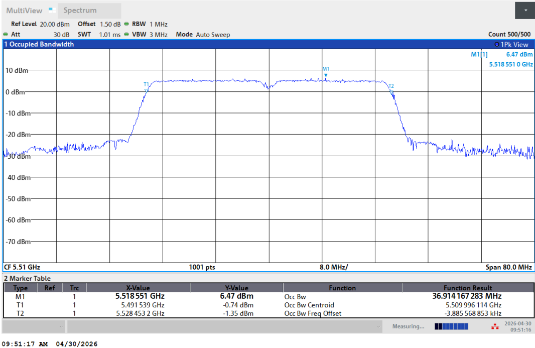
11AC40SISO-Ant1-5510
