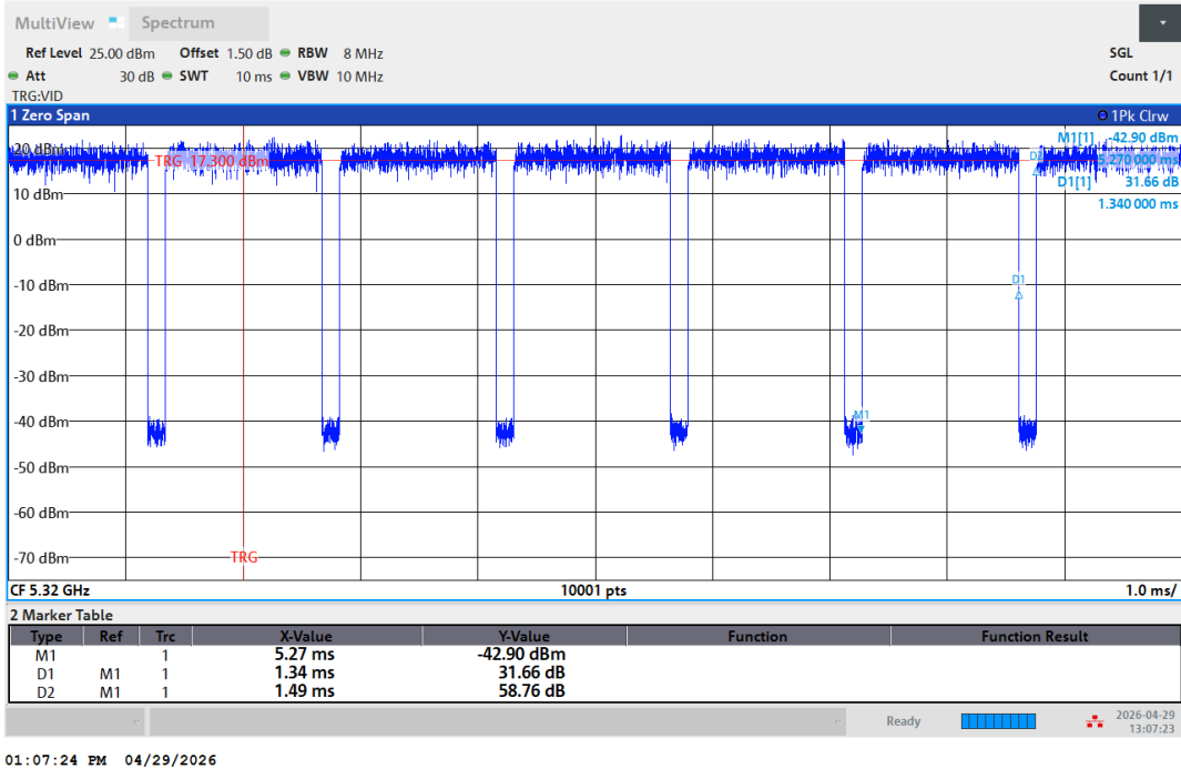
NTNV-11N20SISO-Ant1-5320
