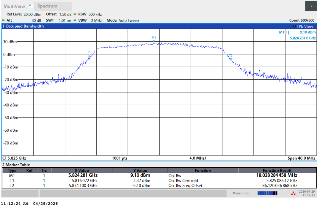
11A-Ant1-5825
