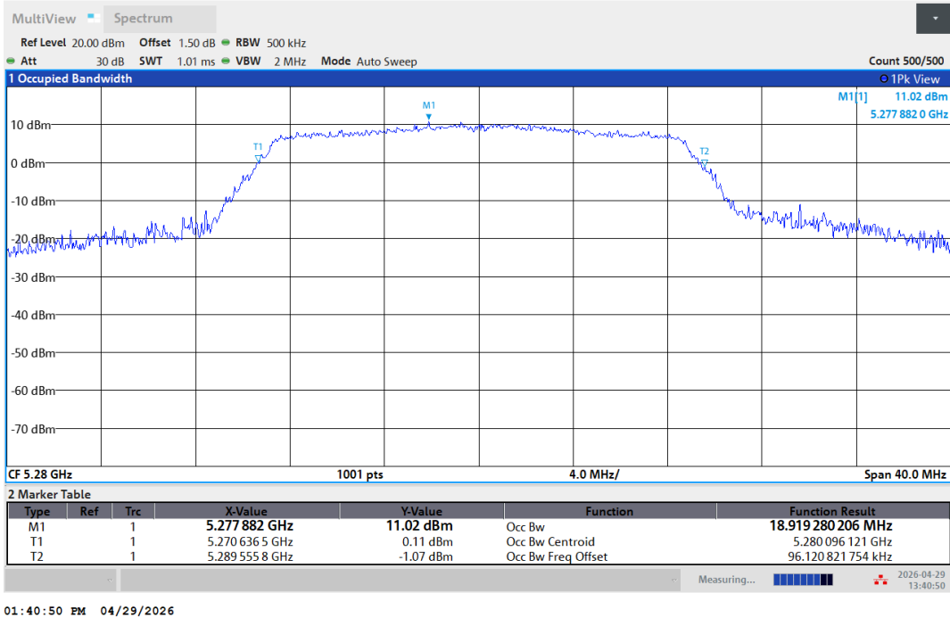
11AC20SISO-Ant1-5280
