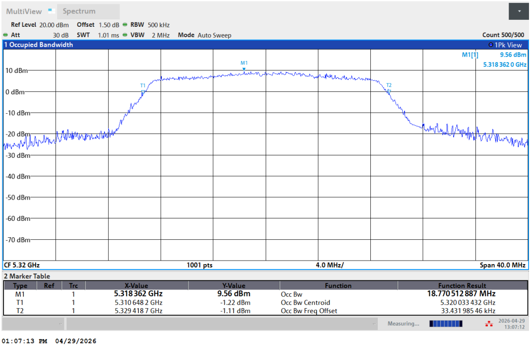
11N20SISO-Ant1-5320
