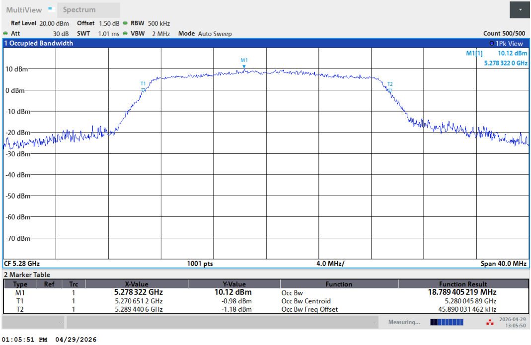
11N20SISO-Ant1-5280
