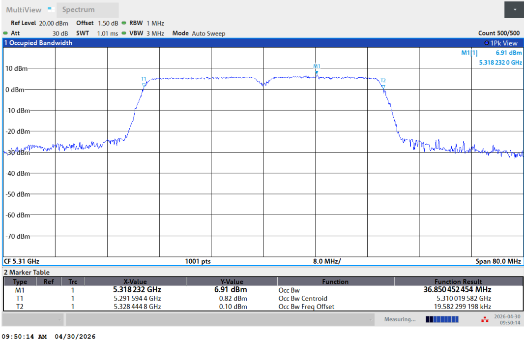
11AC40SISO-Ant1-5310
