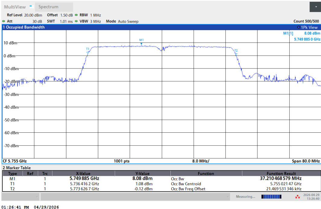
11N40SISO-Ant1-5755
