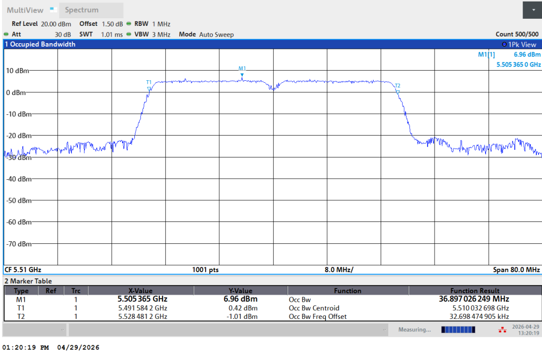
11N40SISO-Ant1-5510
