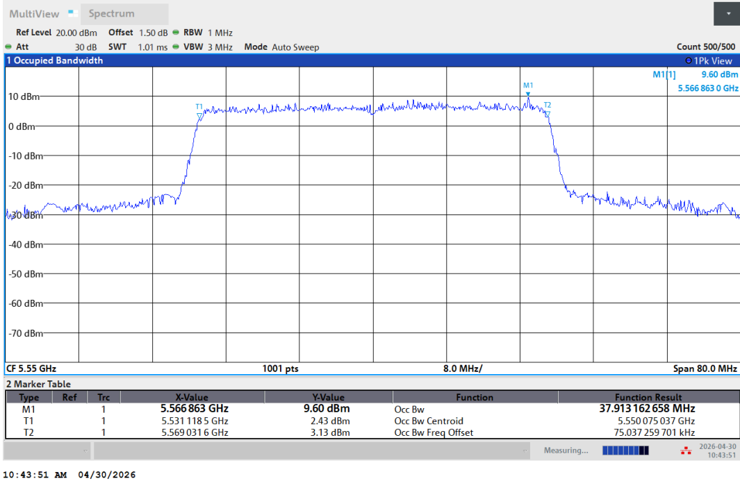
11AX40SISO-Ant1-5550
