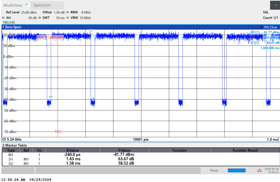
NTNV-11A-Ant1-5240
