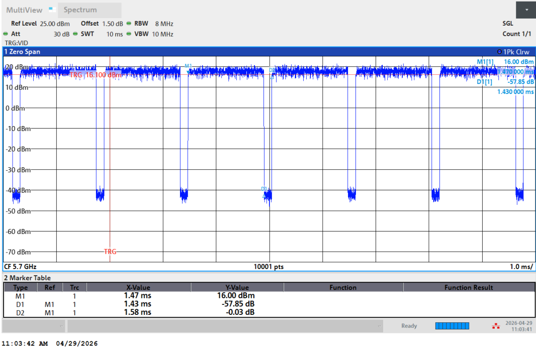
NTNV-11A-Ant1-5700
