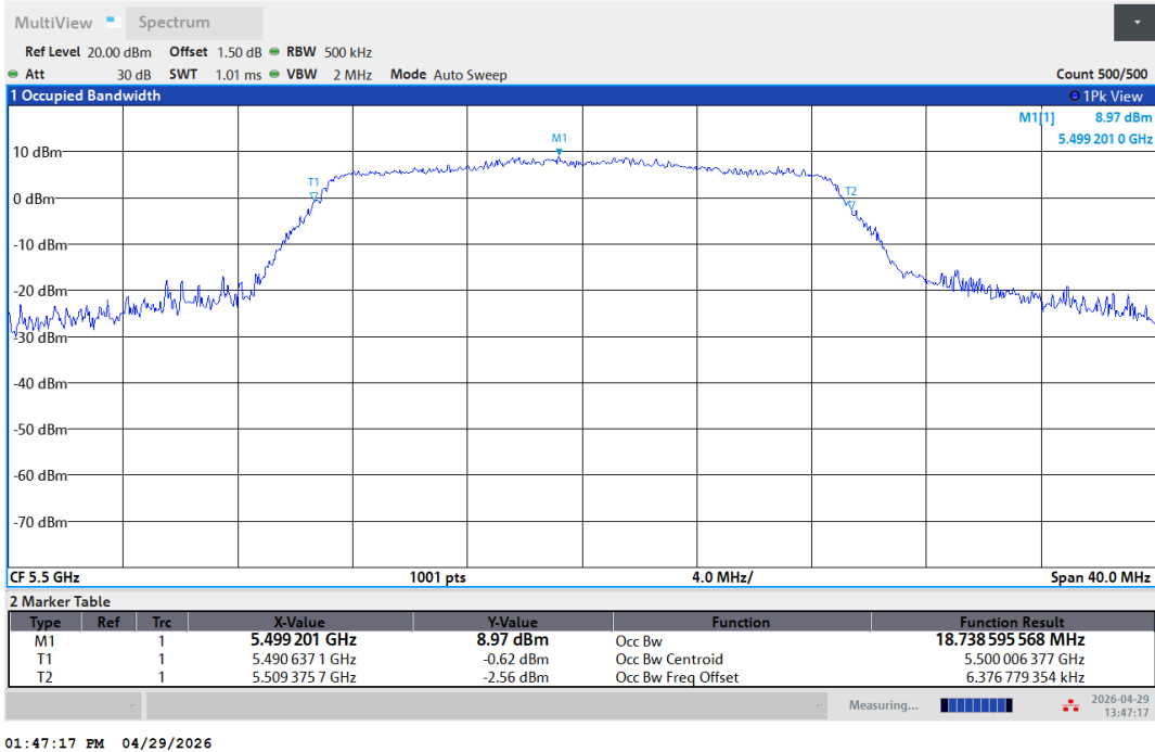
11AC20SISO-Ant1-5500
