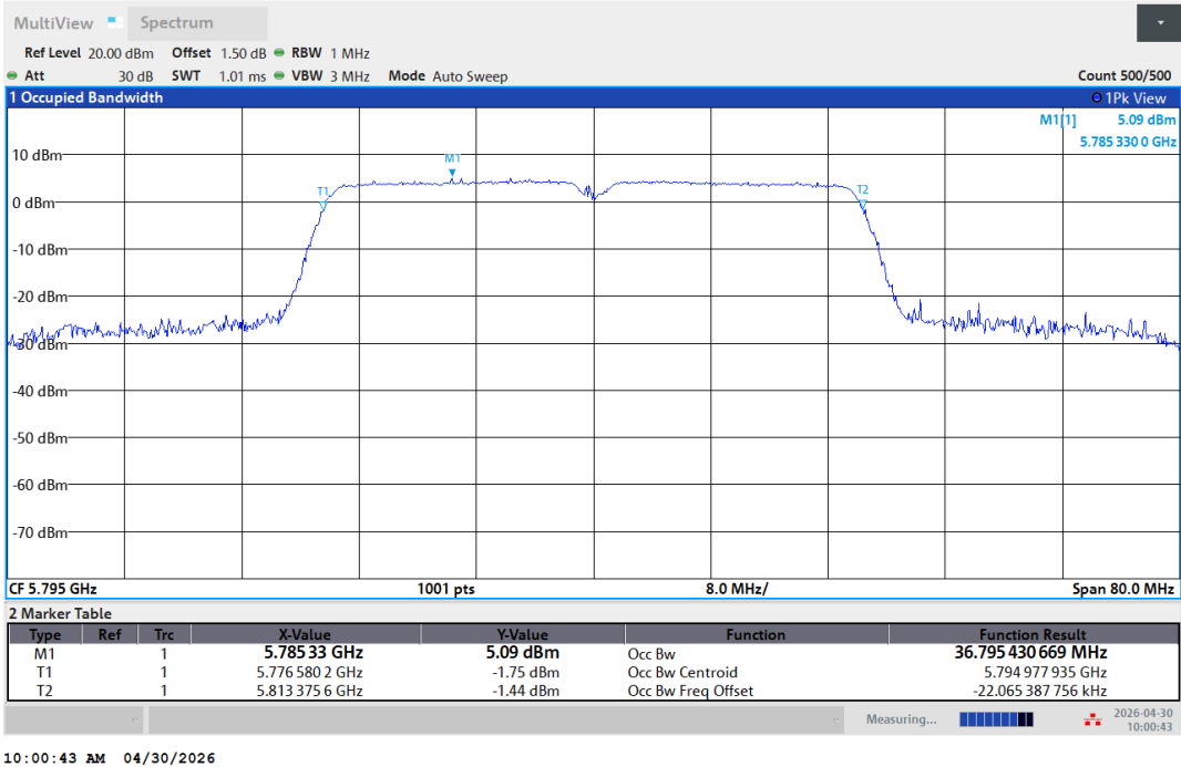
11AC40SISO-Ant1-5795
