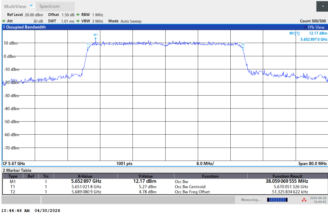
11AX40SISO-Ant1-5670
