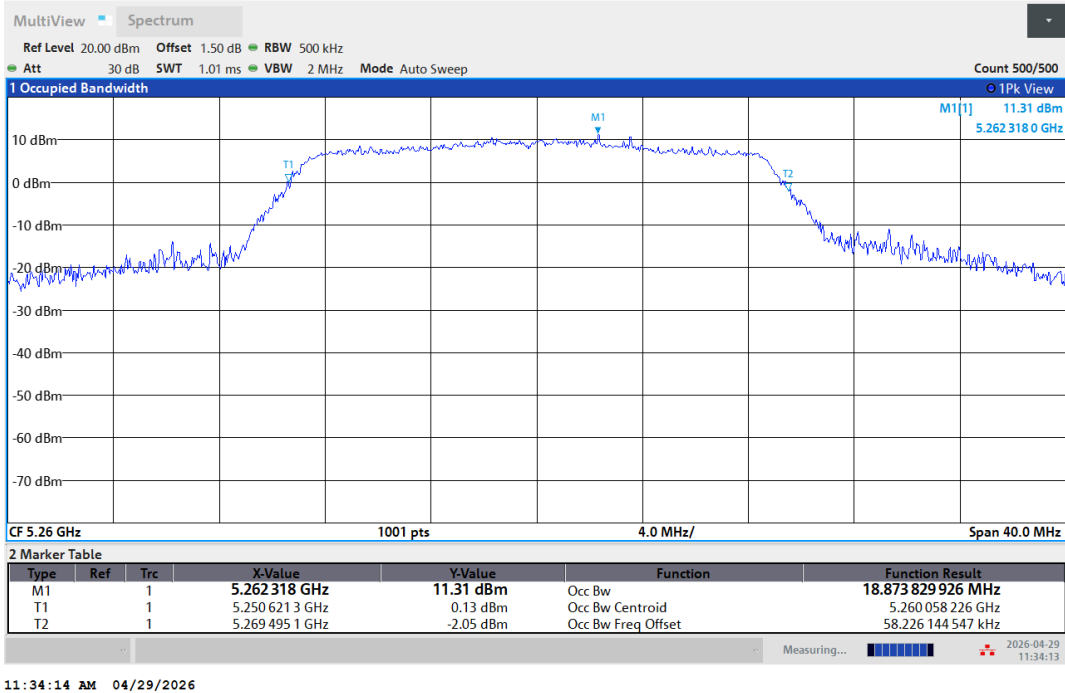
11N20SISO-Ant1-5260
