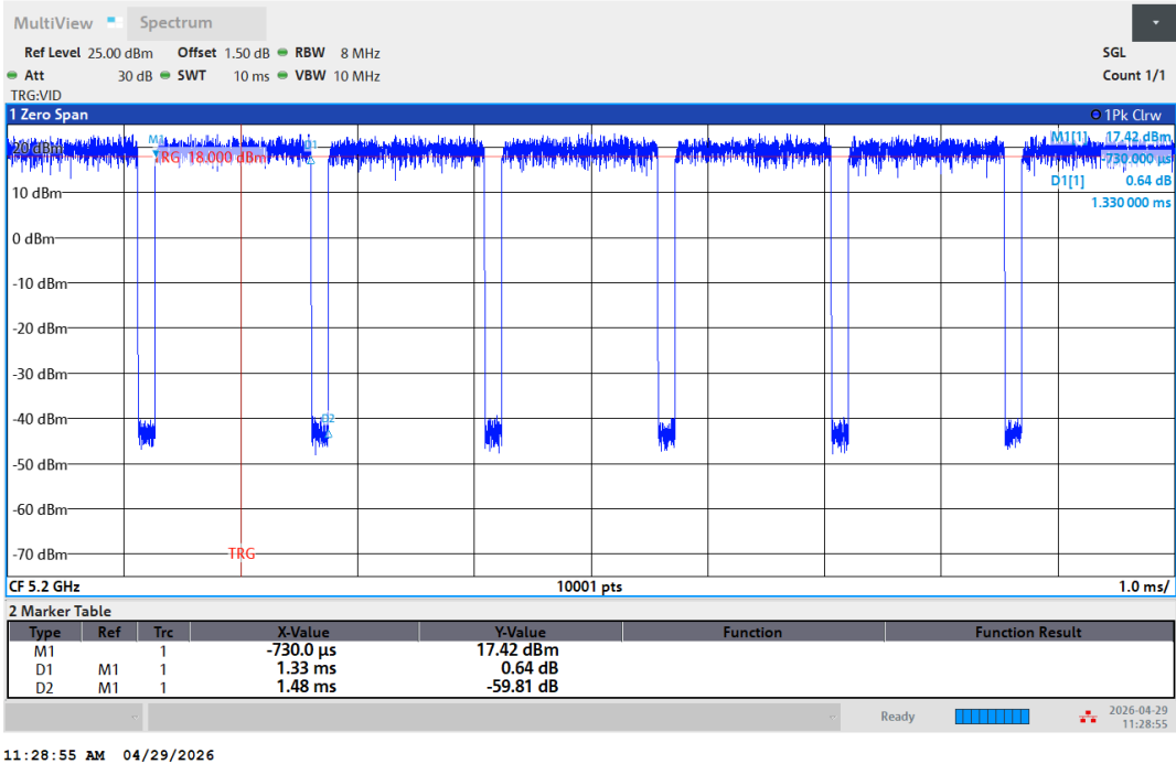
NTNV-11N20SISO-Ant1-5200
