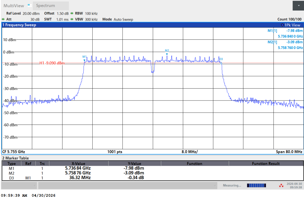
11AC40SiSO-Ant1-5755-PASS
