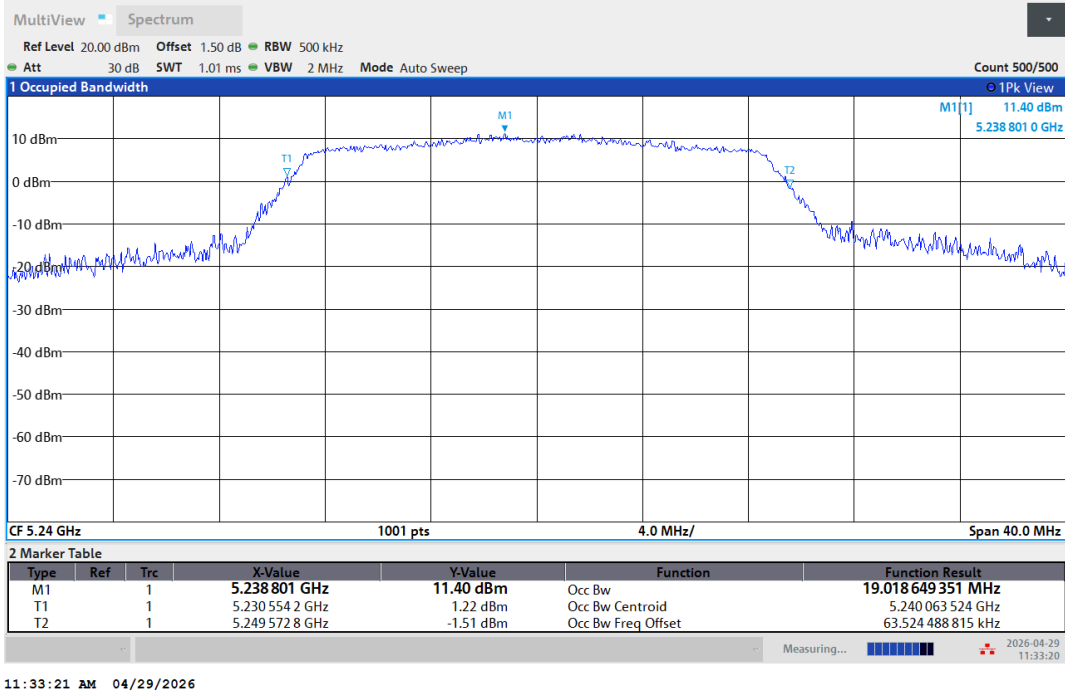
11N20SISO-Ant1-5240
