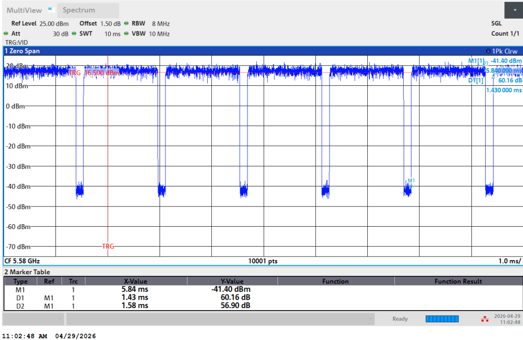
NTNV-11A-Ant1-5580
