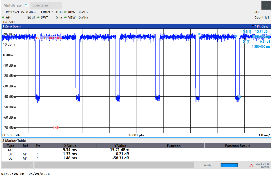
NTNV-11N20SISO-Ant1-5580
