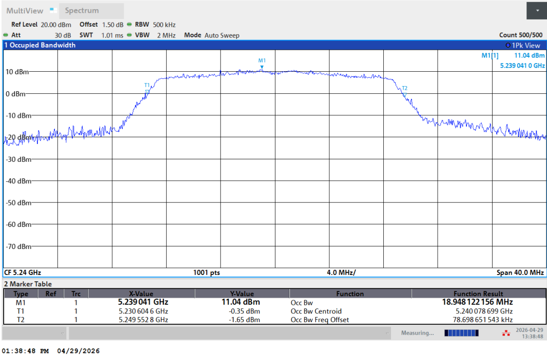
11AC20SISO-Ant1-5240
