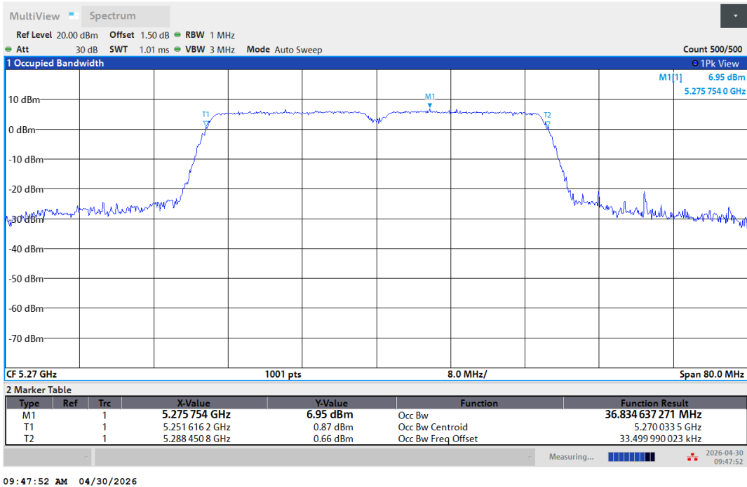
11AC40SISO-Ant1-5270
