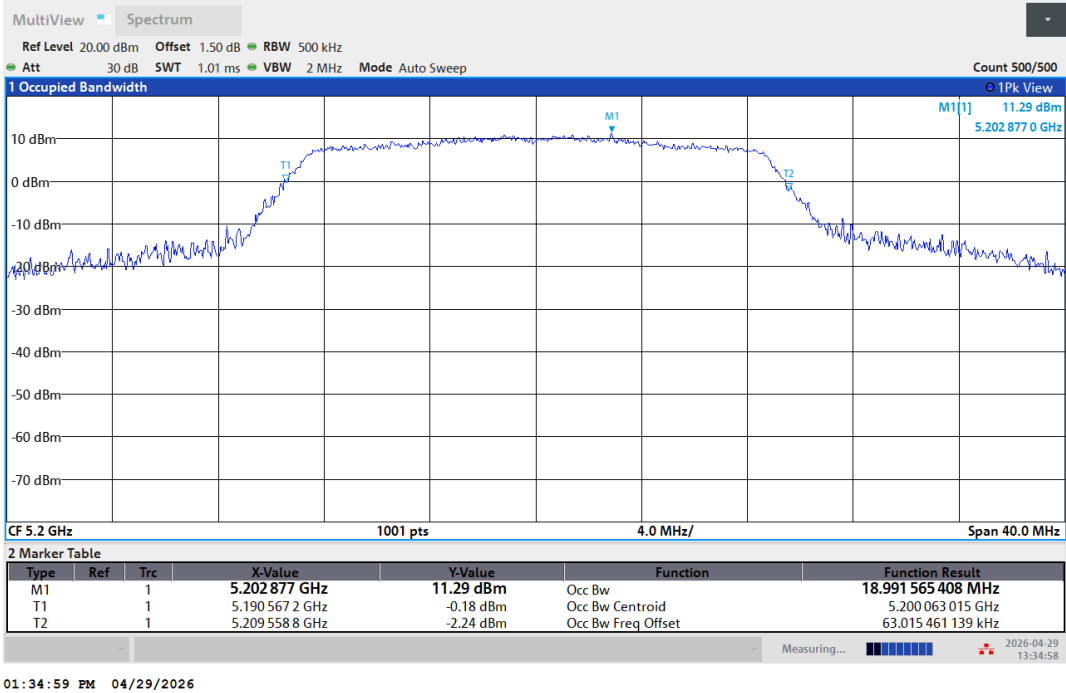
11AC20SISO-Ant1-5200
