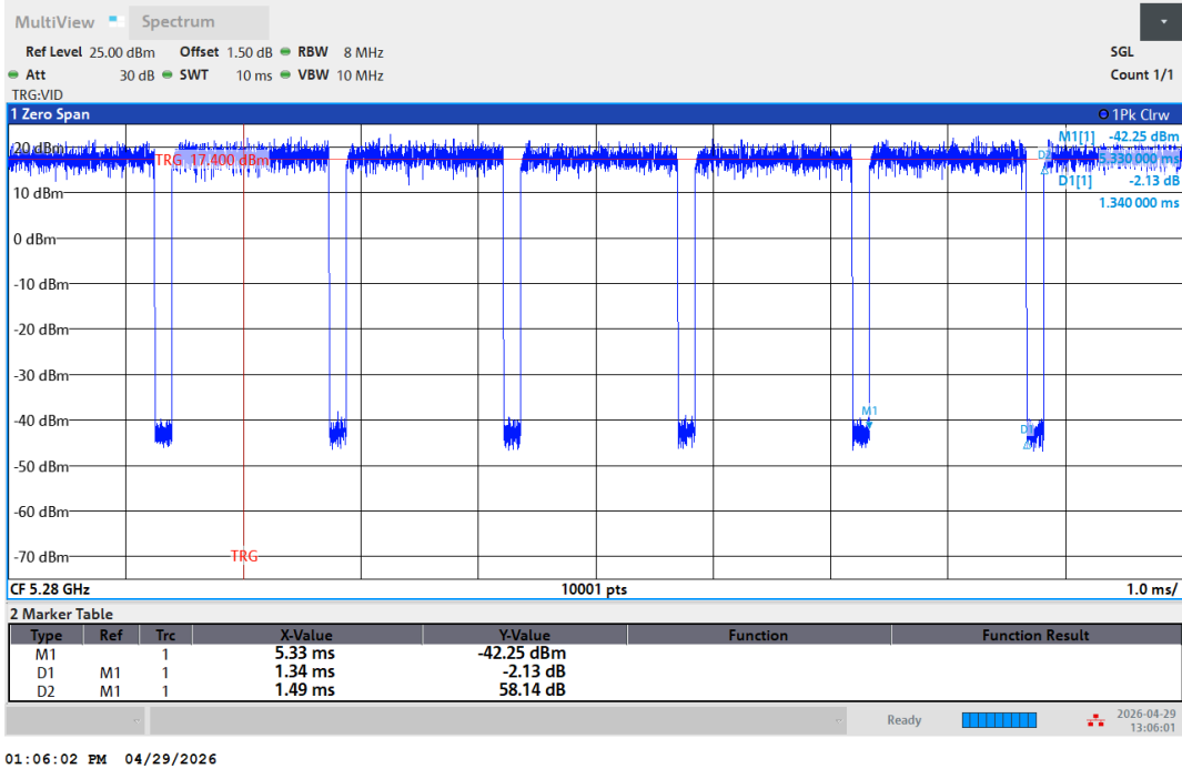
NTNV-11N20SISO-Ant1-5280
