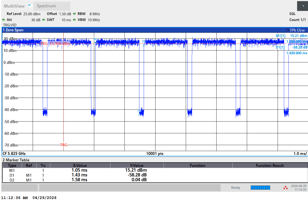
NTNV-11A-Ant1-5825
