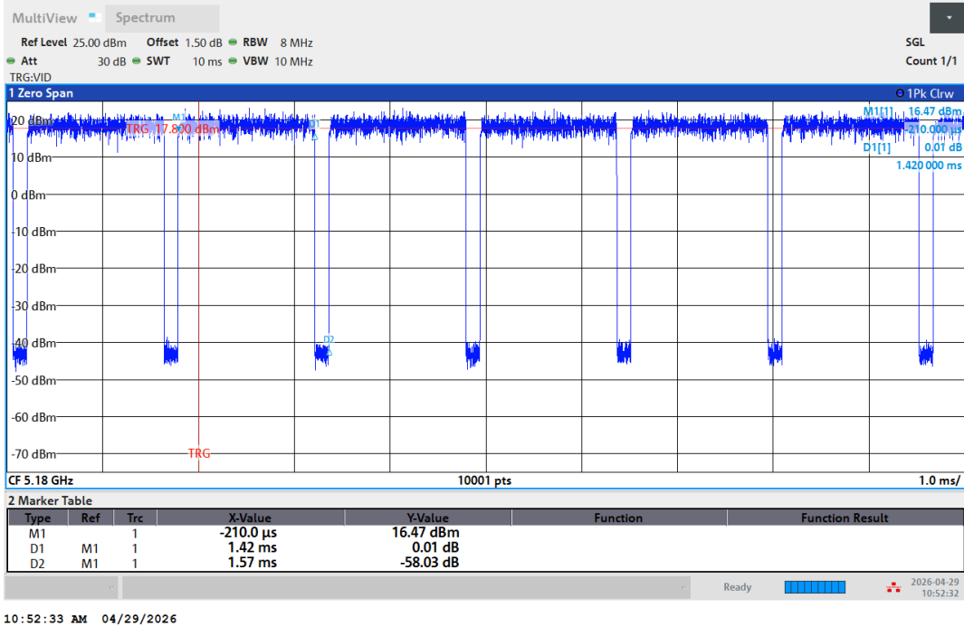
NTNV-11A-Ant1-5180
