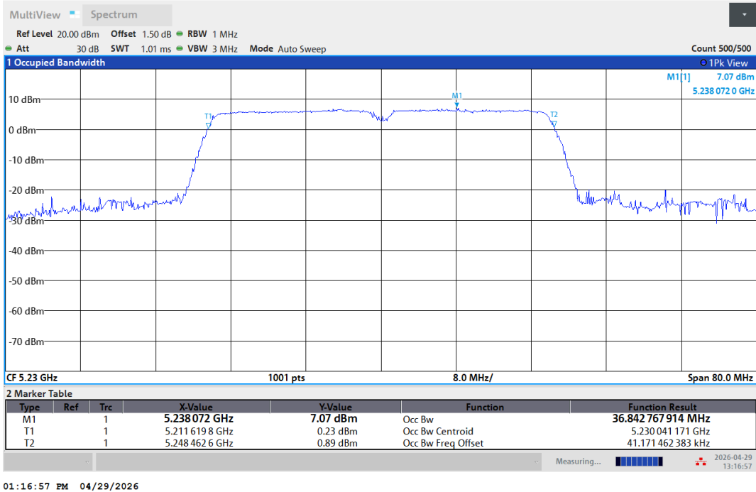
11N40SISO-Ant1-5230
