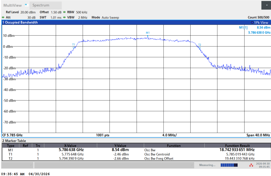
11AC20SISO-Ant1-5785
