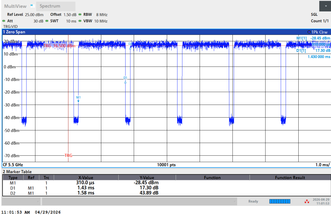
NTNV-11A-Ant1-5500
