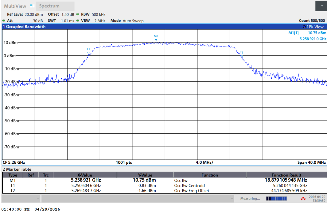
11AC20SISO-Ant1-5260
