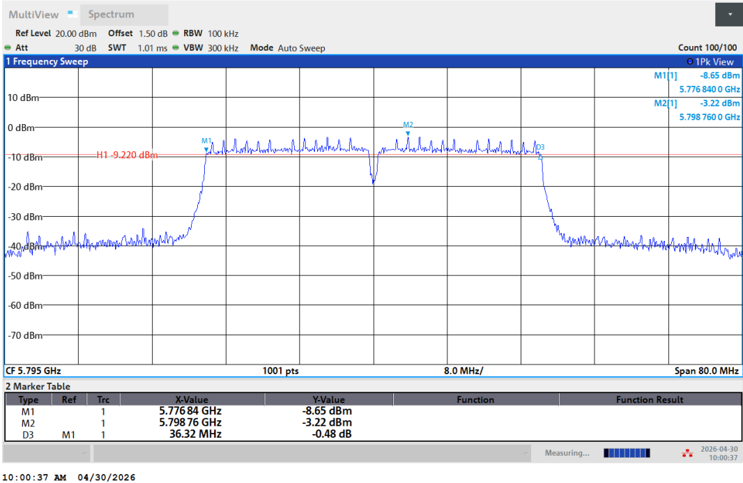
11AC40SiSO-Ant1-5795-PASS
