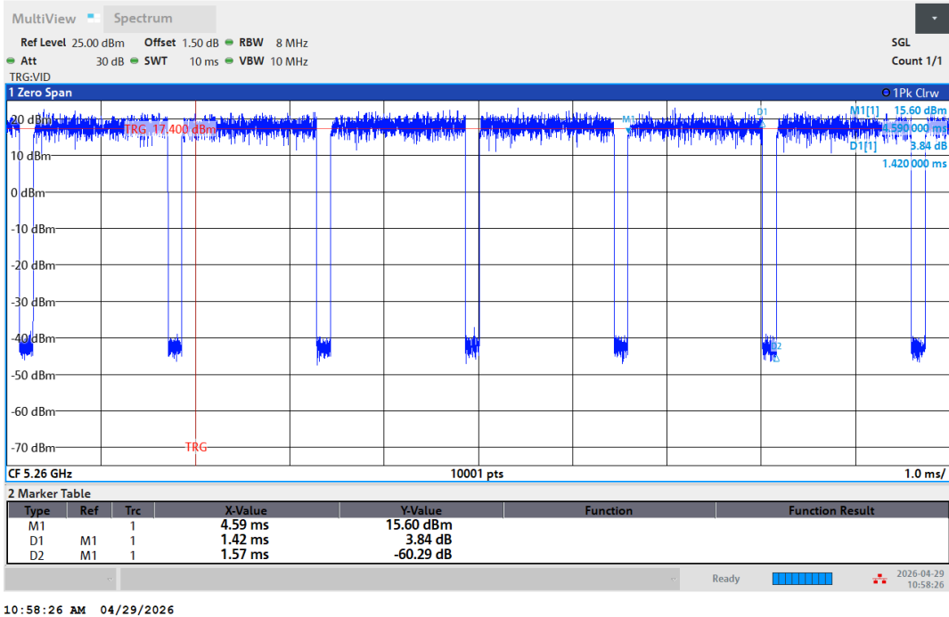
NTNV-11A-Ant1-5260
