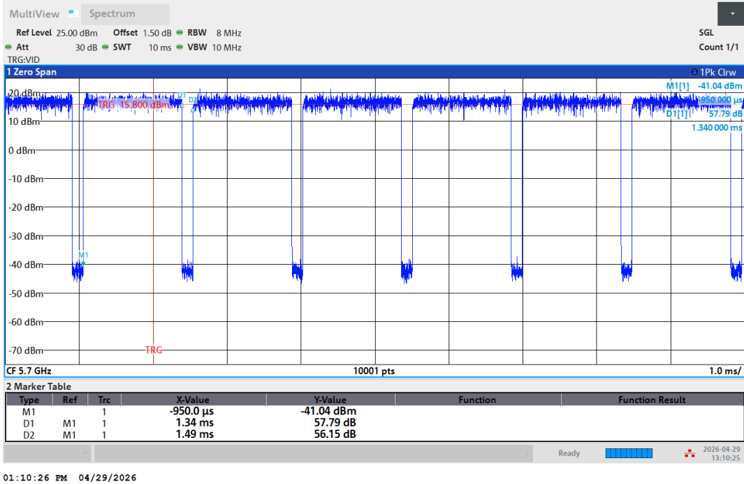
NTNV-11N20SISO-Ant1-5700
