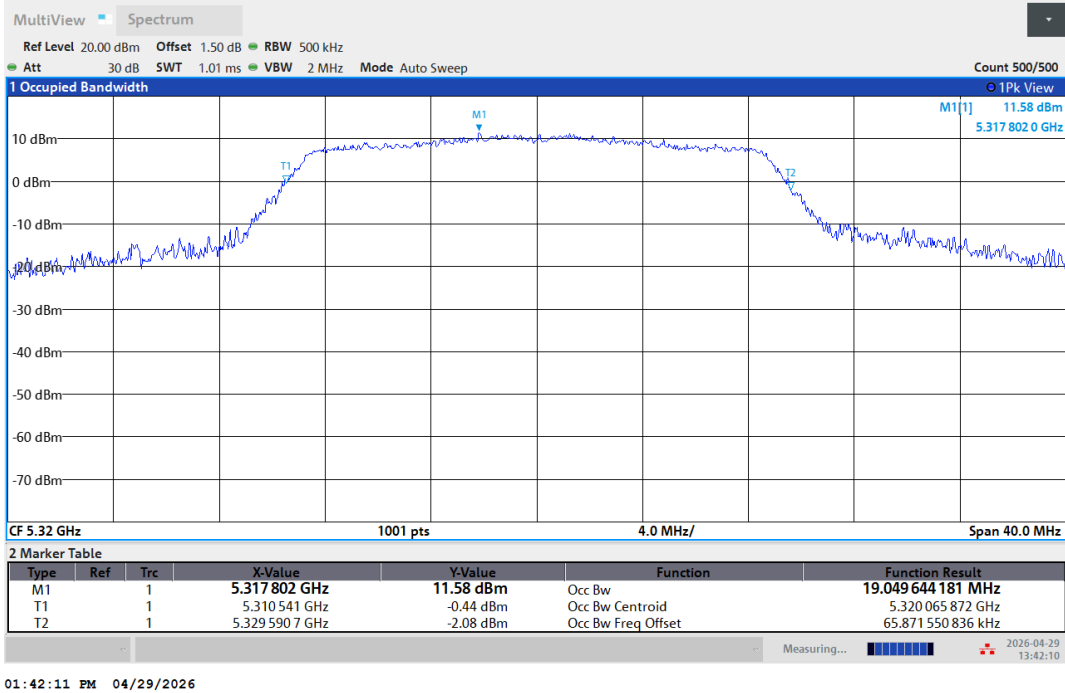
11AC20SISO-Ant1-5320
