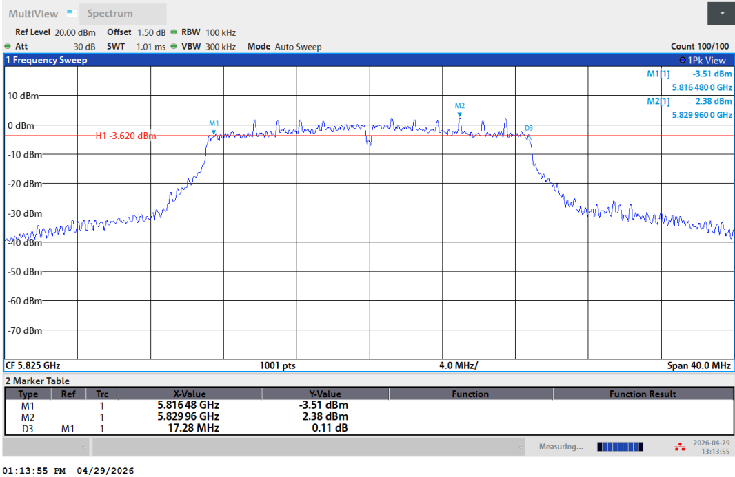
11N20SISO-Ant1-5825-PASS
