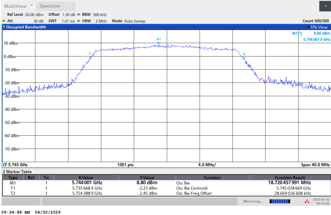
11AC20SISO-Ant1-5745
