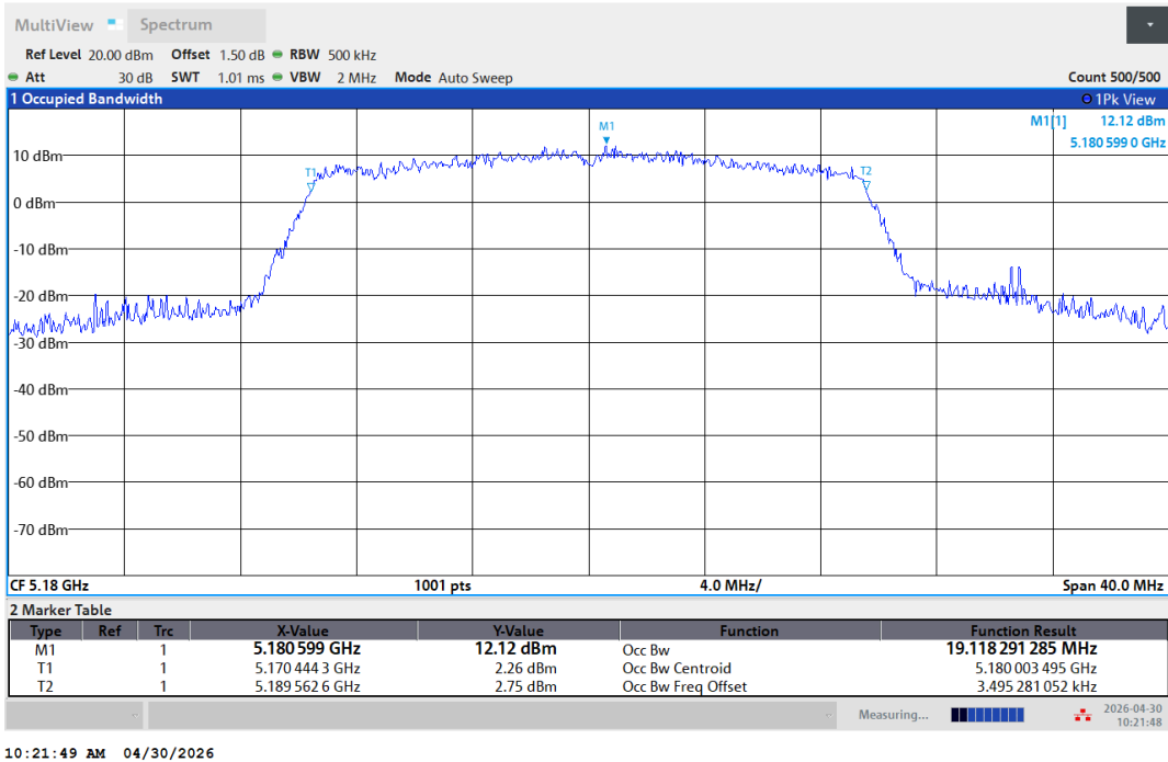
11AX20SISO-Ant1-5180
