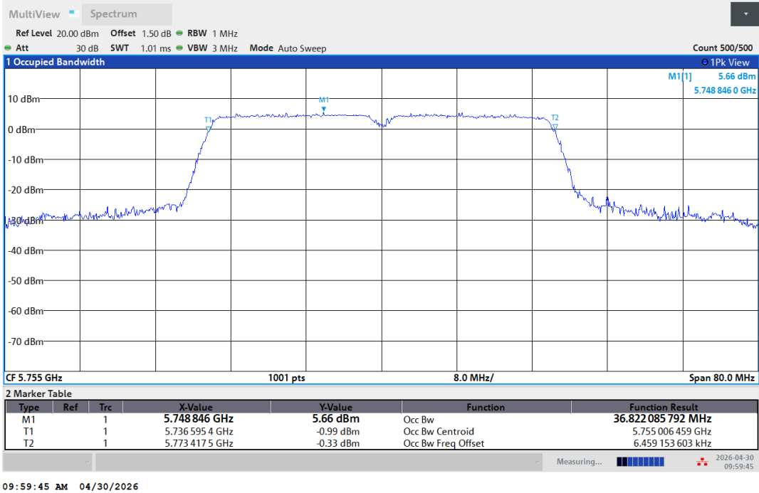
11AC40SISO-Ant1-5755
