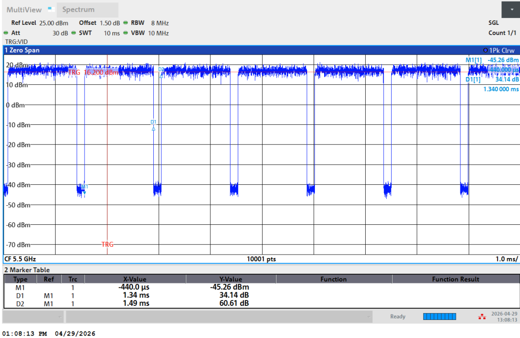
NTNV-11N20SISO-Ant1-5500
