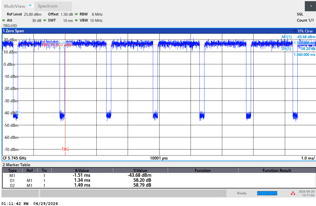
NTNV-11N20SISO-Ant1-5745
