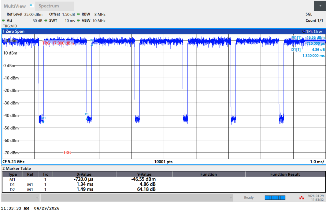
NTNV-11N20SISO-Ant1-5240
