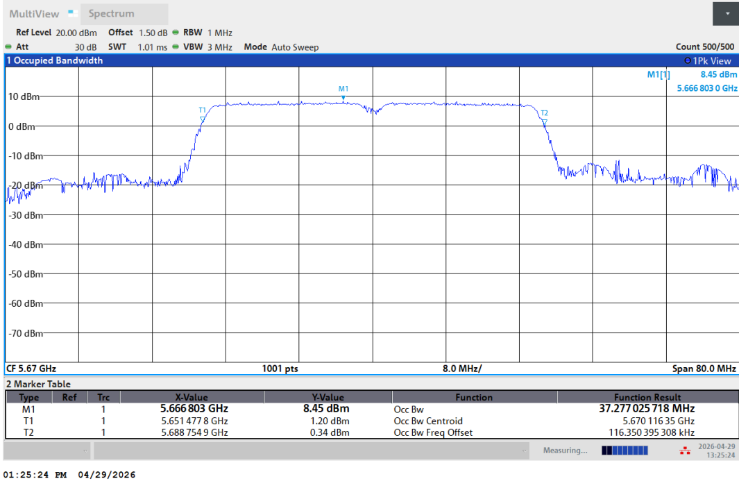
11N40SISO-Ant1-5670
