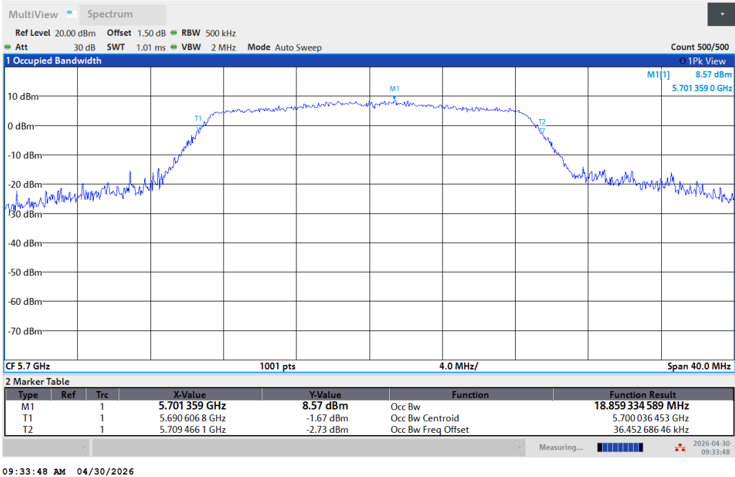
11AC20SISO-Ant1-5700
