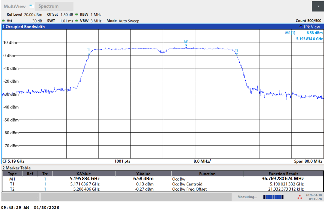
11AC40SISO-Ant1-5190
