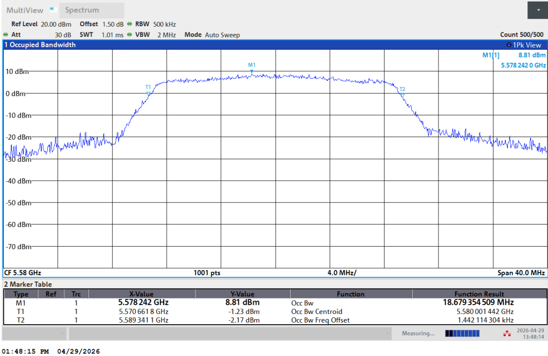
11AC20SISO-Ant1-5580
