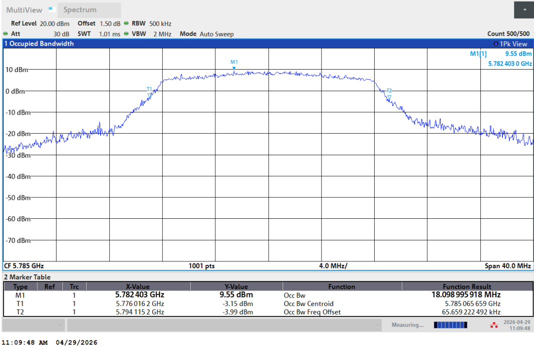
11A-Ant1-5785
