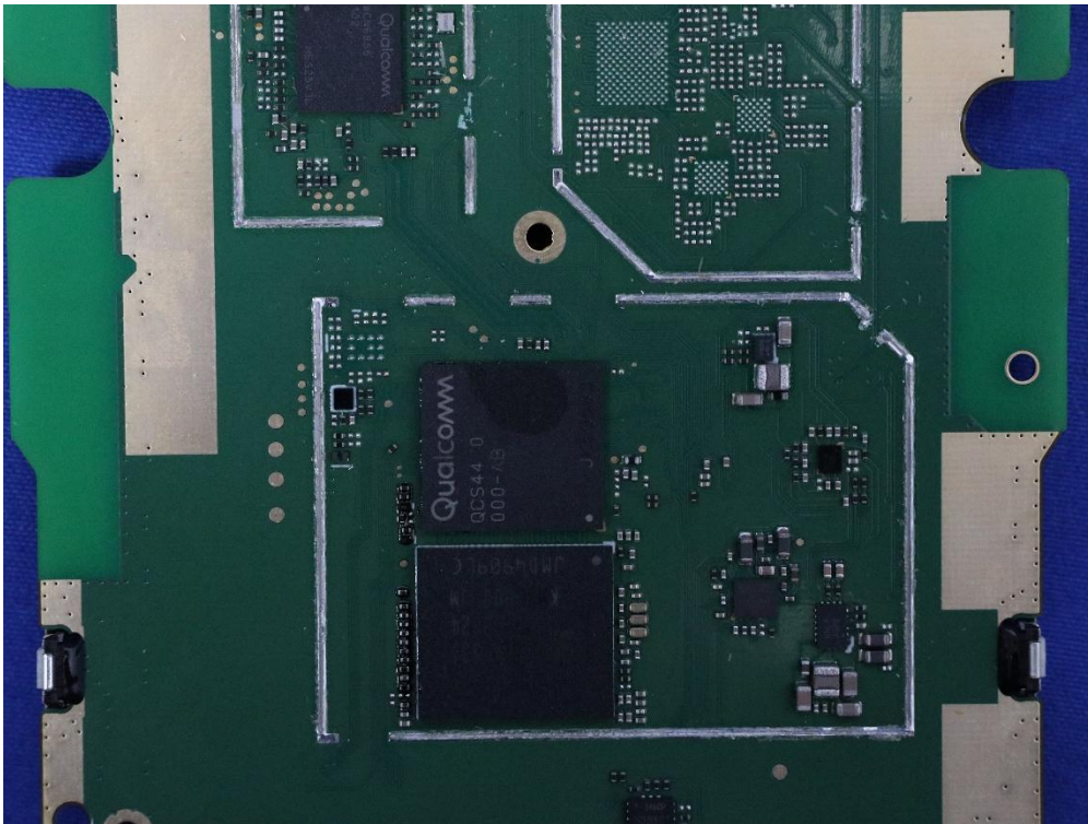
(34) EUT Photo
