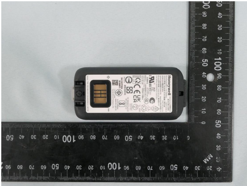
(12) EUT Photo (Brand: Honey, M/N: CK65-BTCS)
