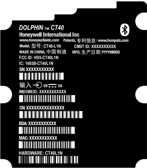
50142903-002(For WWAN)
