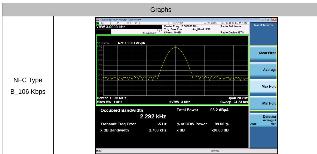
20dB Bandwidth & 99% Bandwidth Plot
