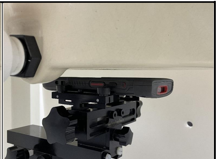
Front Face of EUT with 1.0 cm Gap
