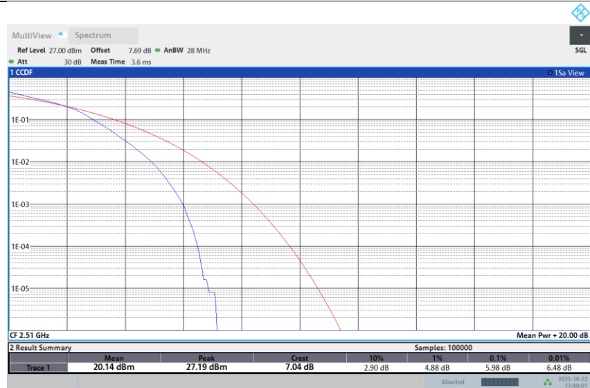
Band 7-20M-Low-64QAM-1RB Low
