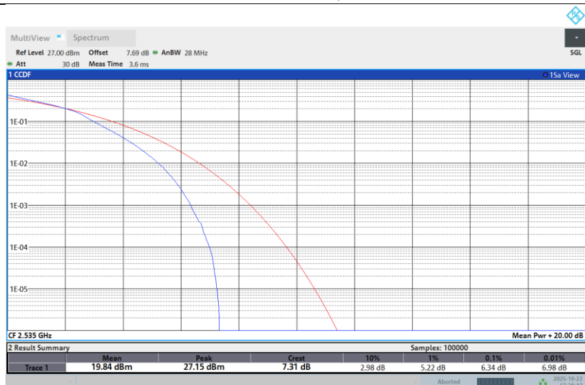
Band 7-15M-Mid-64QAM-1RB Low
