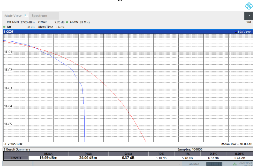
Band 7-10M-High-64QAM-Full RB
