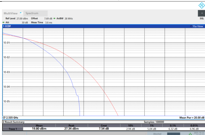
Band 7-20M-Mid-64QAM-1RB Low
