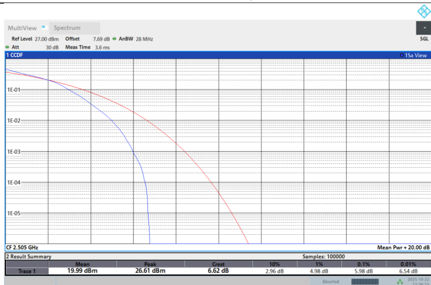
Band 7-10M-Low-64QAM-1RB Low
