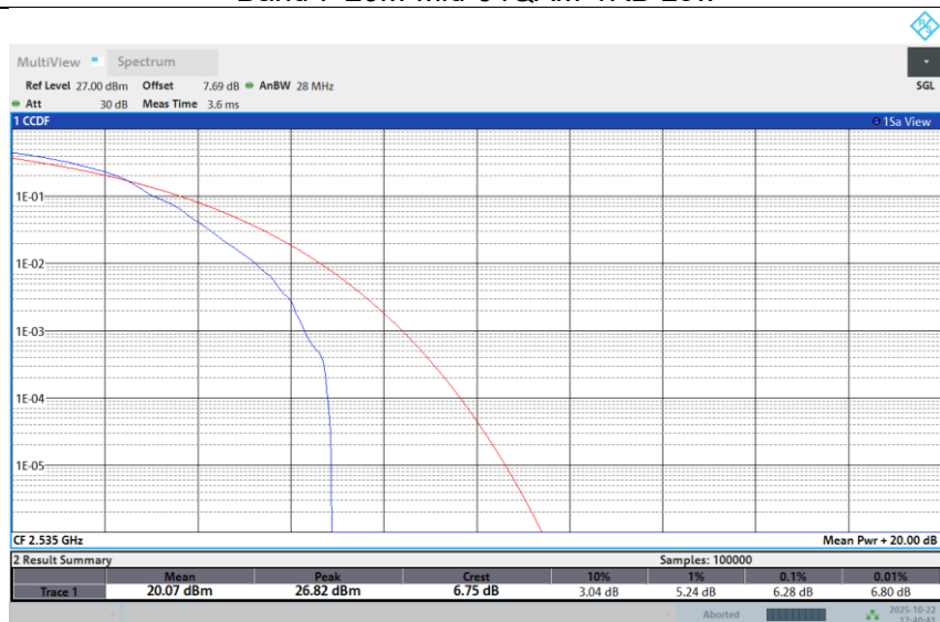
Band 7-20M-Mid-64QAM-Full RB
