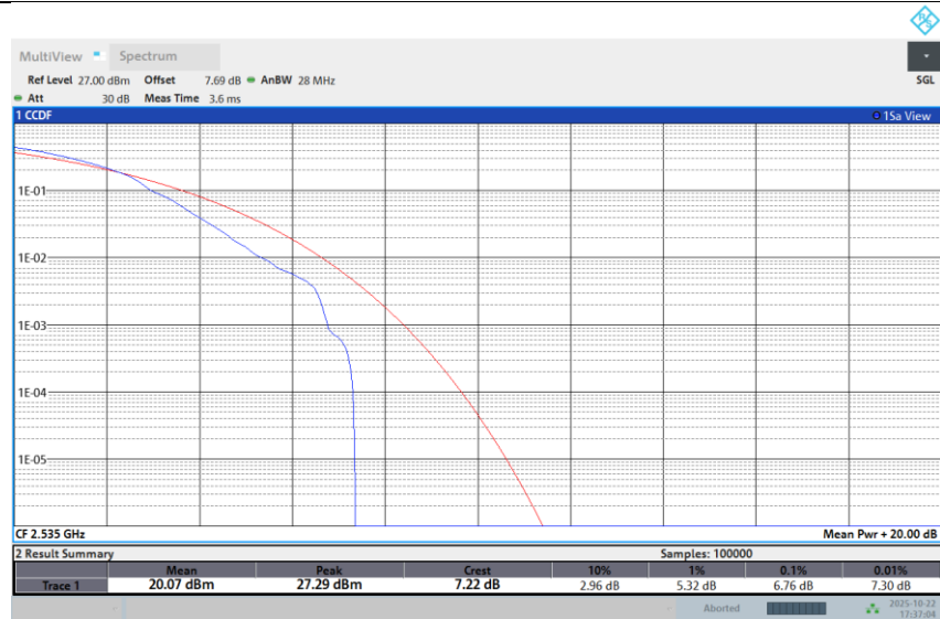
Band 7-10M-Mid-64QAM-Full RB
