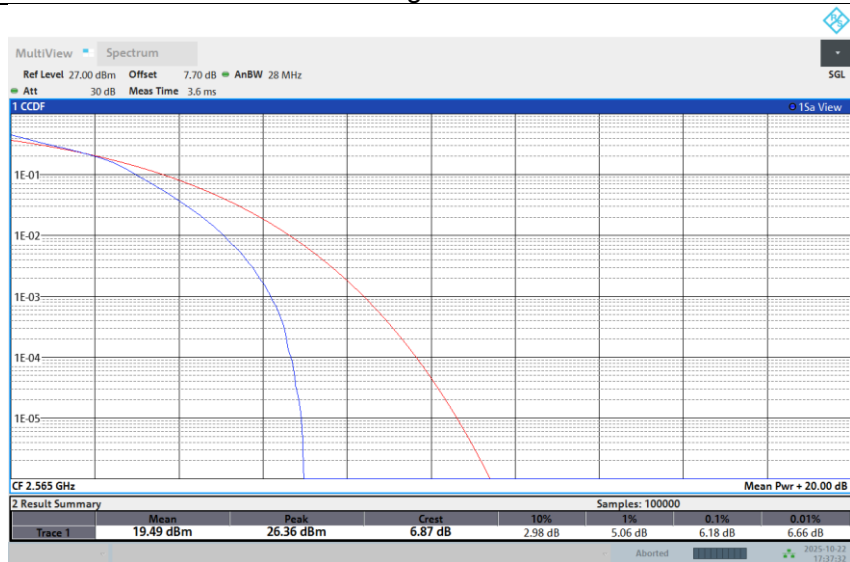
Band 7-10M-High-64QAM-1RB Low
