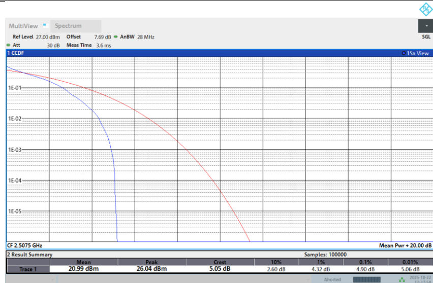
Band 7-15M-Low-QPSK-Full RB
