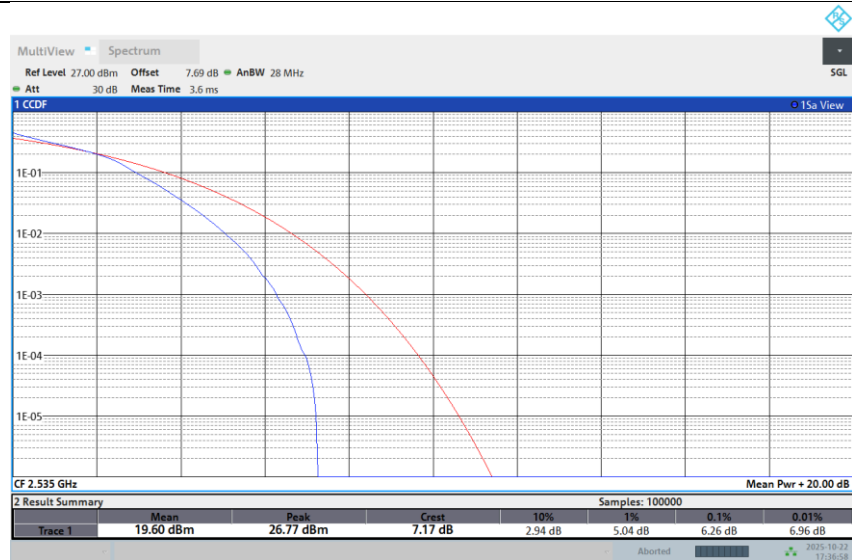
Band 7-10M-Mid-64QAM-1RB Low
