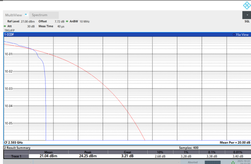
Band 41-5M-MID-16QAM-Full RB
