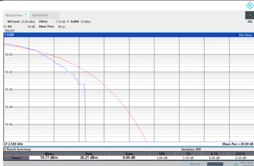
Band 41-5M-MID-64QAM-1RB Low
