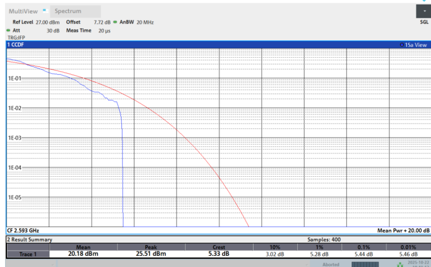
Band 41-15M-MID-64QAM-1RB Low
