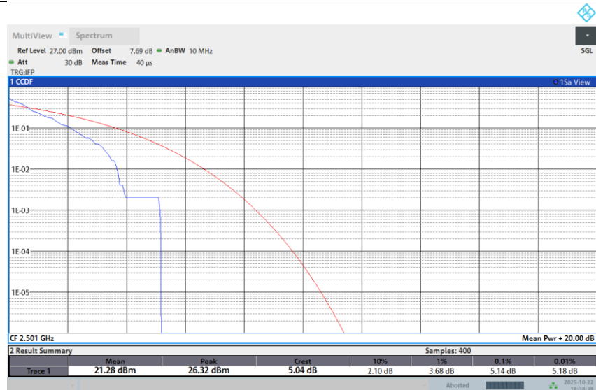
Band 41-10M-LOW-16QAM-1RB Low
