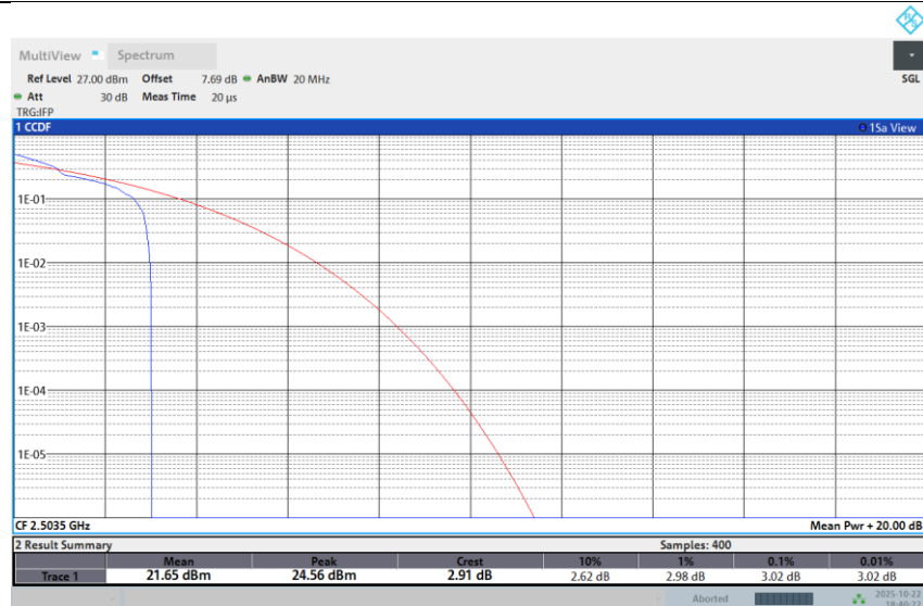
Band 41-15M-LOW-QPSK-Full RB
