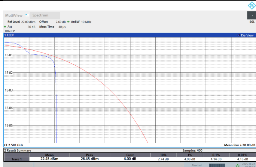
Band 41-10M-LOW-16QAM-Full RB
