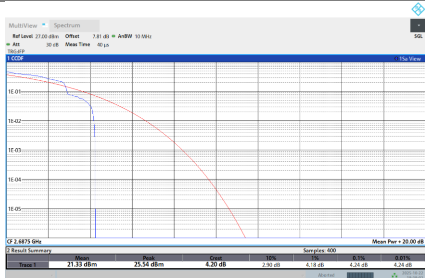
Band 41-5M-HIGH-16QAM-Full RB
