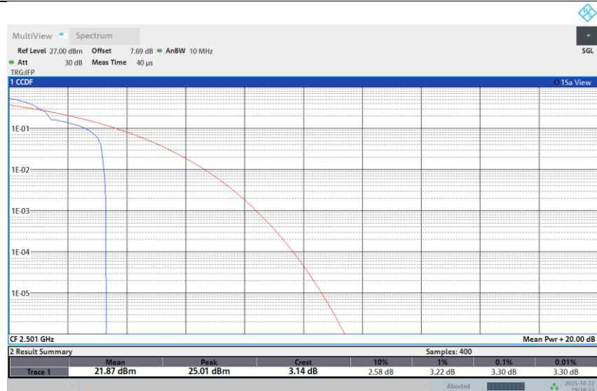
Band 41-10M-LOW-QPSK-Full RB
