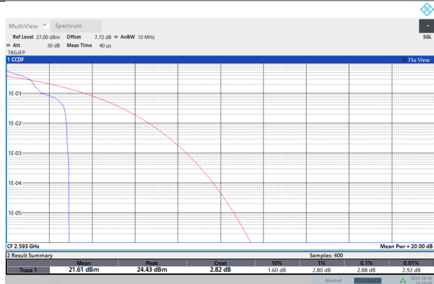
Band 41-10M-MID-QPSK-Full RB
