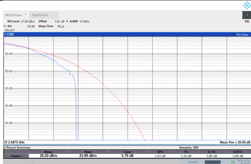
Band 41-5M-HIGH-64QAM-1RB Low
