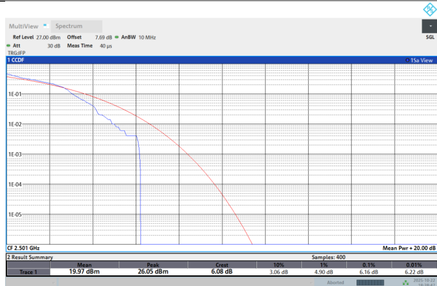
Band 41-10M-LOW-64QAM-1RB Low
