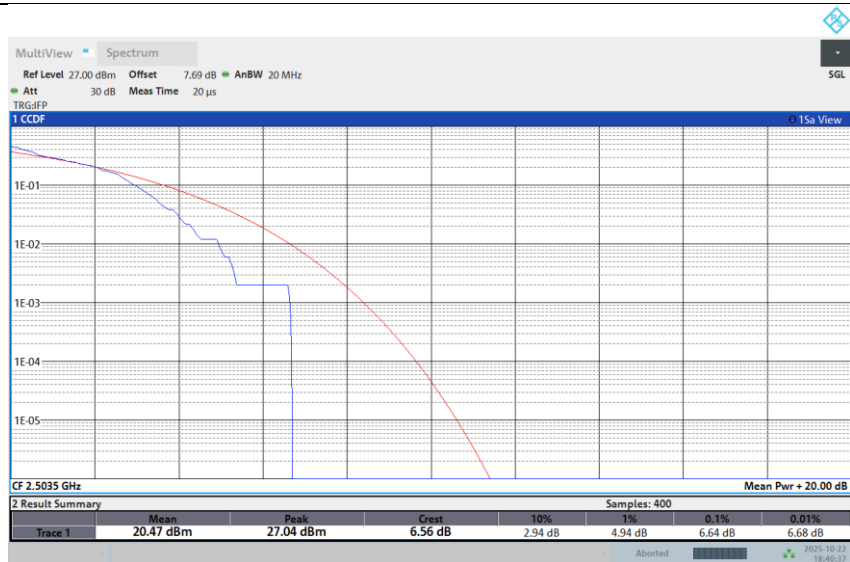
Band 41-15M-LOW-64QAM-1RB Low
