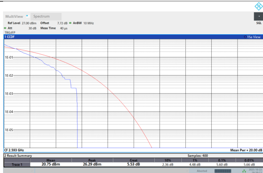
Band 41-10M-MID-16QAM-1RB Low
