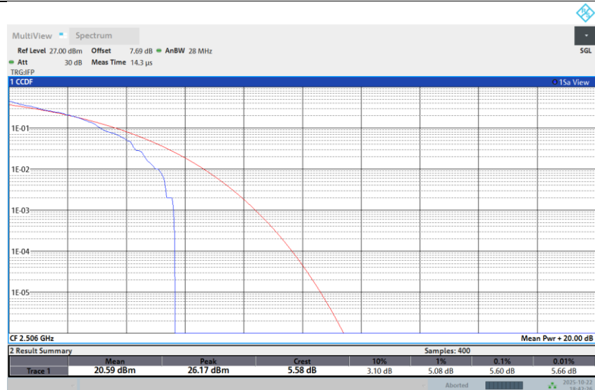
Band 41-20M-LOW-64QAM-1RB Low
