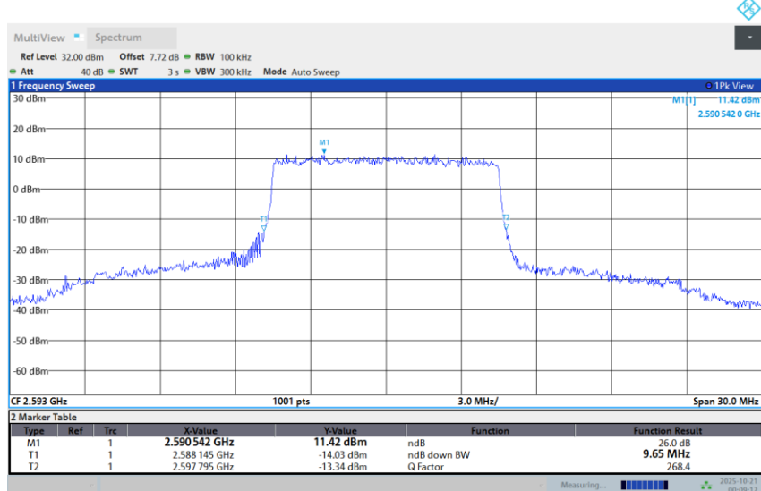
Band 41-10M-MID-64QAM-Full RB
