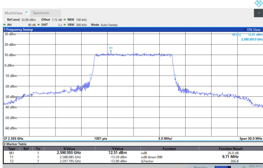
Band 41-10M-MID-16QAM-Full RB
