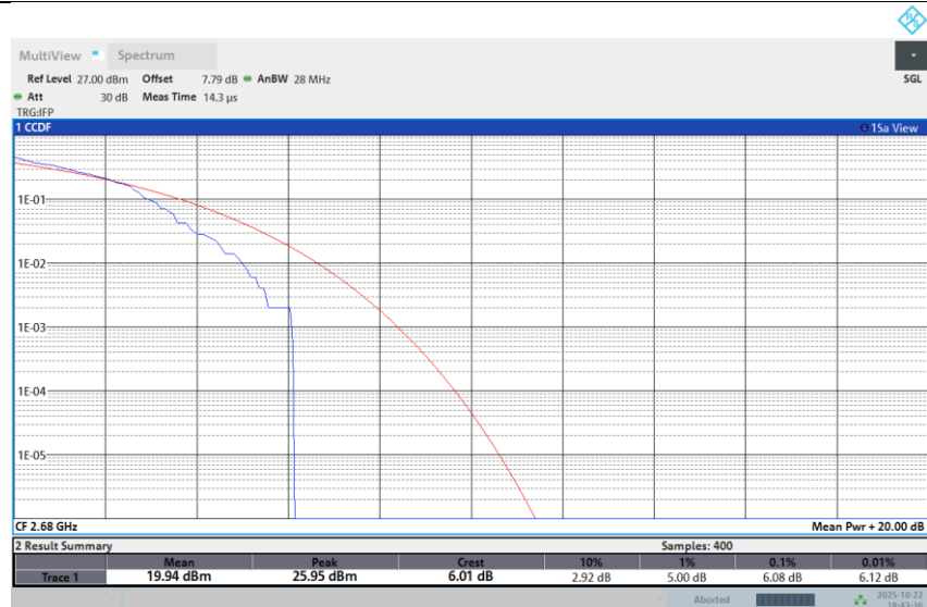
Band 41-20M-HIGH-64QAM-1RB Low
