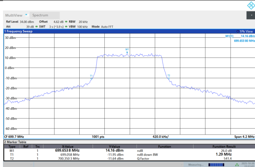
Band 12-1.4M-LOW-16QAM-Full RB
