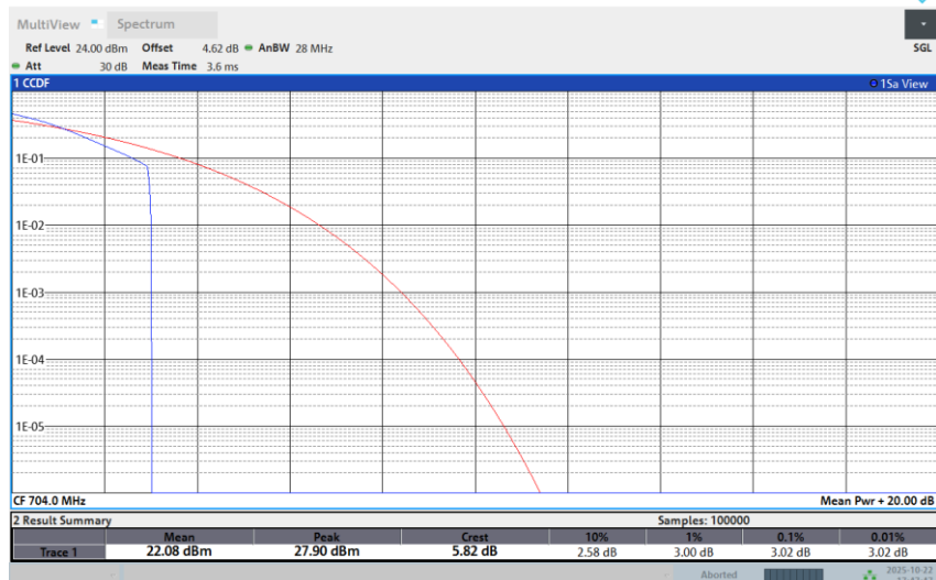
Band 12-10M-LOW-16QAM-1RB Low
