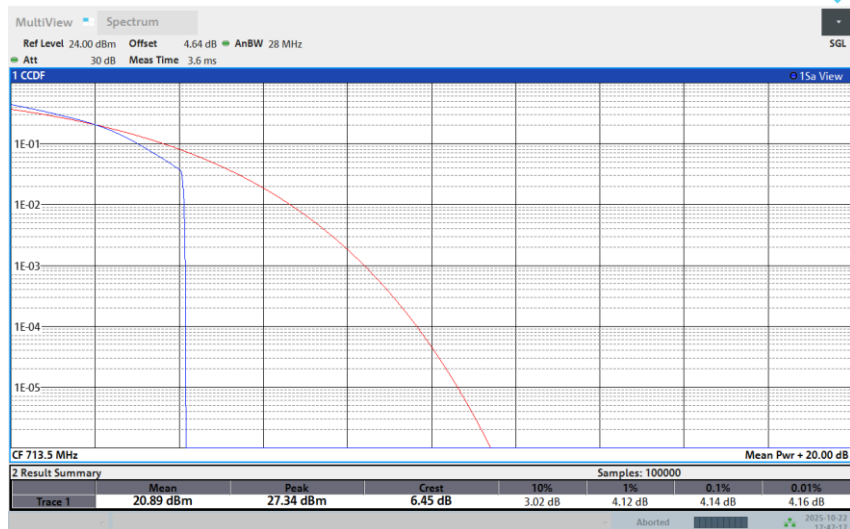
Band 12-5M-HIGH-64QAM-1RB Low
