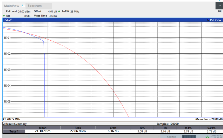
Band 12-10M-MID-64QAM-1RB Low
