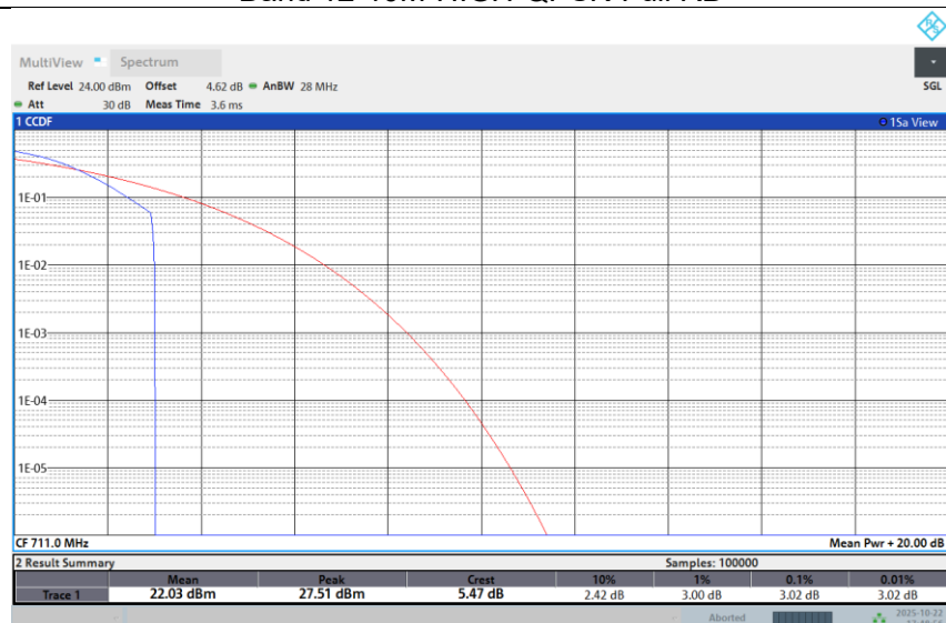
Band 12-10M-HIGH-16QAM-1RB Low
