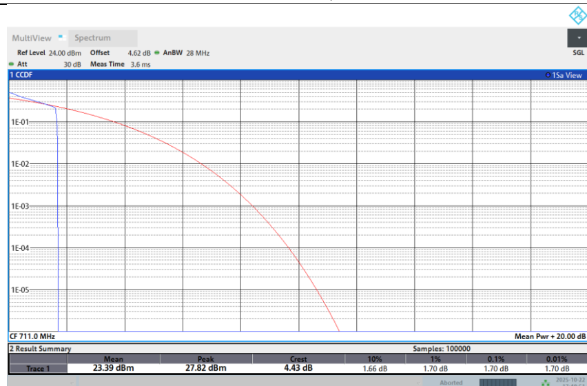
Band 12-10M-HIGH-QPSK-Full RB
