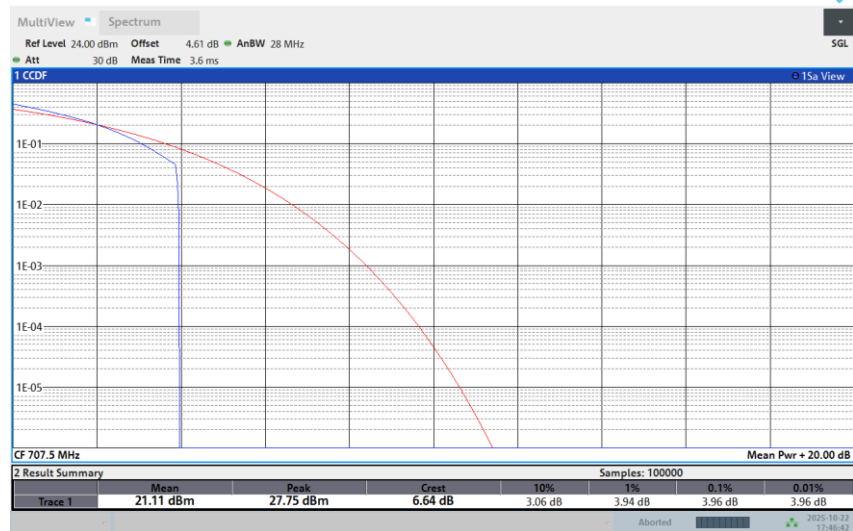
Band 12-5M-MID-64QAM-1RB Low
