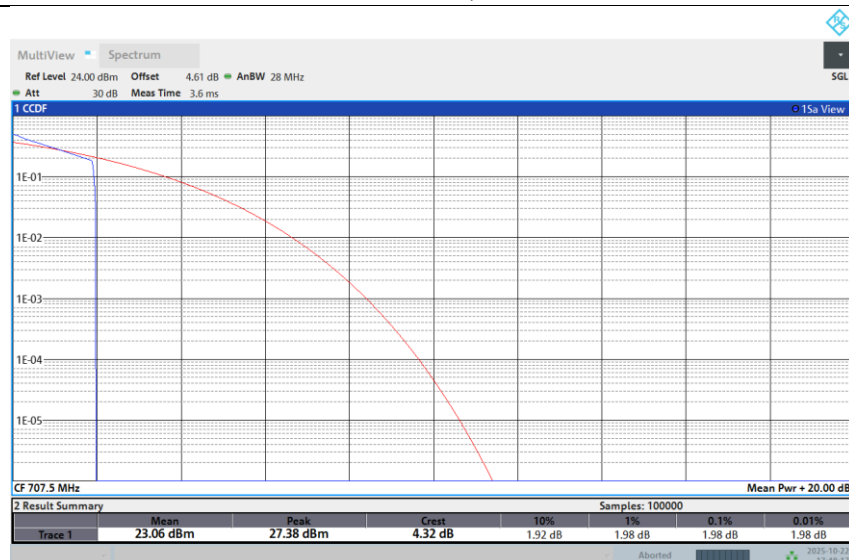
Band 12-10M-MID-QPSK-Full RB
