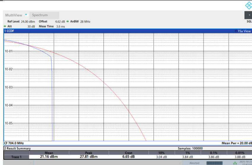
Band 12-10M-LOW-64QAM-1RB Low
