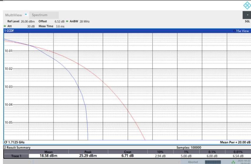
Band 66-5M-LOW-64QAM-1RB Low
