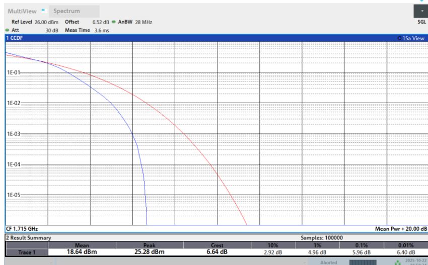
Band 66-10M-LOW-64QAM-1RB Low
