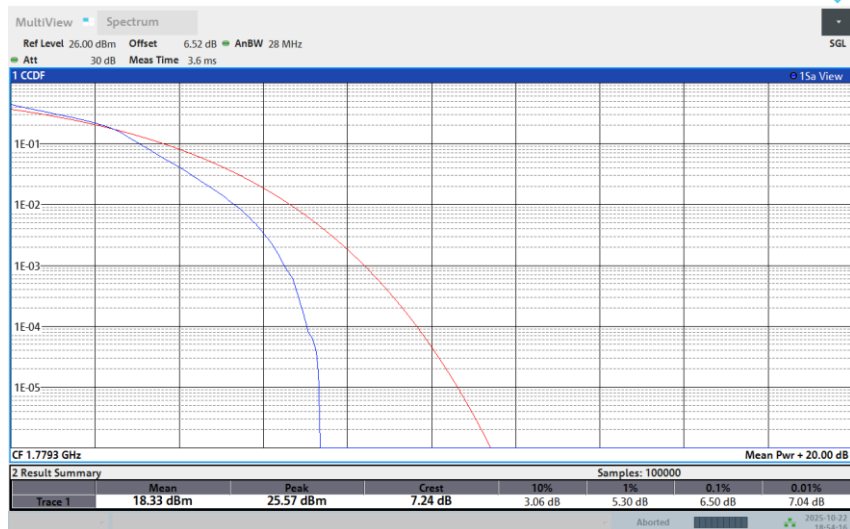
Band 66-1.4M-HIGH-64QAM-1RB Low
