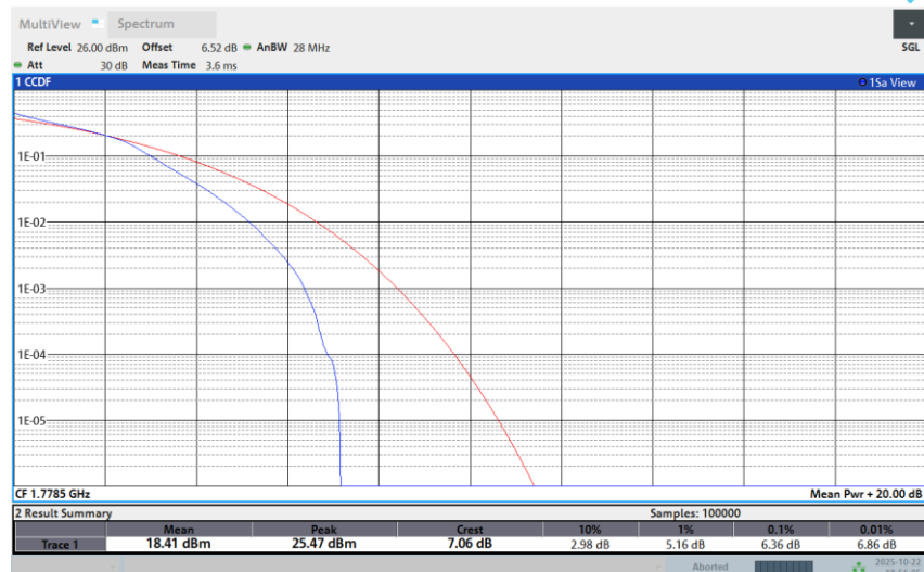
Band 66-3M-HIGH-64QAM-1RB Low
