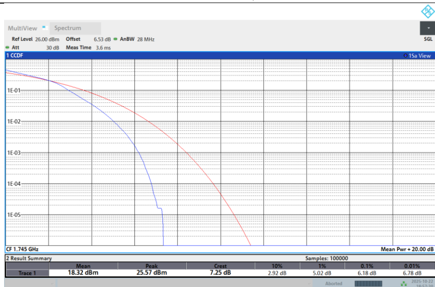
Band 66-5M-MID-64QAM-1RB Low
