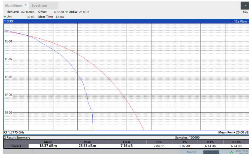
Band 66-5M-HIGH-64QAM-1RB Low
