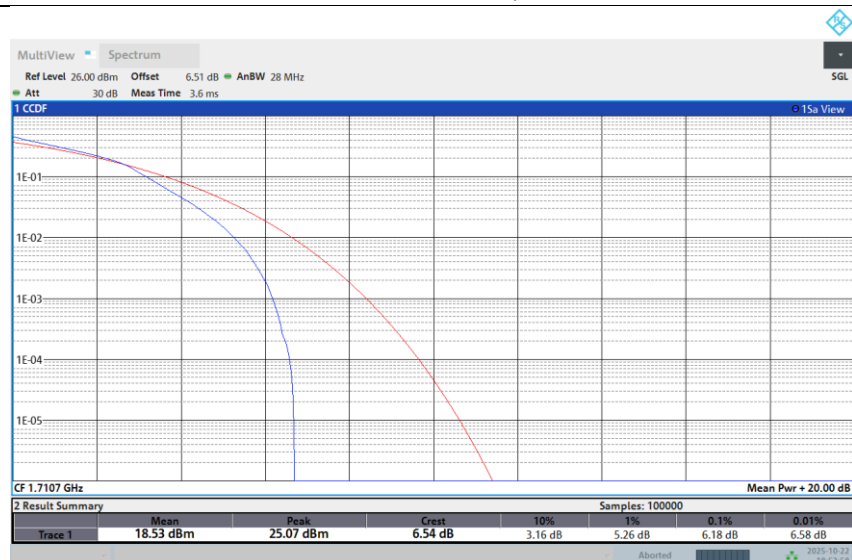
Band 66-1.4M-LOW-64QAM-1RB Low
