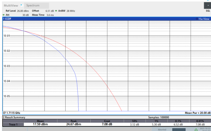
Band 66-3M-MID-QPSK-1RB Low
