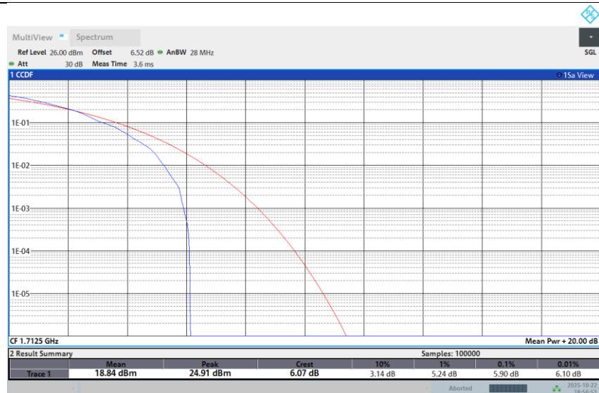
Band 66-5M-LOW-64QAM-Full RB
