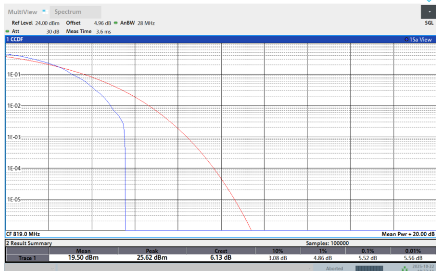
Band 26-10M-LOW-64QAM-Full RB
