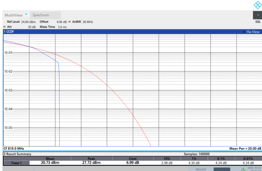
Band 26-5M-MID-64QAM-1RB Low
