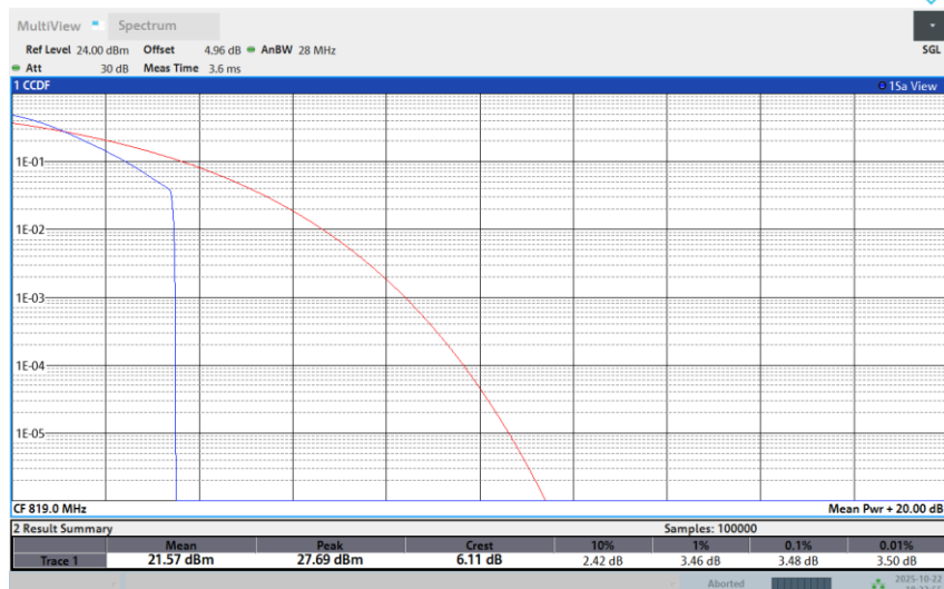
Band 26-10M-LOW-16QAM-1RB Low
