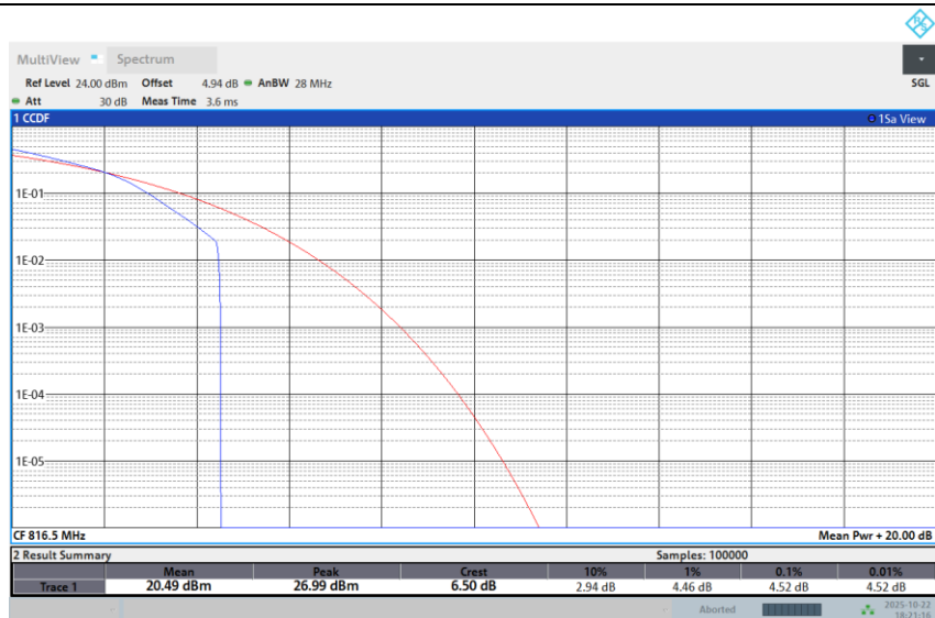
Band 26-5M-LOW-64QAM-1RB Low
