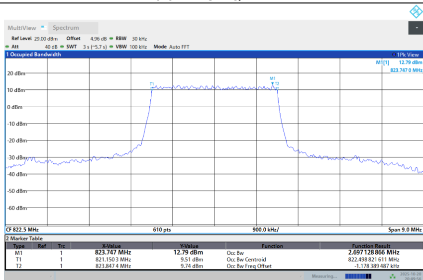
Band 26-3M-HIGH-16QAM-Full RB
