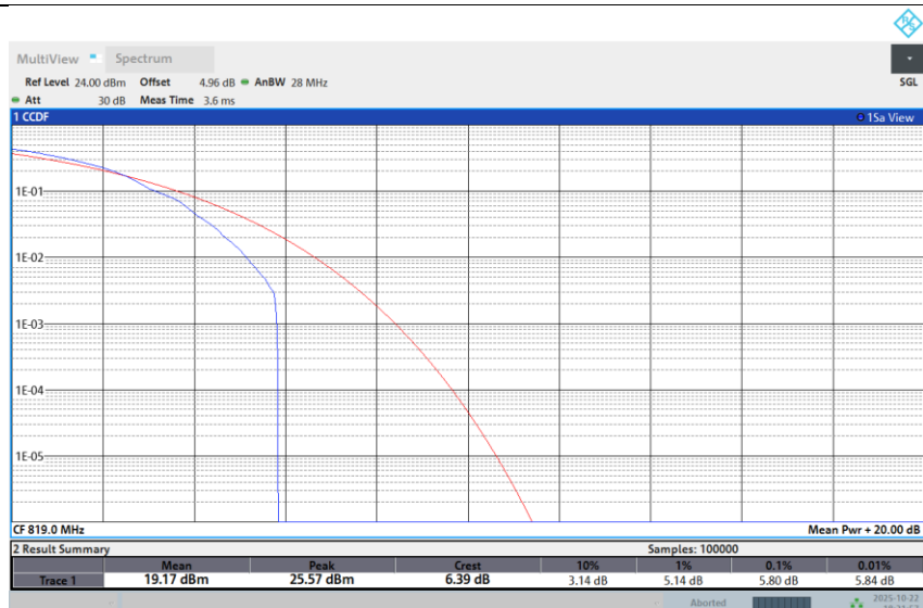
Band 26-5M-MID-64QAM-Full RB
