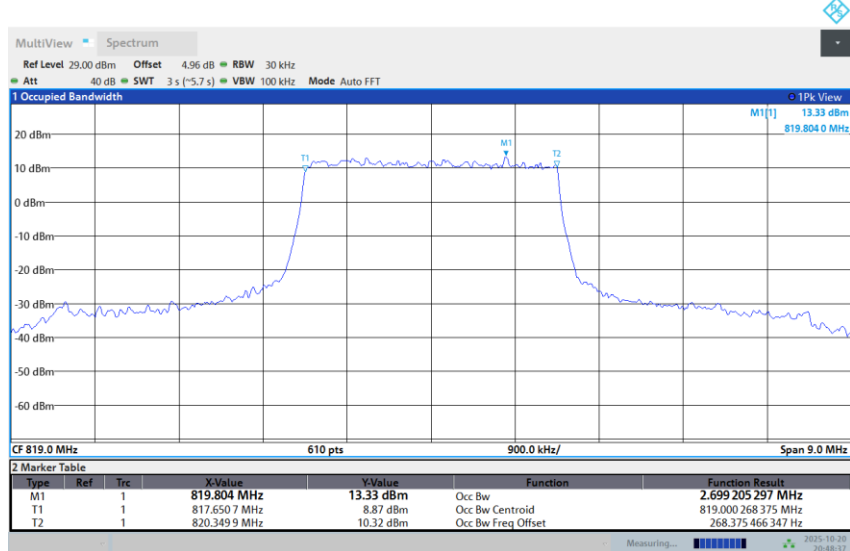
Band 26-3M-MID-16QAM-Full RB
