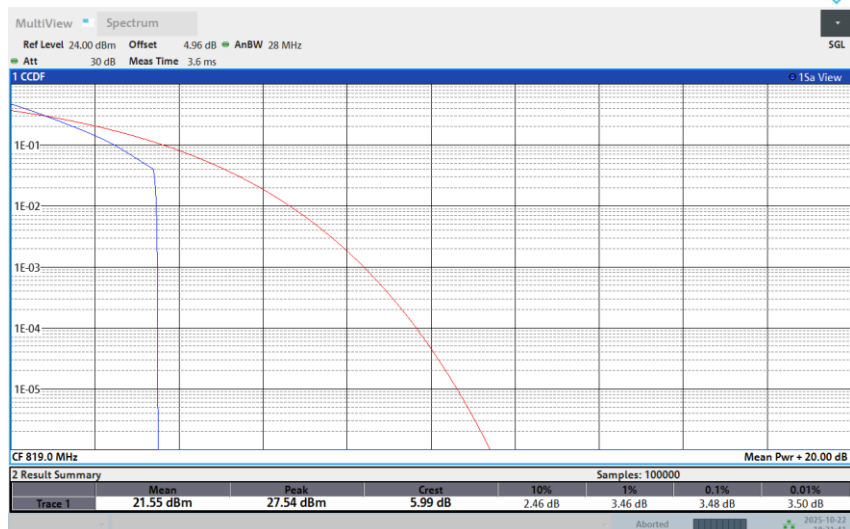
Band 26-5M-MID-16QAM-1RB Low
