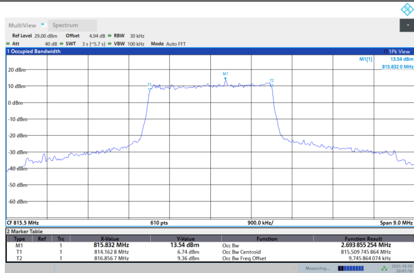
Band 26-3M-LOW-16QAM-Full RB
