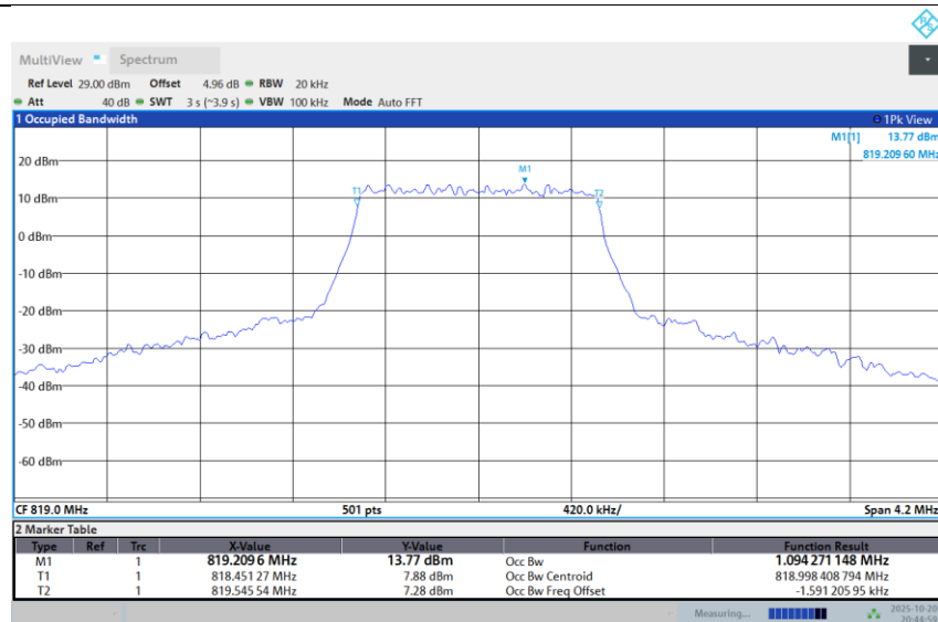
Band 26-1.4M-MID-64QAM-Full RB
