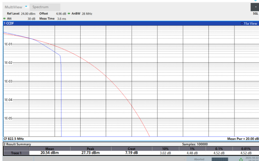
Band 26-3M-HIGH-64QAM-1RB Low
