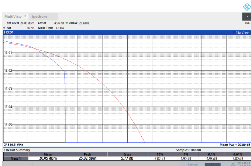
Band 26-5M-LOW-16QAM-Full RB
