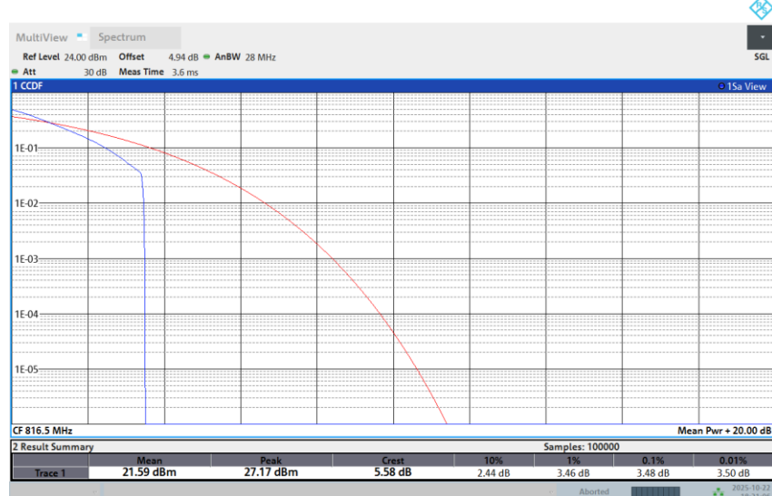
Band 26-5M-LOW-16QAM-1RB Low
