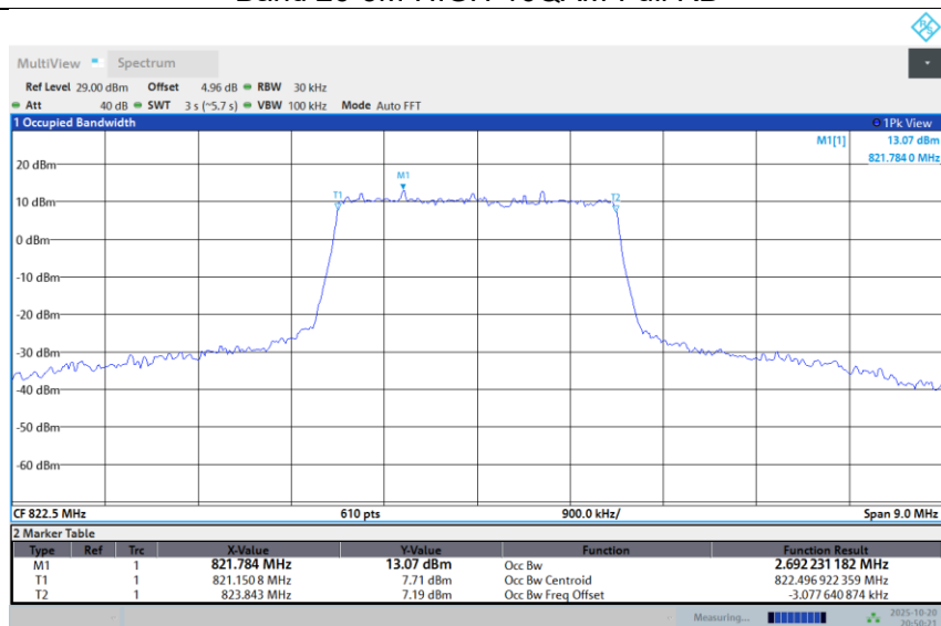
Band 26-3M-HIGH-64QAM-Full RB
