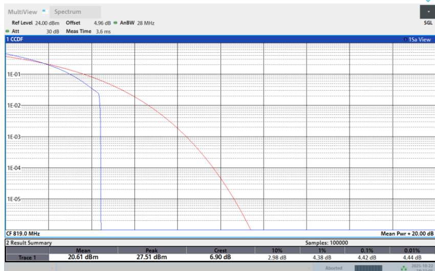
Band 26-10M-LOW-64QAM-1RB Low
