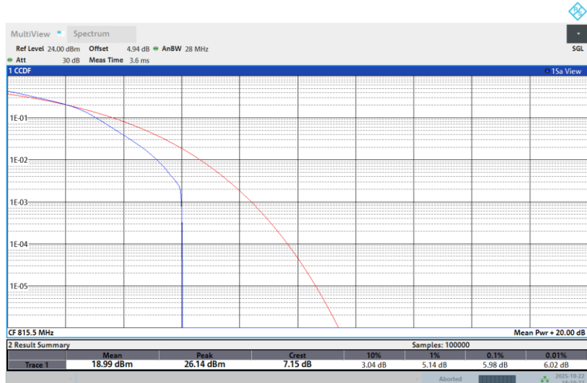
Band 26-3M-LOW-64QAM-1RB Low
