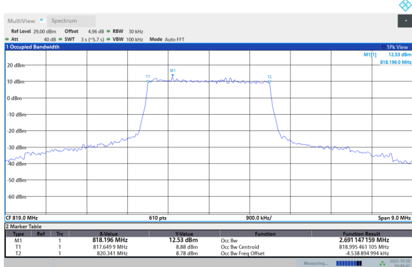
Band 26-3M-MID-64QAM-Full RB
