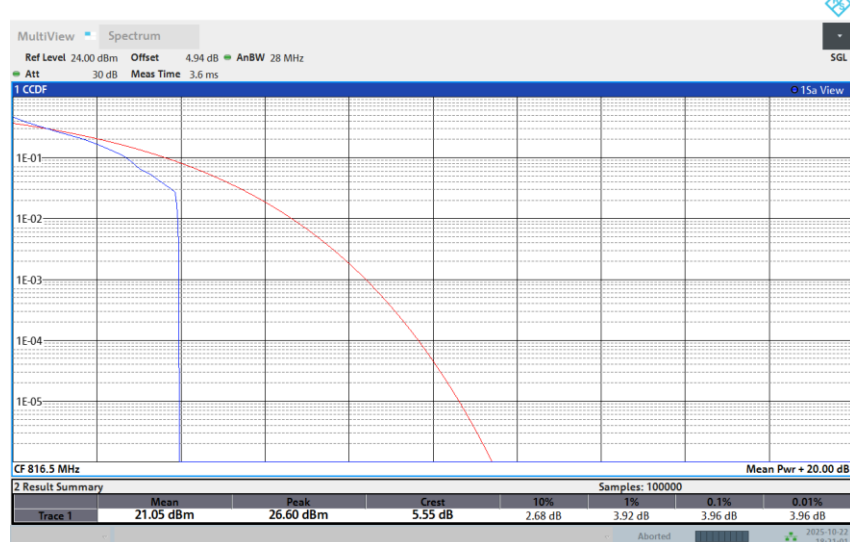
Band 26-5M-LOW-QPSK-Full RB
