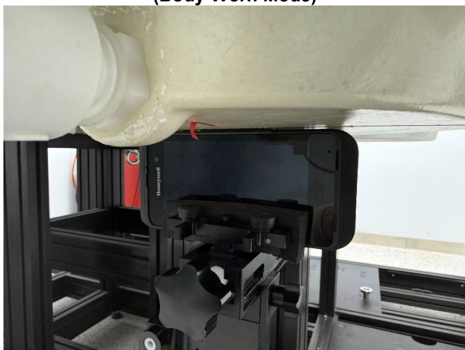
Right Side of EUT with 0 cm Gap (Limbs Mode)
