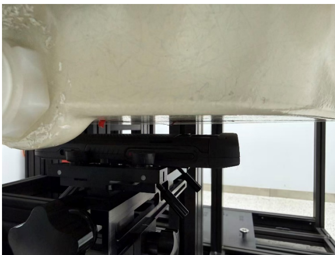
Rear Face of EUT with 1 cm Gap (Body-Worn Mode)
