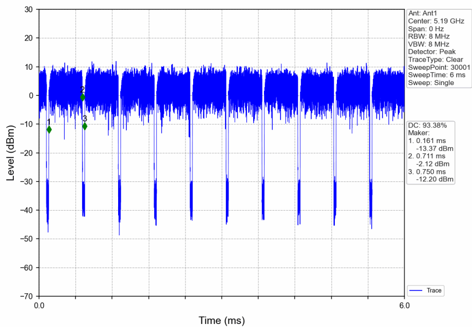
802.11ax(HEW40)_LCH_5190MHz_Ant1_NTNV
