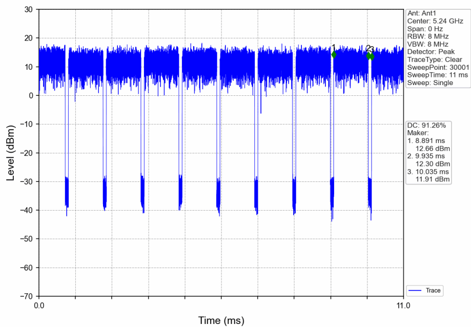
802.11ax(HEW20)_HCH_5240MHz_Ant1_NTNV
