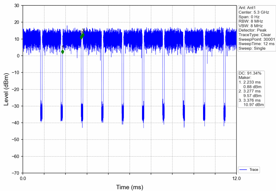
802.11ax(HEW20)_MCH_5300MHz_Ant1_NTNV
