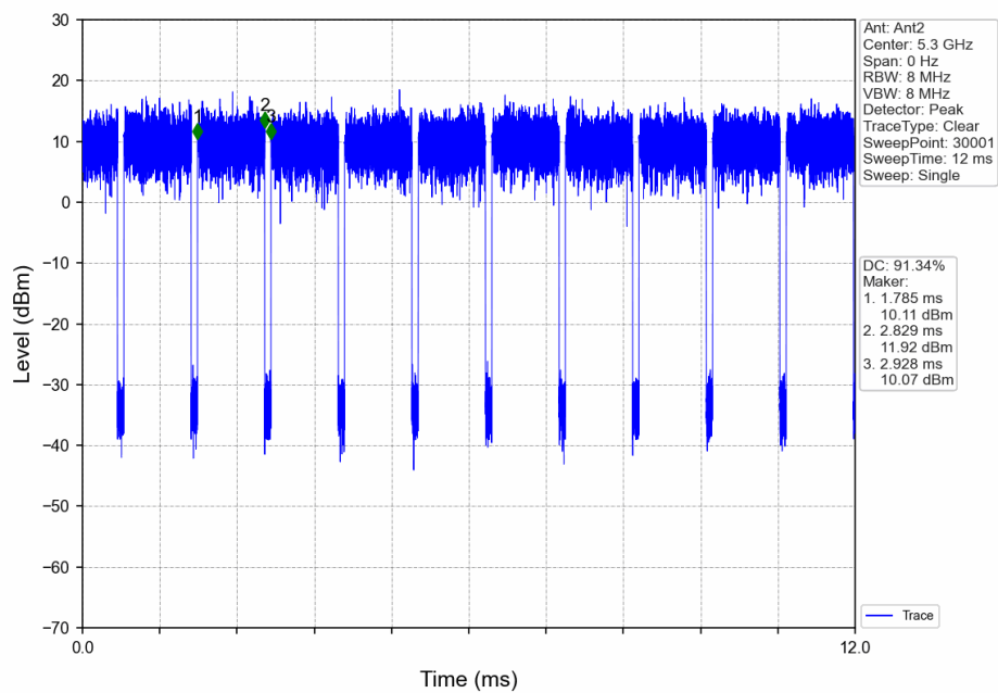
802.11ax(HEW20)_MCH_5300MHz_Ant2_NTNV
