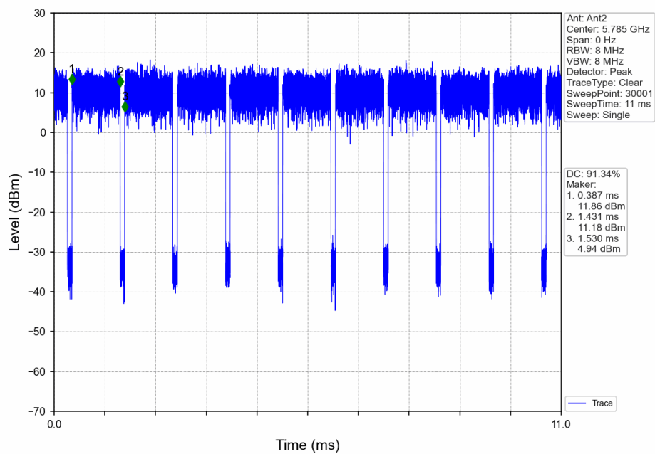
802.11ax(HEW20)_MCH_5785MHz_Ant2_NTNV
