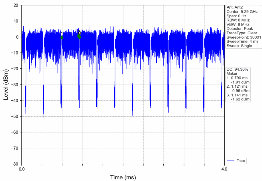
802.11ac(VHT80)_MCH_5290MHz_Ant2_NTNV
