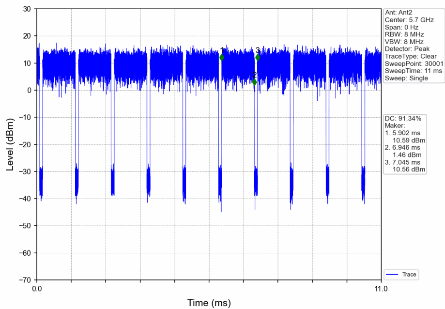
802.11ax(HEW20)_HCH_5700MHz_Ant2_NTNV
