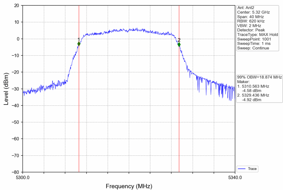
802.11ac(VHT20)_HCH_5320MHz_Ant2_NTNV
