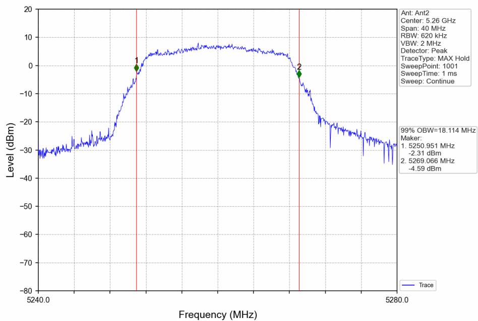
802.11a_LCH_5260MHz_Ant2_NTNV
