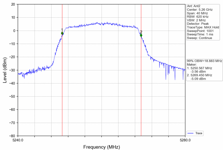
802.11ac(VHT20)_LCH_5260MHz_Ant2_NTNV
