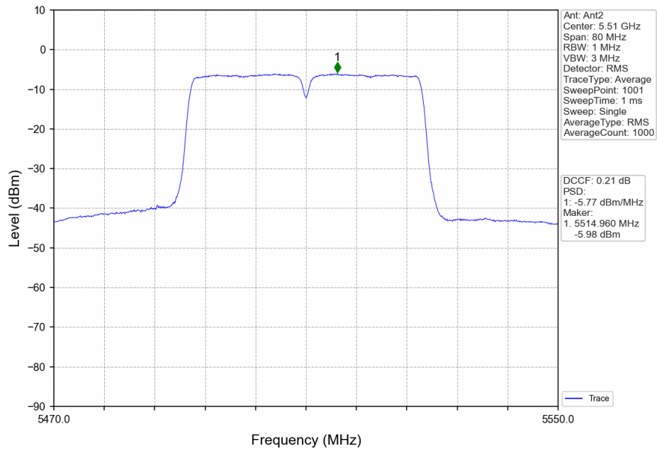
802.11ac(VHT40)_LCH_5510MHz_MIMO_NTNV
