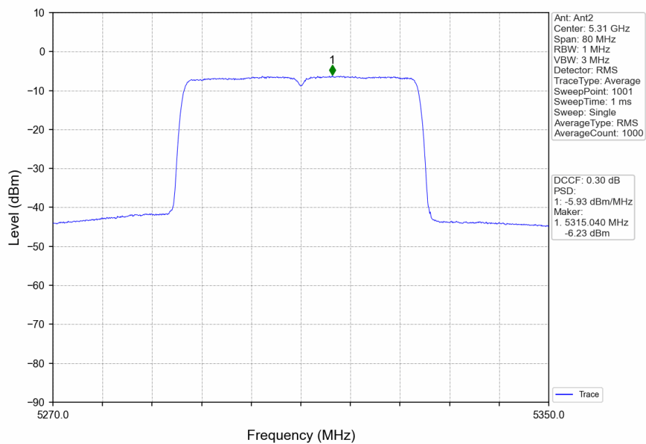
802.11ax(HEW40)_HCH_5310MHz_Ant2_NTNV
