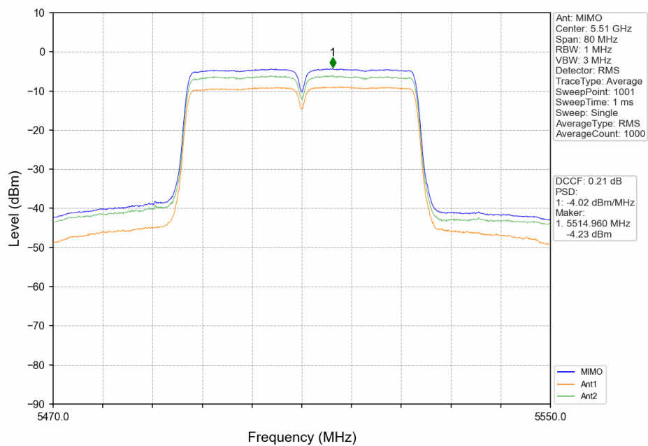
802.11ac(VHT40)_LCH_5510MHz_MIMO_NTNV
