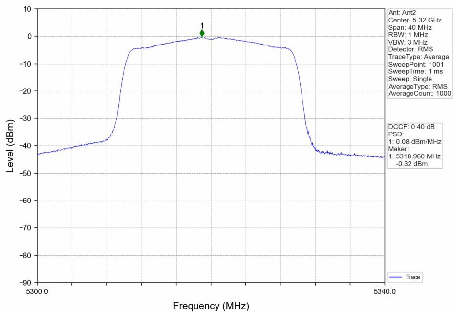
802.11ax(HEW20)_HCH_5320MHz_Ant2_NTNV
