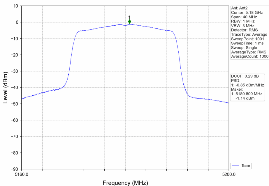
802.11ax(HEW20)_LCH_5180MHz_Ant2_NTNV
