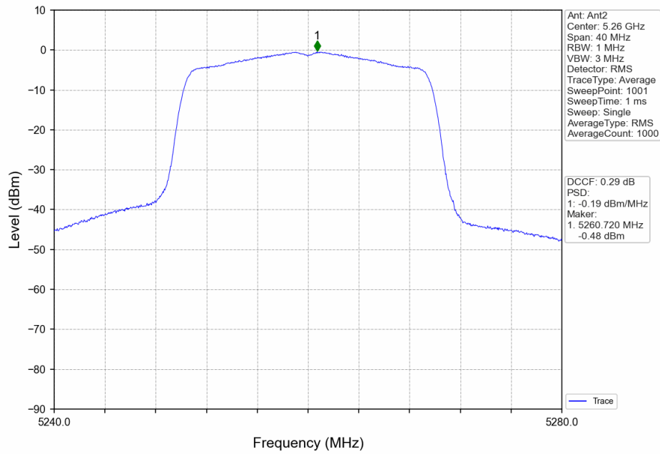
802.11ax(HEW20)_LCH_5260MHz_MIMO_NTNV
