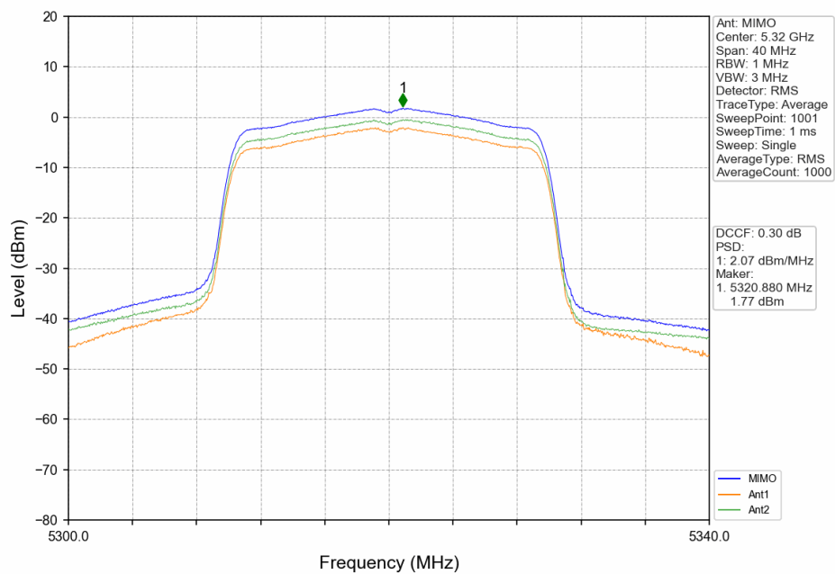
802.11ax(HEW20)_HCH_5320MHz_MIMO_NTNV
