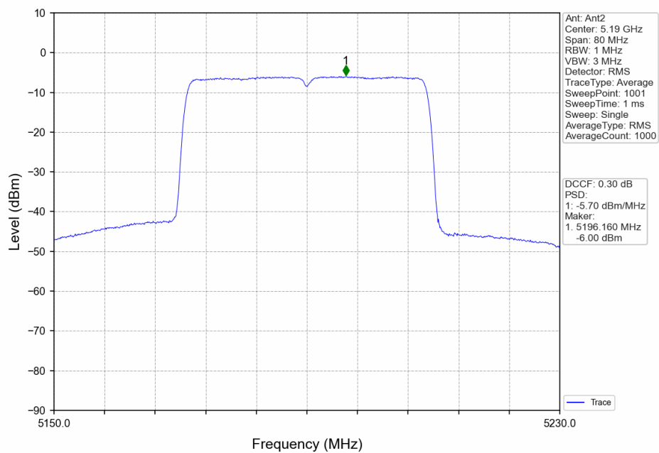
802.11ax(HEW40)_LCH_5190MHz_Ant2_NTNV
