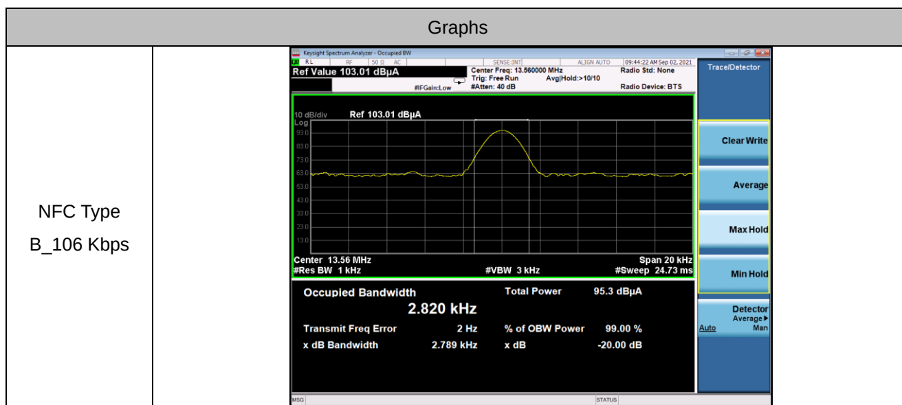
20dB Bandwidth & 99% Bandwidth Plot
