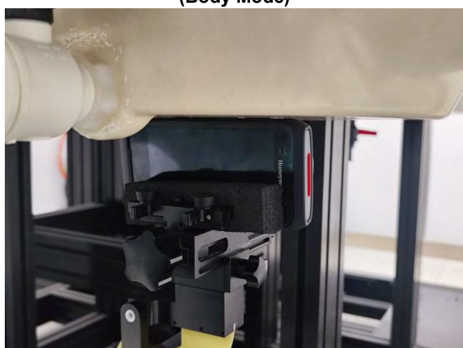
Left Side of EUT with 0 cm Gap (Body Mode)
