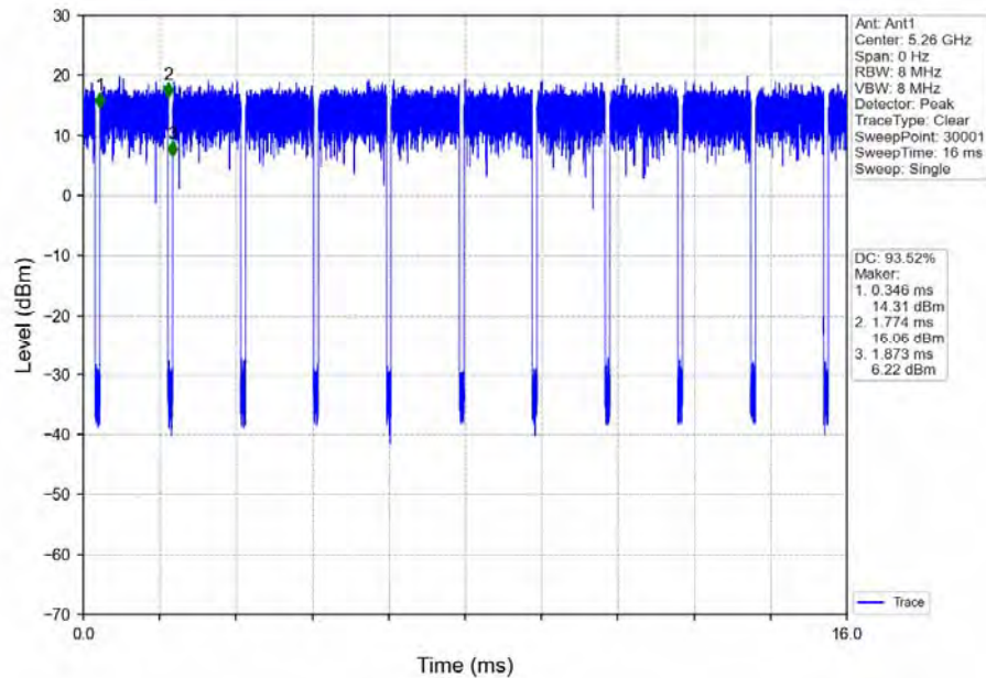
802.11a_LCH_5260MHz_Ant1_NTNV
