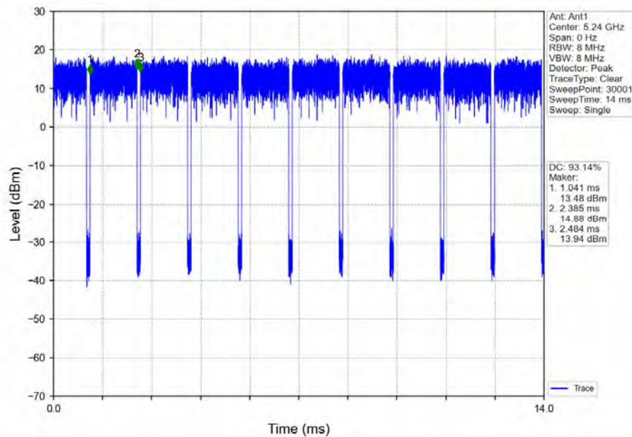
802.11ac(VHT20) HCH_5240MHz_Ant1_NTNV
