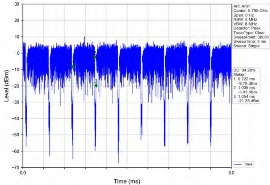
802.11ax(HEW40)_HCH_5795MHz_Ant1_NTNV_MIMO
