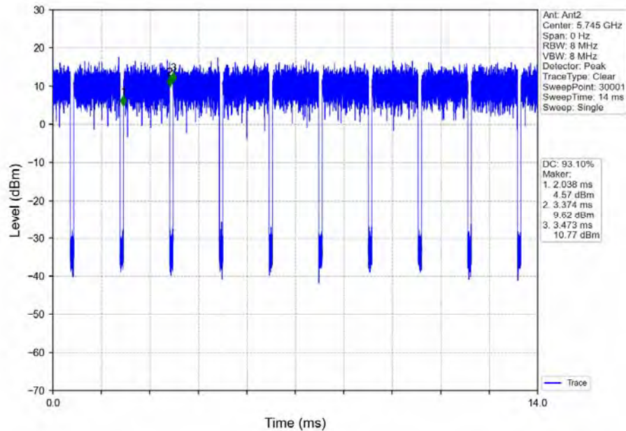
802.11n(HT20)_LCH_5745MHz_Ant2_NTNV
