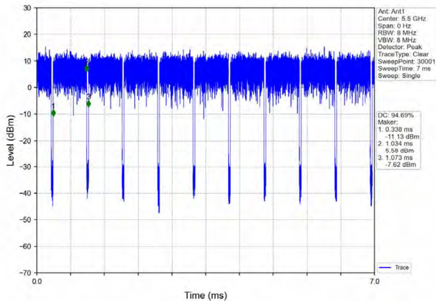
802.11ac(VHT20)_LCH_5500MHz_Ant1_NTNV_MIMO
