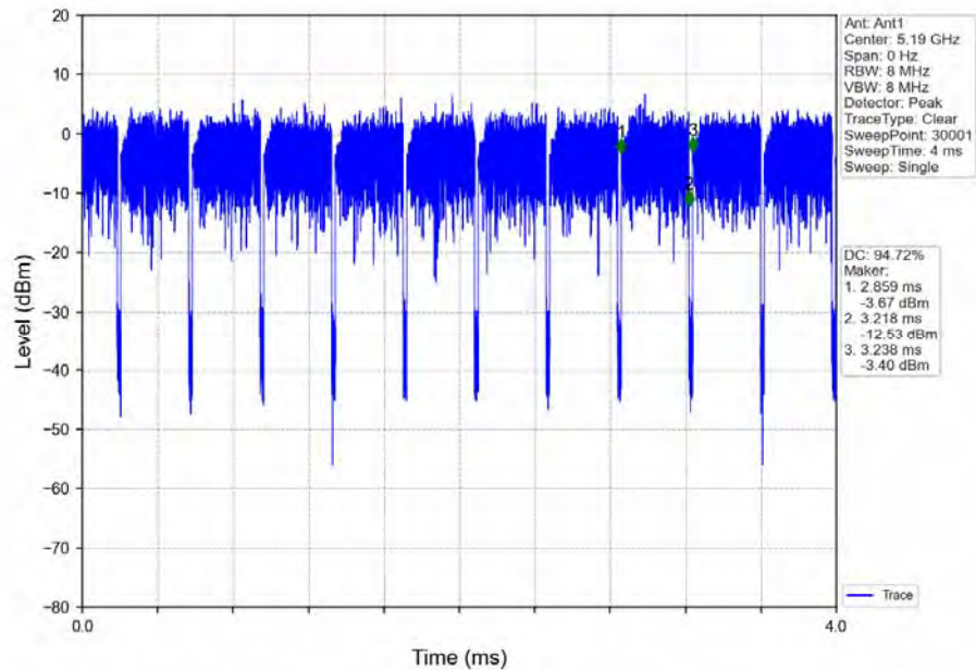
802.11ac(VHT40)_LCH_5190MHz_Ant1_NTNV_MIMO
