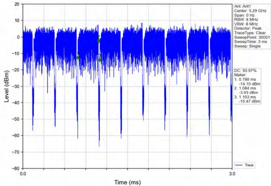
802.11ax(HEW80)_MCH_5290MHz_Ant1_NTNV
