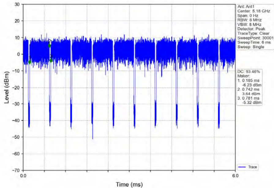
802.11ax(HEW20)_LCH_5180MHz_Ant1_NTNV_MIMO
