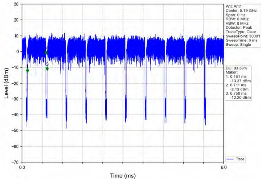
802.11ax(HEW40)_LCH_5190MHz_Ant1_NTNV
