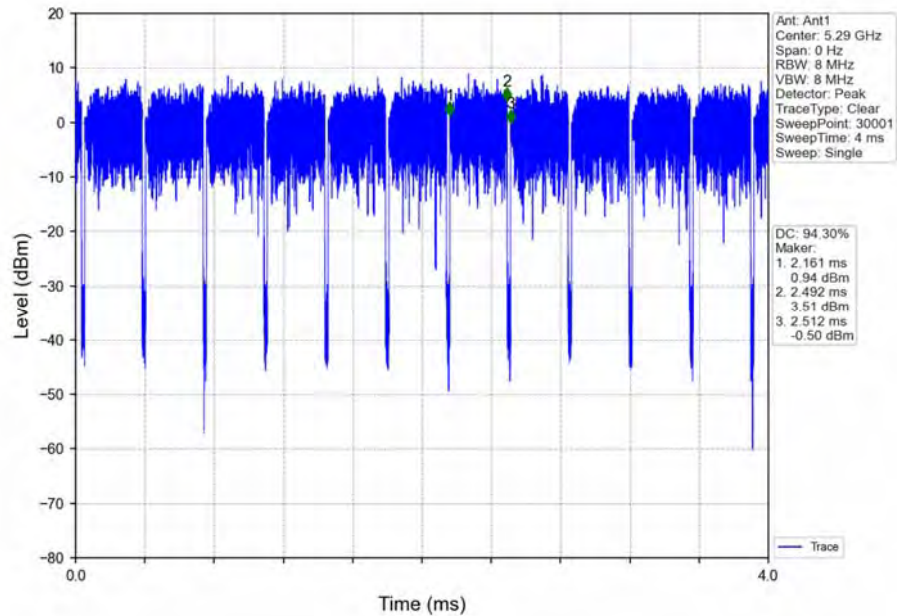
802.11ac(VHT80)_MCH_5290MHz_Ant1_NTNV
