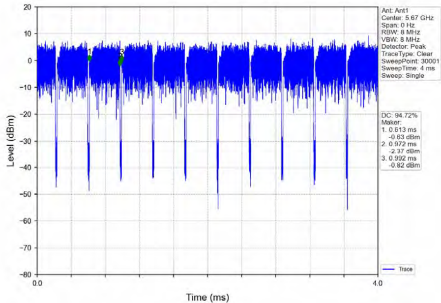
802.11ac(VHT40)_HCH_5670MHz_Ant1_NTNV_MIMO
