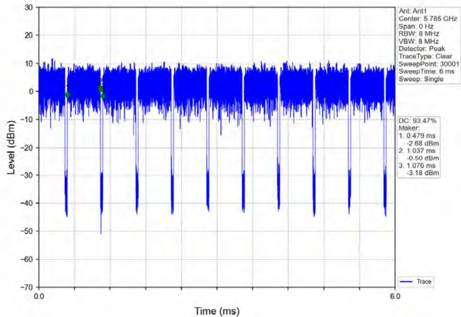
802.11ax(HEW20)_MCH_5785MHz_Ant1_NTNV_MIMO
