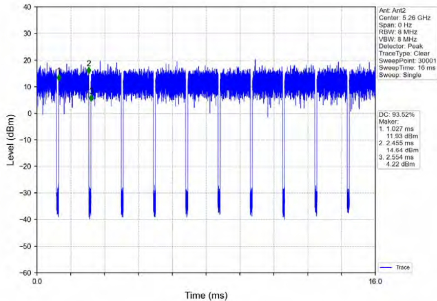
802.11a_LCH_5260MHz_Ant2_NTNV
