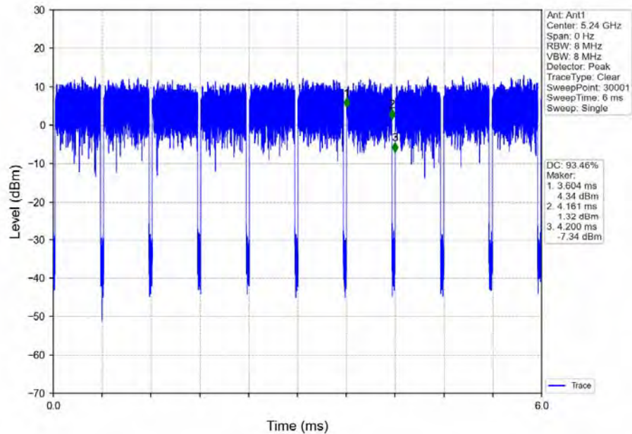
802.11ax(HEW20)_HCH_5240MHz_Ant1_NTNV_MIMO
