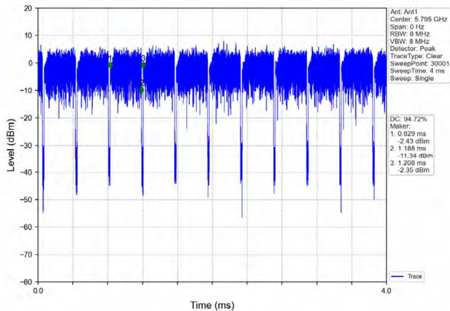
802.11ac(VHT40)_HCH_5795MHz_Ant1_NTNV_MIMO
