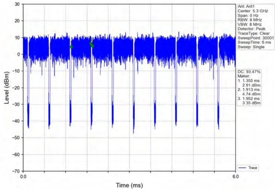
802.11ax(HEW20)_MCH_5300MHz_Ant1_NTNV_MIMO
