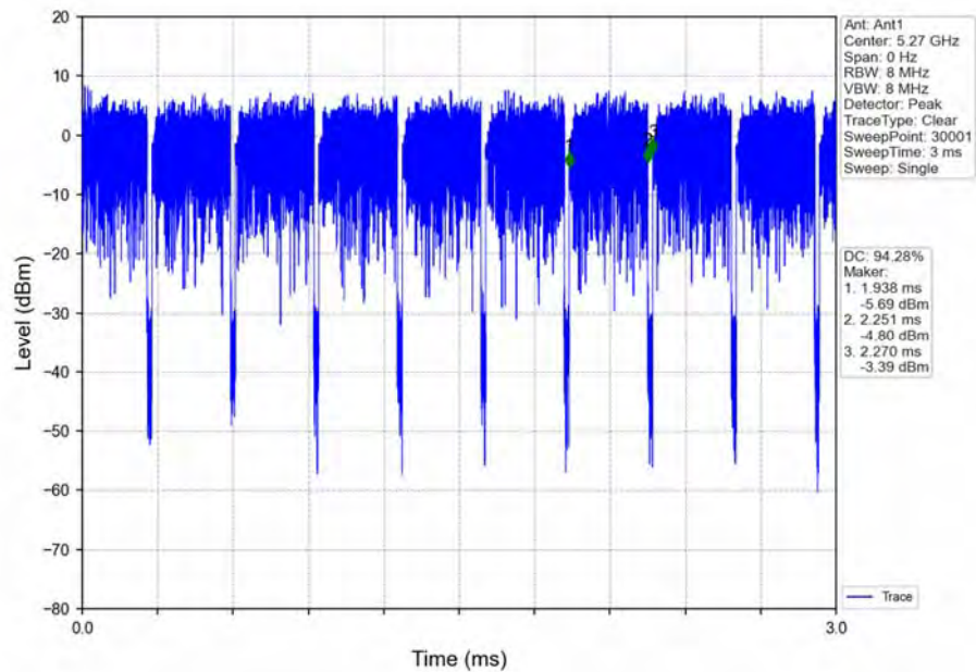
802.11ax(HEW40) LCH_5270MHz_Ant1_NTNV_MIMO
