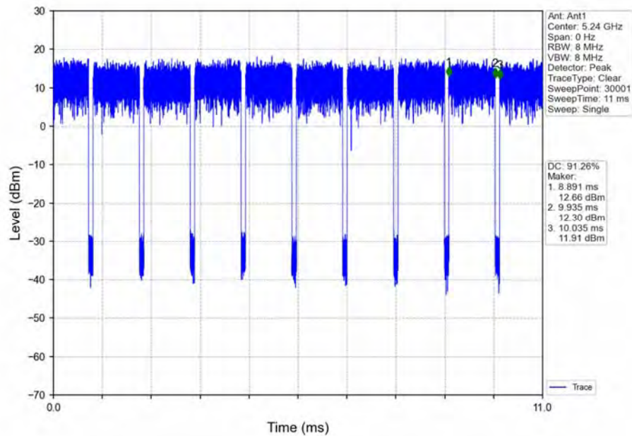
802.11ax(HEW20)_HCH_5240MHz_Ant1_NTNV
