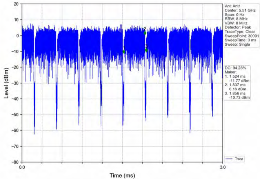
802.11ax(HEW40)_LCH_5510MHz_Ant1_NTNV_MIMO
