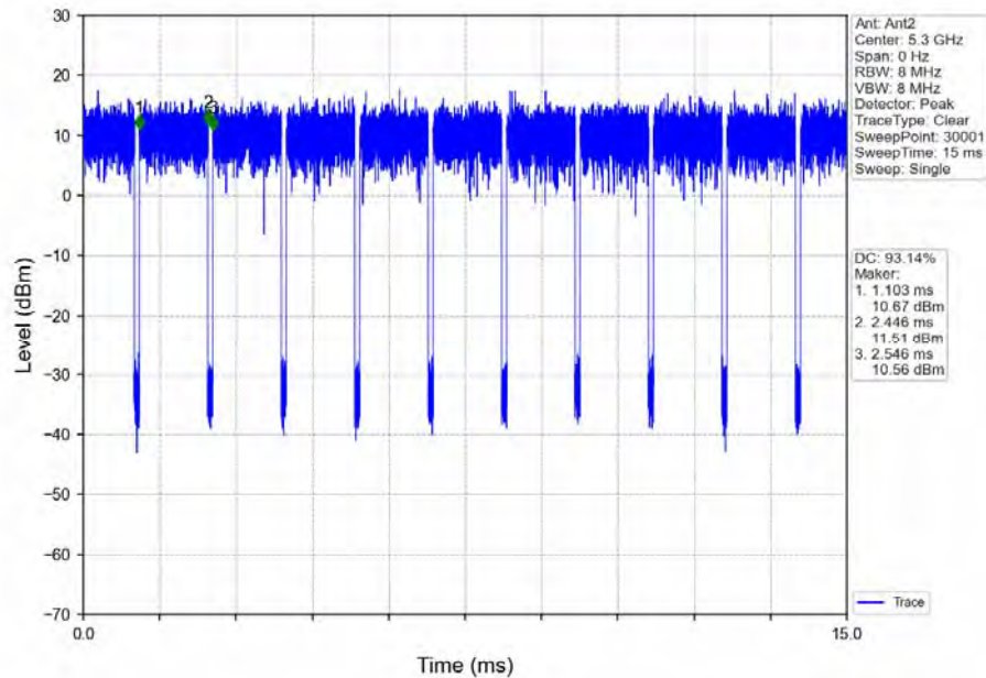
802.11ac(VHT20)_MCH_5300MHz_Ant2_NTNV
