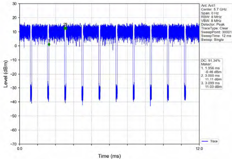
802.11ax(HEW20)_HCH_5700MHz_Ant1_NTNV
