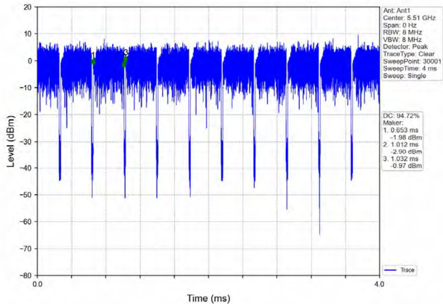
802.11ac(VHT40)_LCH_5510MHz_Ant1_NTNV_MIMO
