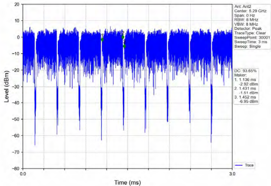
802.11ax(HEW80)_MCH_5290MHz_Ant2_NTNV
