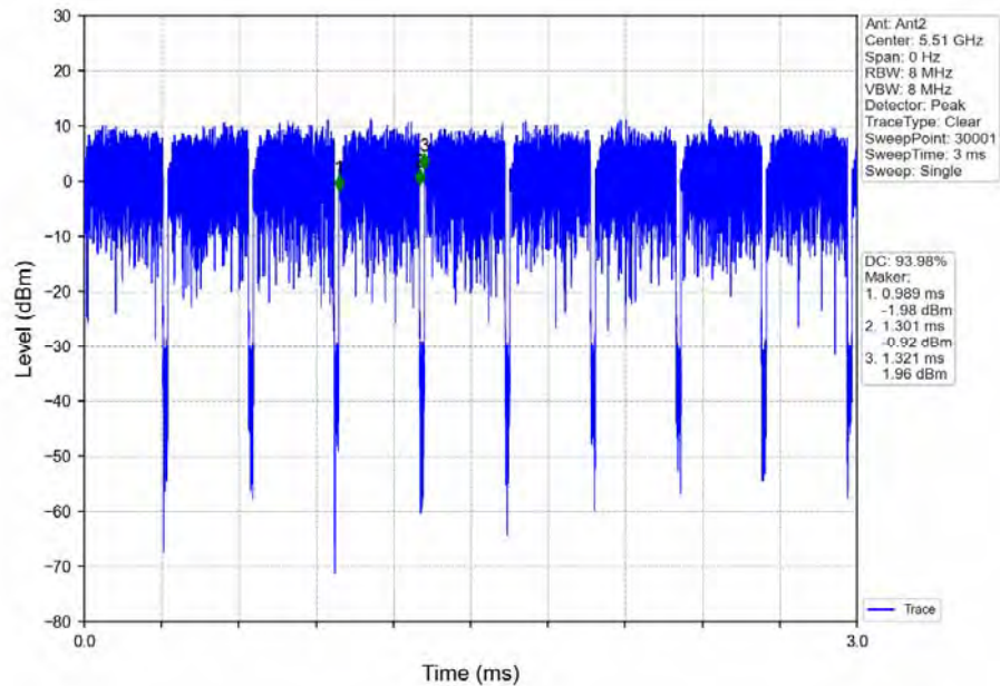
802.11ax(HEW40)_LCH_5510MHz_Ant2_NTNV_MIMO
