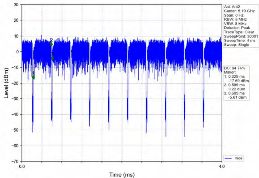
802.11ac(VHT40)_LCH_5190MHz_Ant2_NTNV_MIMO
