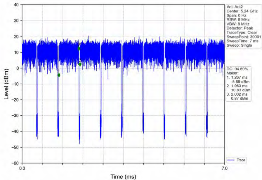
802.11ac(VHT20)_HCH_5240MHz_Ant2_NTNV_MIMO
