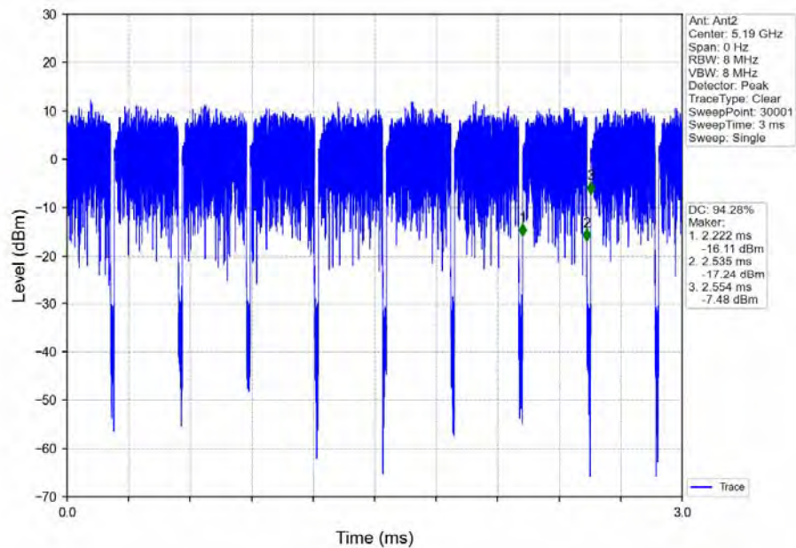
802.11ax(HEW40)_LCH_5190MHz_Ant2_NTNV_MIMO
