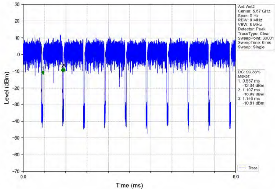
802.11ax(HEW40)_HCH_5670MHz_Ant2_NTNV
