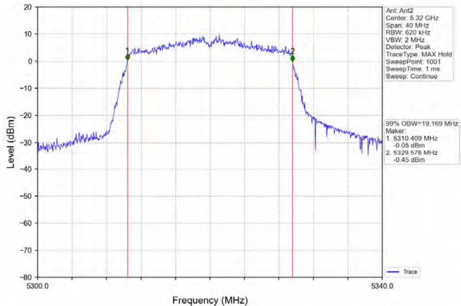
802.11ax(HEW20)_HCH_5320MHz_Ant2_NTNV
