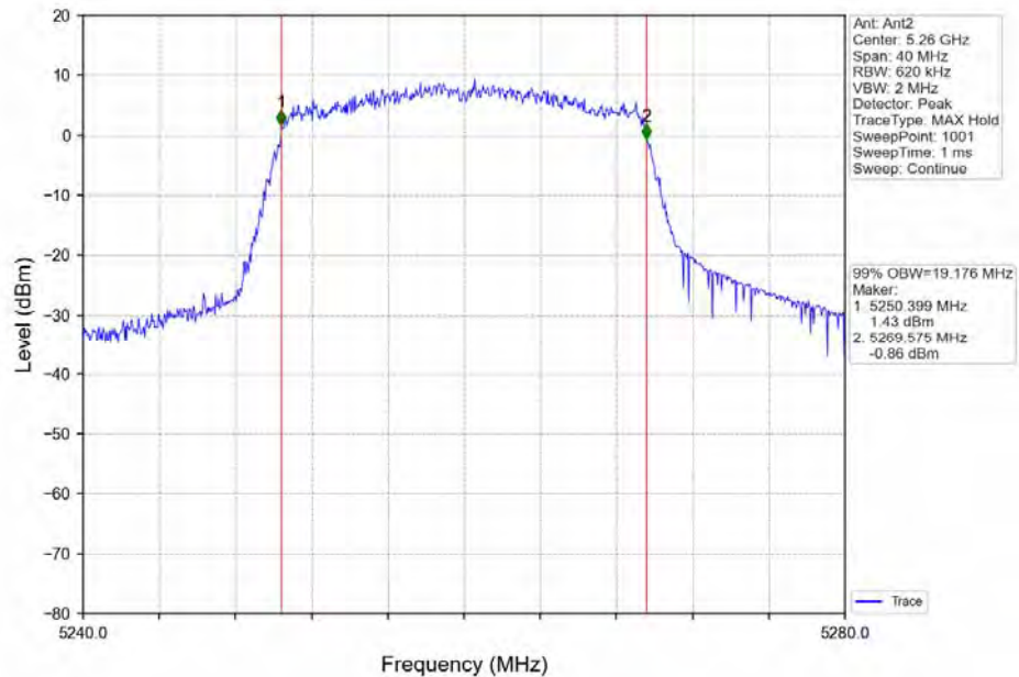
802.11ax(HEW20)_LCH_5260MHz_Ant2_NTNV
