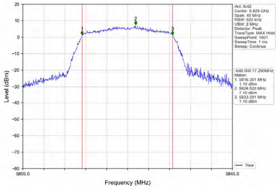
802.11ac(VHT20) HCH_5825MHz_Ant2_NTNV
