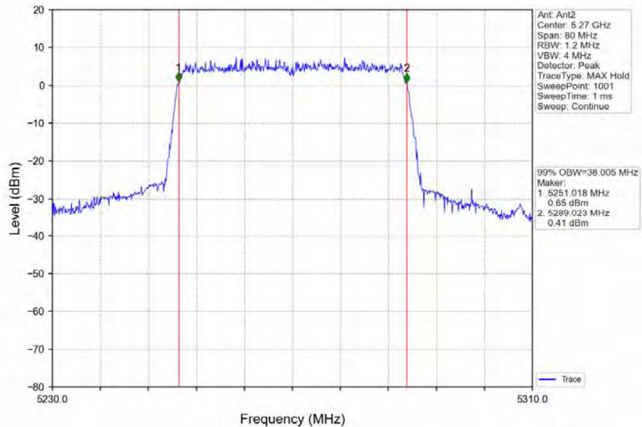
802.11ax(HEW40)_LCH_5270MHz_Ant2_NTNV
