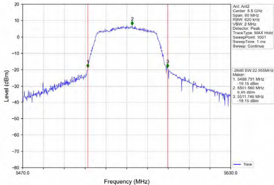
802.11ac(VHT20)_LCH_5500MHz_Ant2_NTNV
