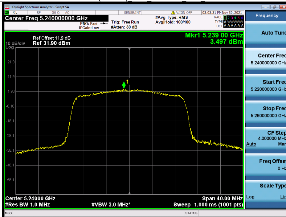
802.11ax(HEW20) HCH 5240MHz Ant2 NTN
