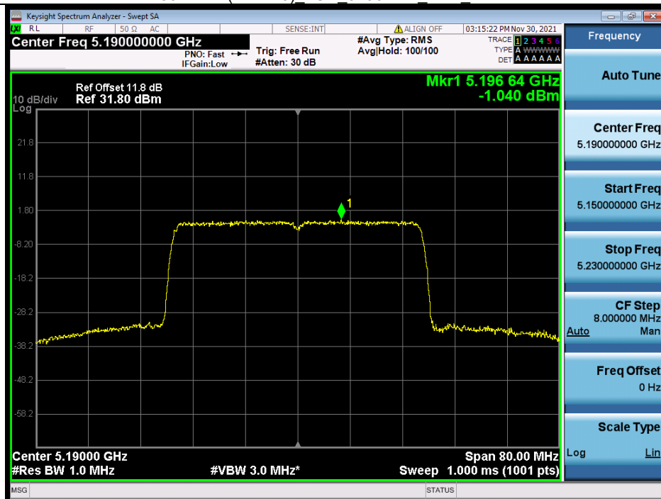
802.11ax(HEW40) LCH 5190MHz Ant2 NTN
