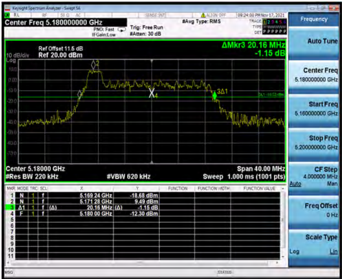
11AX20SISO_Ant1_5180_26Tone_RU4
