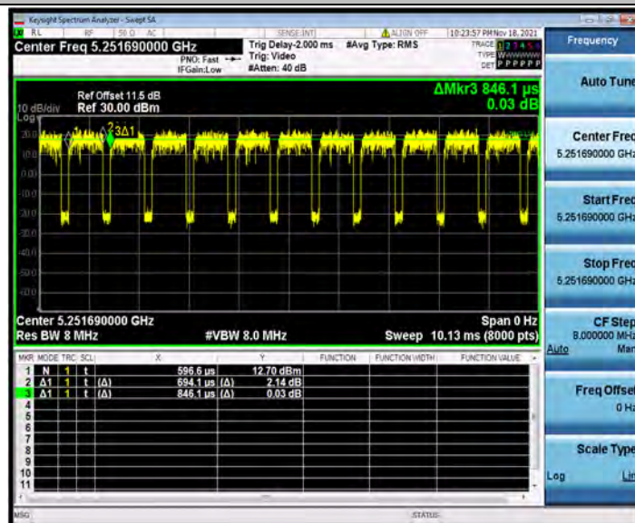
11AX20SISO_Ant2_5260_26Tone_RU4
