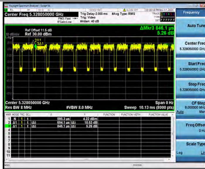
11AX20SISO_Ant1_5320_242Tone_RU61
