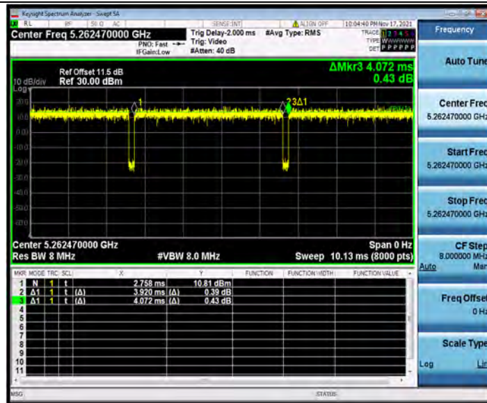
11AX20SISO_Ant2_5260_26Tone_RU0
