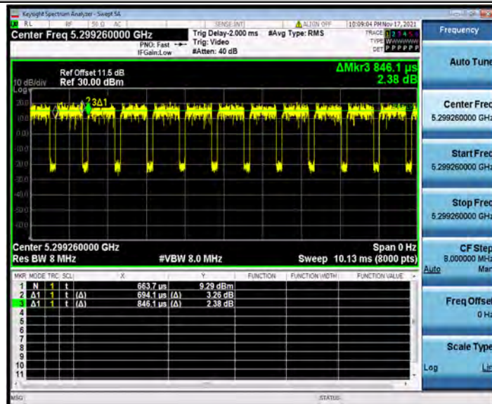
11AX20SISO_Ant1_5300_26Tone_RU8
