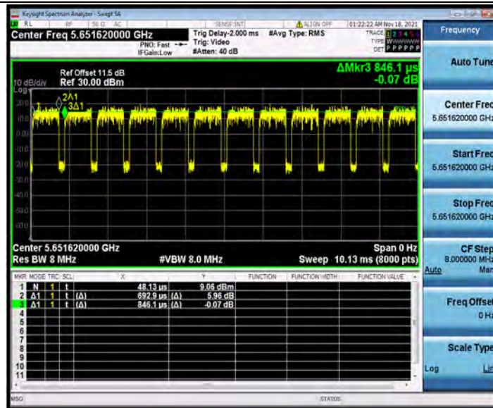
11AX40SISO_Ant1_5670_26Tone_RU8
