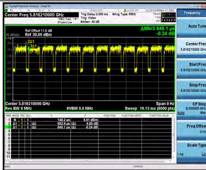
11AX20SISO_Ant1_5825_26Tone_RU4
