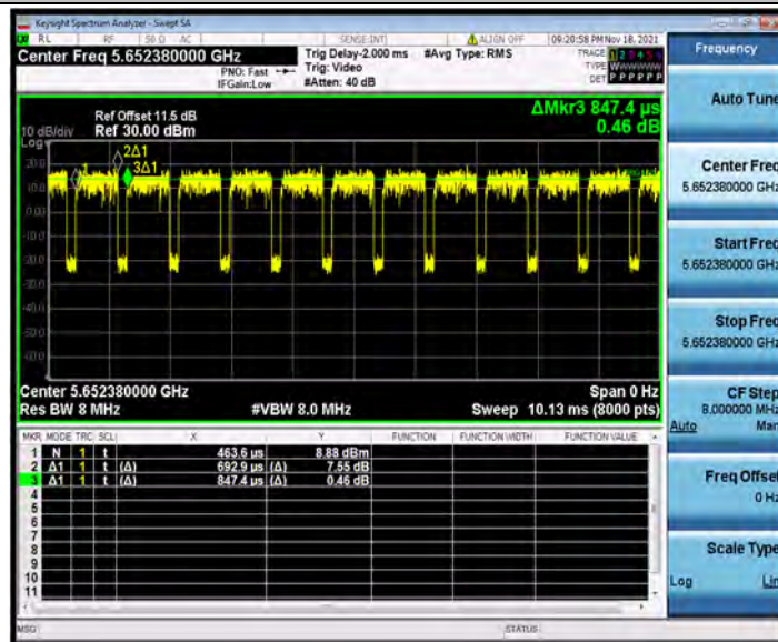
11AX80SISO_Ant1_5690_26Tone_RU18
