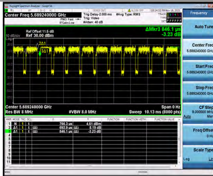
11AX80SISO_Ant1_5690_26Tone_RU36
