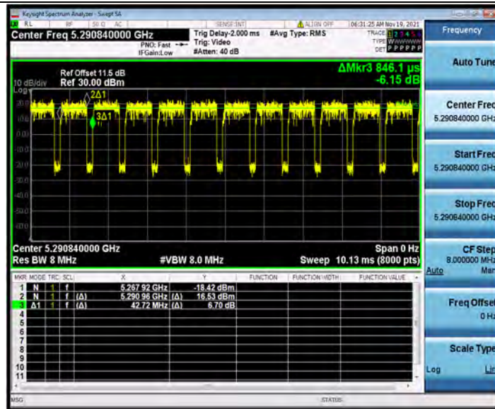
11AX80SISO_Ant2_5290_26Tone_RU36
