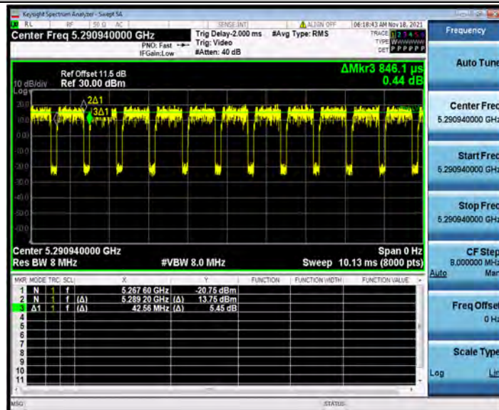
11AX80ISO_Ant1_5290_26Tone_RU36
