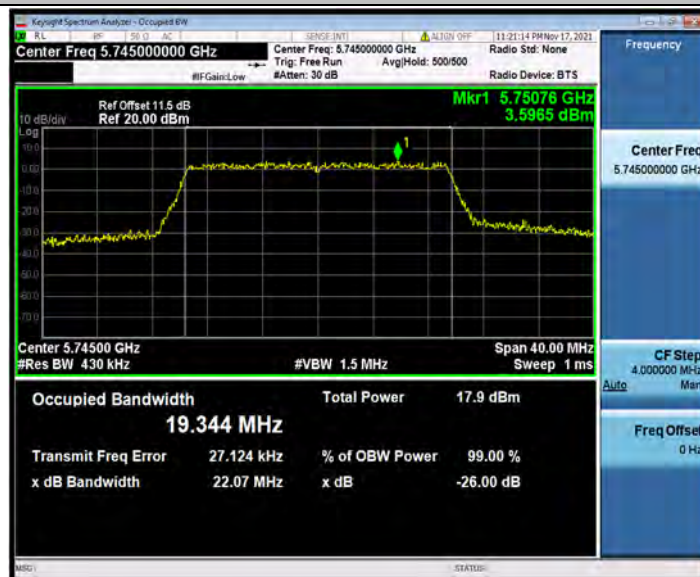
11AX20SISO_Ant2_5745_26Tone_RU0
