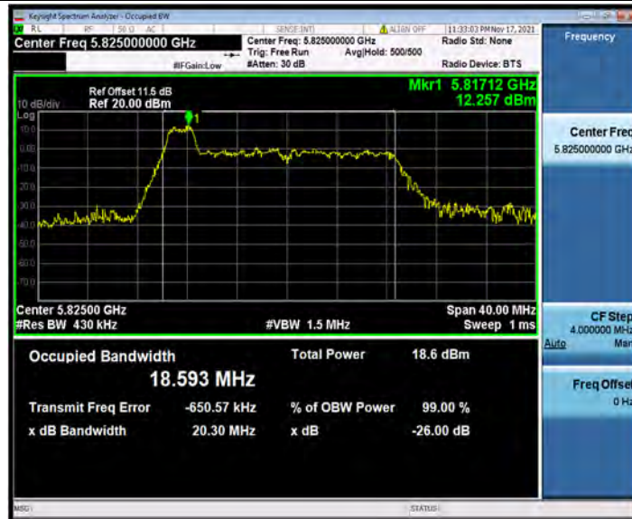
11AX20SISO_Ant1_5825_26Tone_RU4
