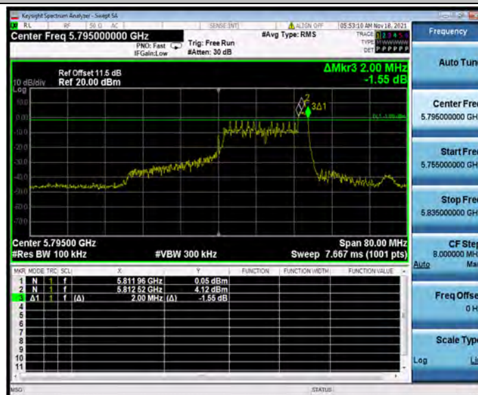
11AX40SISO_Ant1_5795_26Tone_RU17
