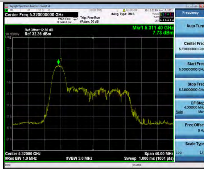
11AX20SISO_Ant1_5320_26Tone_RU4
