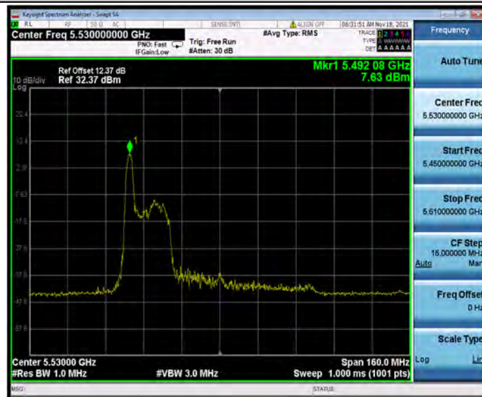
11AX80SISO_Ant1_5530_26Tone_RU18
