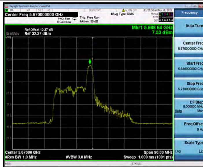
11AX40SISO_Ant1_5670_26Tone_RU17
