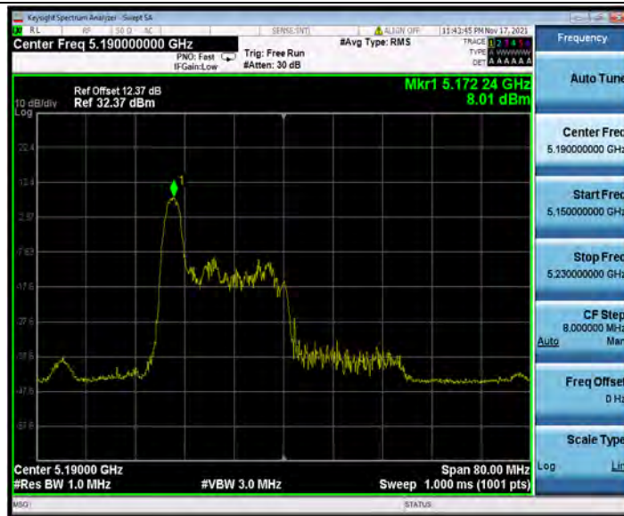
11AX40SISO_Ant1_5190_26Tone_RU8
