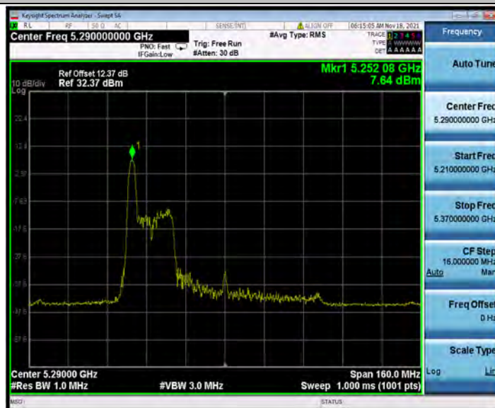
11AX80SISO_Ant1_5290_26Tone_RU18
