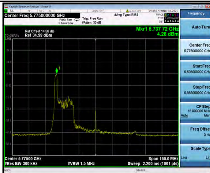
11AX80SISO_Ant1_5775_26Tone_RU18
