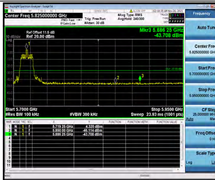
11AX20MIMO_Ant1_High_5720_26Tone_RU8
