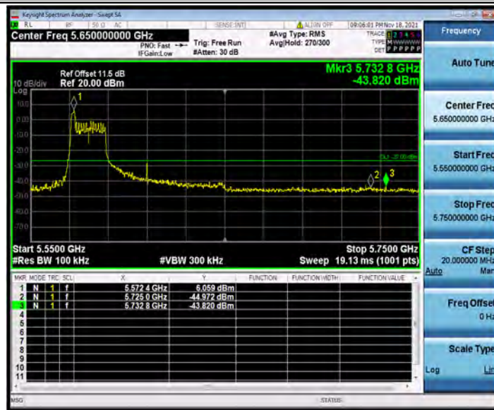
11AX80SISO_Ant1_High_5610_26Tone_RU18
