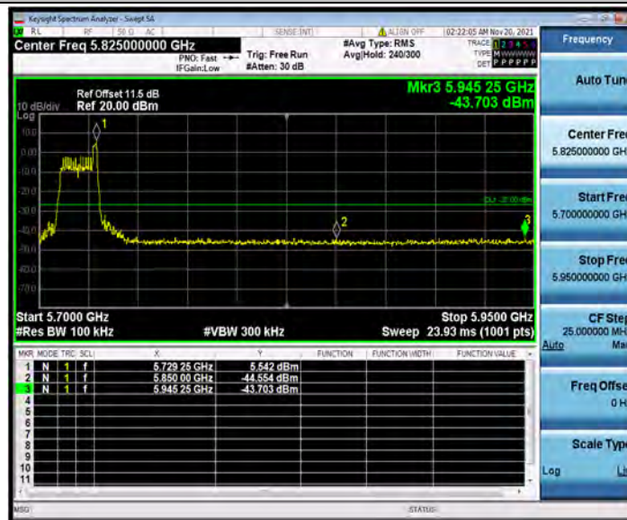
11AX20MIMO_Ant1_High_5720_242Tone_RU61
