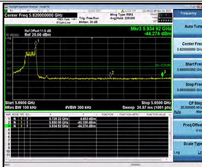
11AX40SISO_Ant2_High_5710_26Tone_RU17
