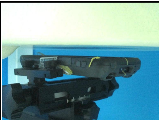
Body worn - Front Face of EUT at 10 mm
