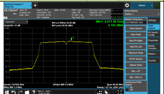
Channel 134 (5670MHz)
