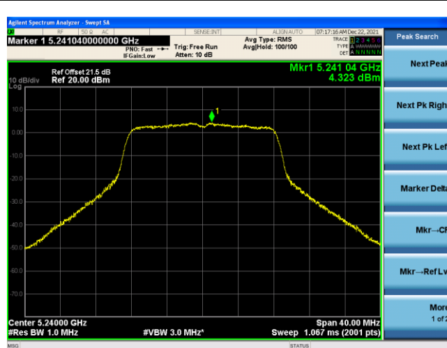
Channel 48 (5240MHz)
