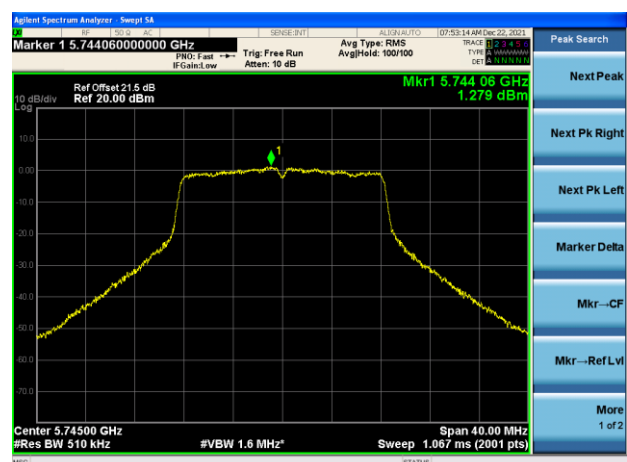
Channel 149 (5745MHz)
