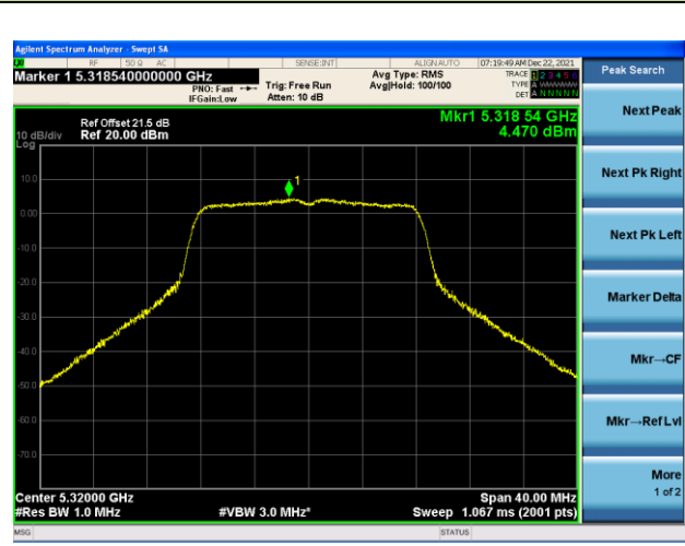
Channel 64 (5320MHz)
