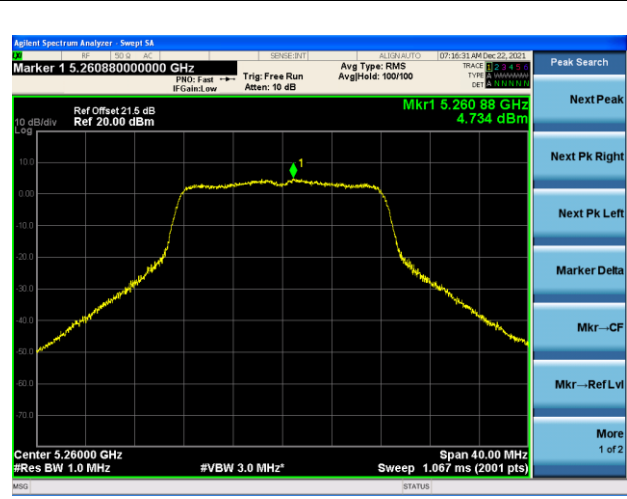
Channel 52 (5260MHz)
