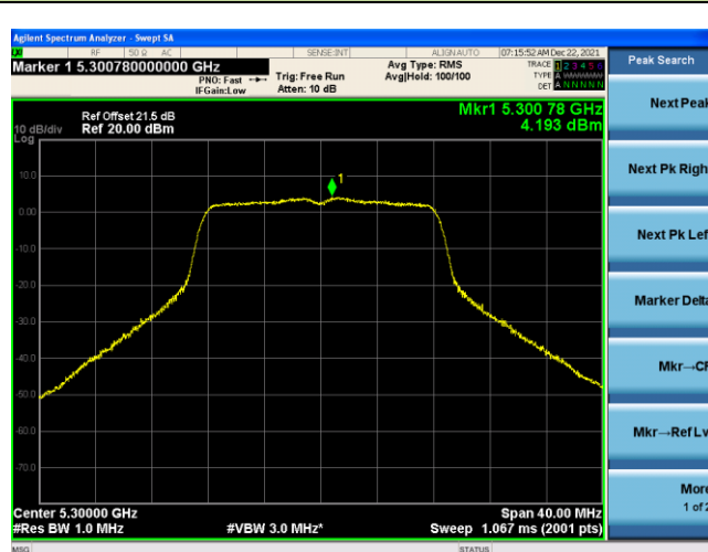
Channel 60 (5300MHz)
