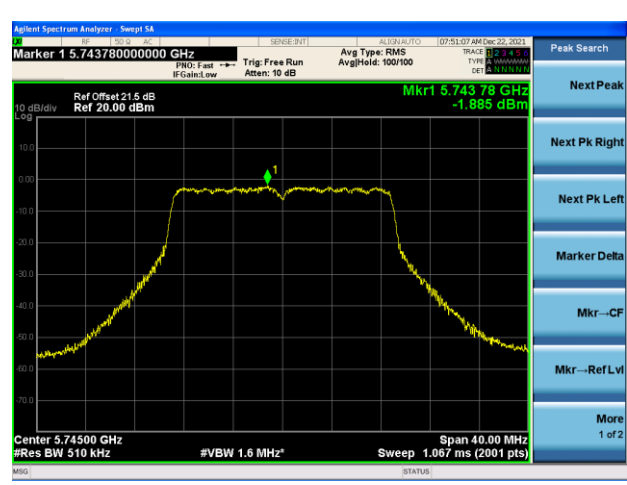
Channel 149 (5745MHz)
