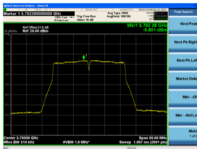
Channel 159 (5795MHz)
