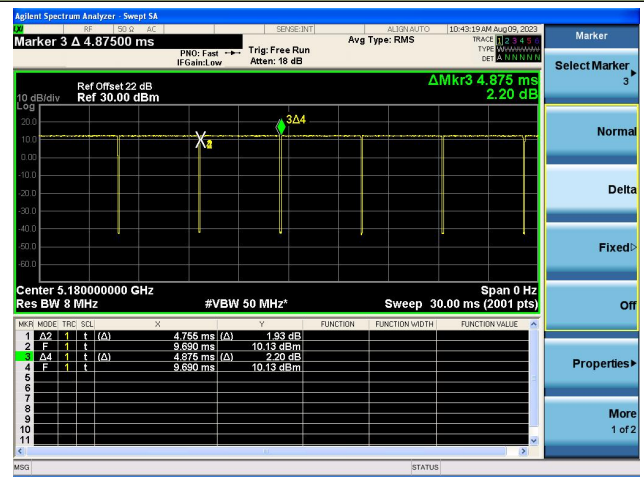
802.11ac-VHT20 (T = 4.755ms)
