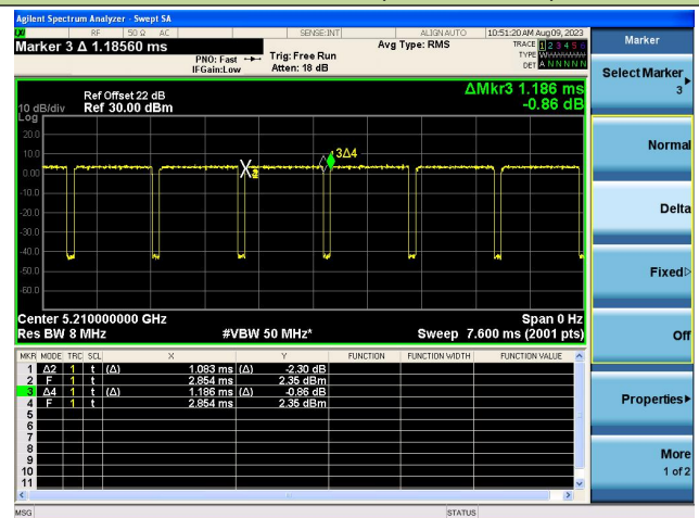
802.11ac-VHT80 (T = 1.083ms)
