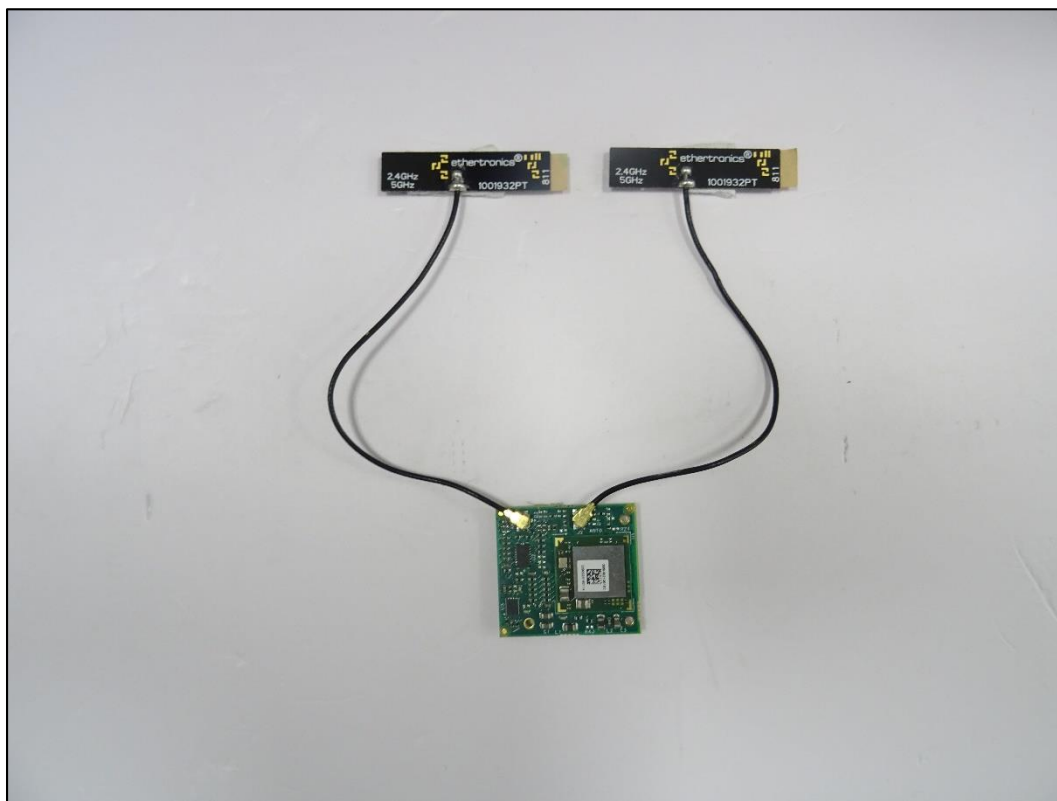
Module with Antenna (Part No: 1001932PT)
