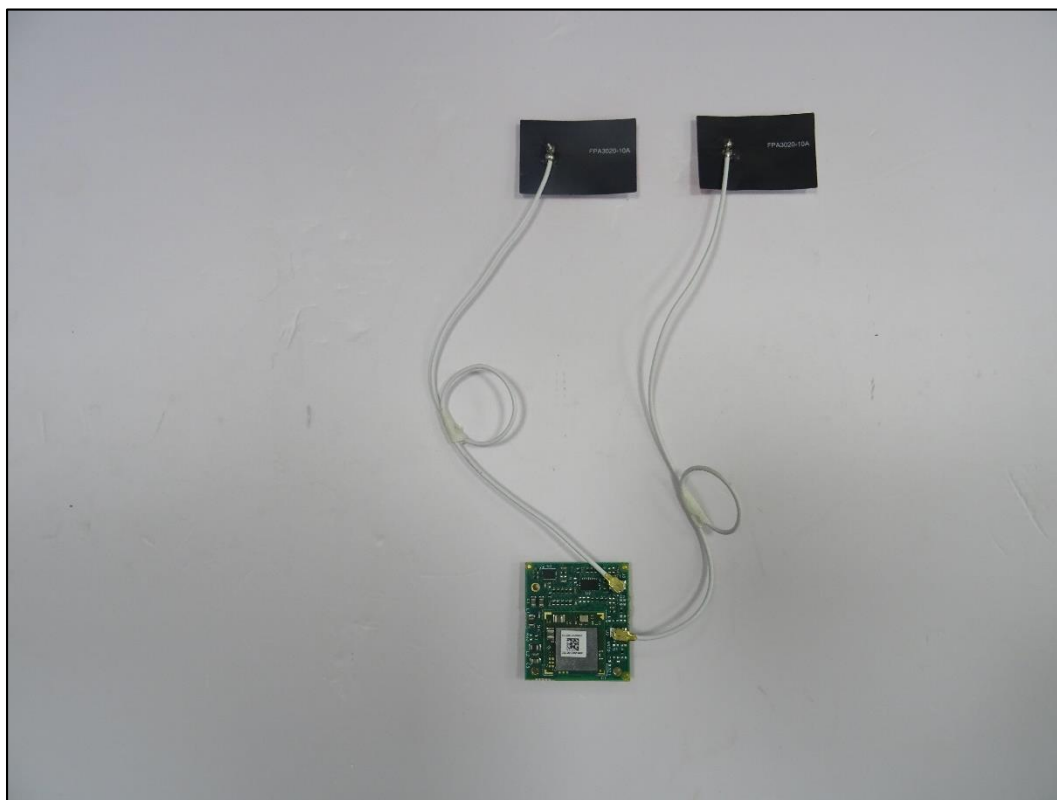
Module with Antenna (Part No: FPA3020-10)
