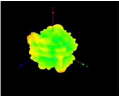
WiFi chain 1_6550MHz
