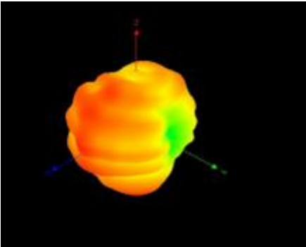
WiFi chain 0_5550MHz
