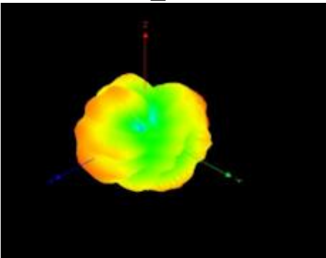
WiFi chain 1_5550MHz
