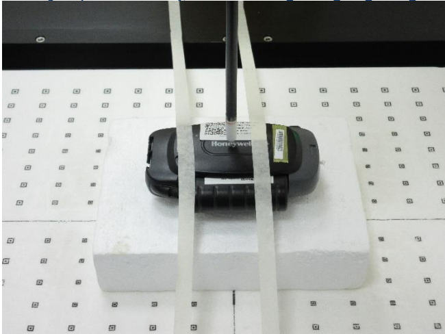
Testing Setup for Power Density, Rear Face at 2 mm A720XP thick Holster w/o
