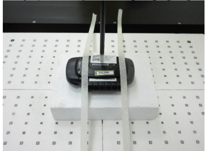
Testing Setup for Power Density, Rear Face at 2 mm A710XP thick Holster w/o
