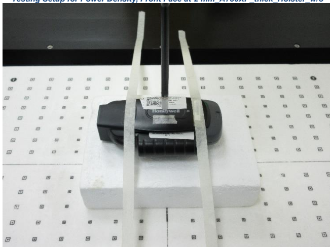
Testing Setup for Power Density, Front Face at 2 mm A730XP thick Holster w/o
