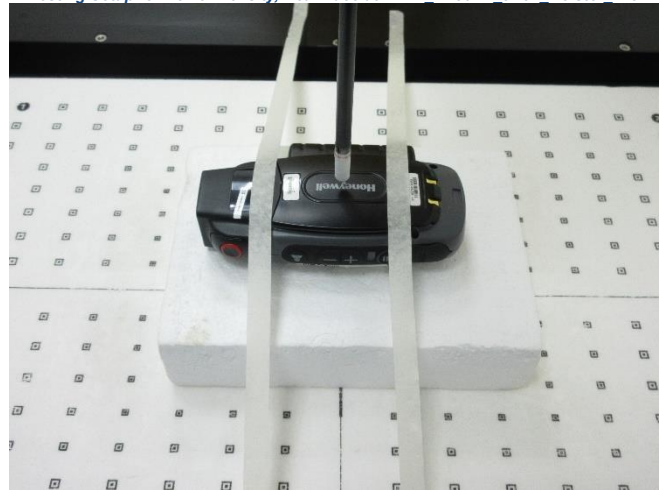
Testing Setup for Power Density, Rear Face at 2 mm A730XP thick Holster w/o
