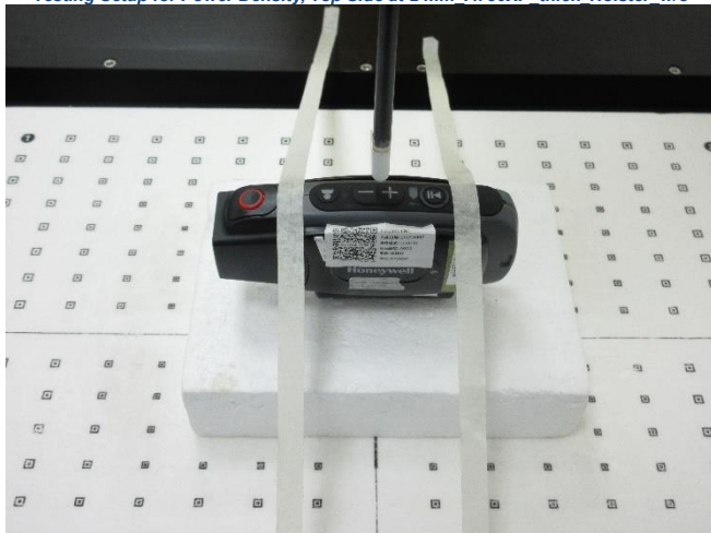
Testing Setup for Power Density, Top Side at 2 mm A730XP thick Holster w/o
