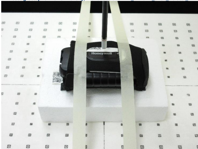
Testing Setup for Power Density, Front Face at 2 mm A720XP thick Holster w
