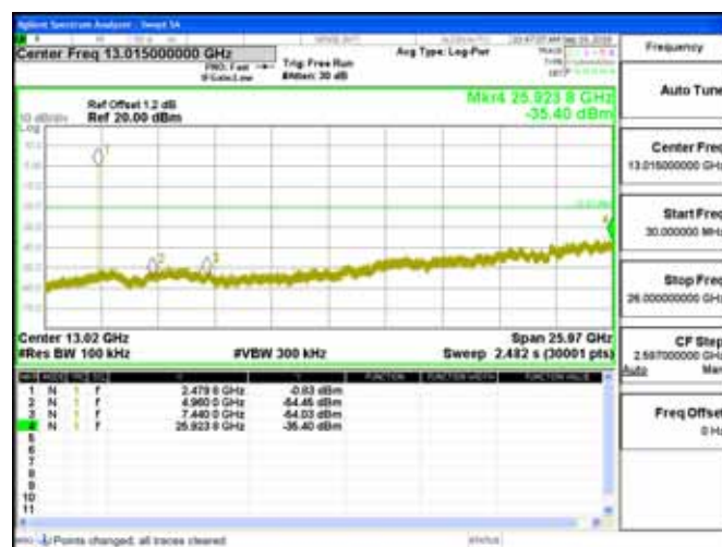
Spurious Emission_π/4DQPSK_2M_2480MHz
