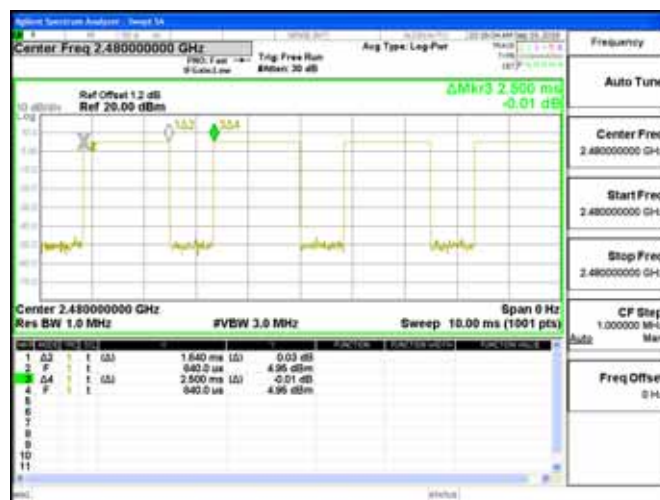
Dwell Time_GFSK_1M_DH3_2480MHz
