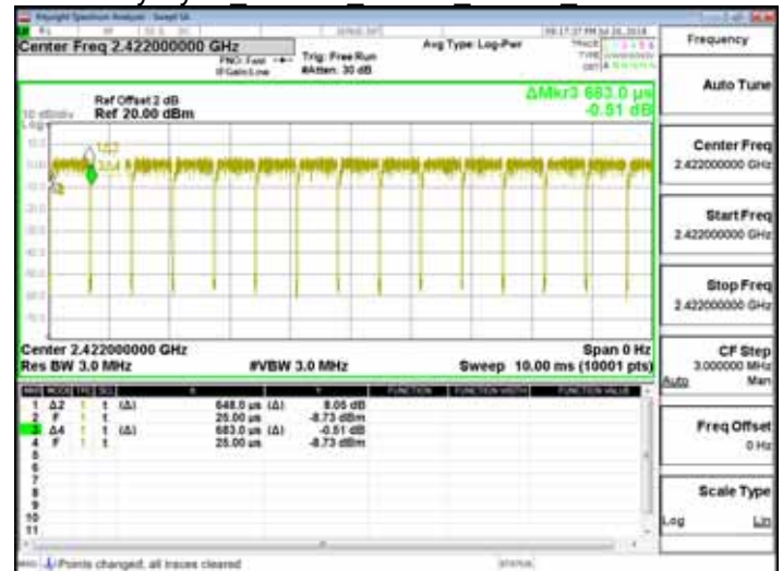
Duty Cycle 802.11n 40MHz Chain0 2422MHz
