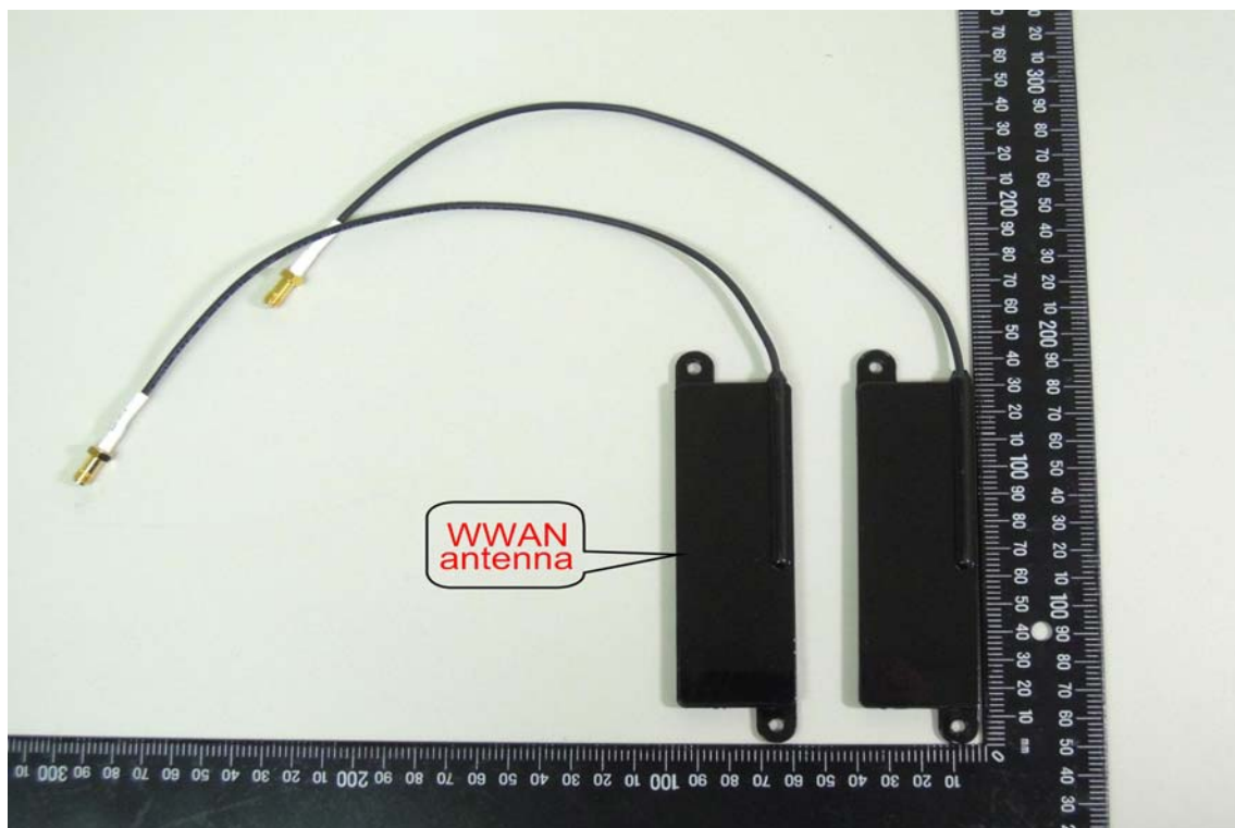
WWAN External Antenna-2 (Model No.: TRA6927M3)
