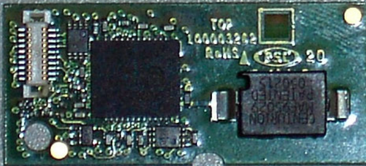
BT Module : TOP View of PCB
